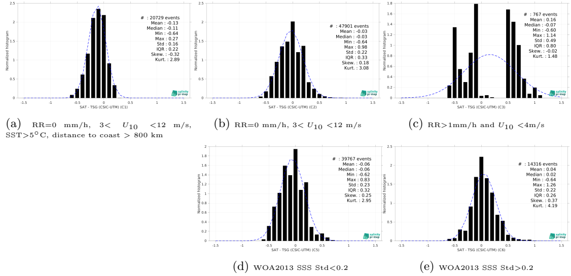
Figure 15: Normalized histogram of \Delta SSS (SMOS SSS L4 v2 - Daily (BEC) - TSG (CSIC-UTM)) for 5 different subdatasets corresponding to: RR=0 mm/h, 3 < U_{10} < 12 m/s, SST>5°C, distance to coast > 800 km (a), RR=0 mm/h, 3 < U_{10} < 12 m/s (b), RR>1mm/h and U_{10} < 4 m/s (c), WOA2013 SSS Std<0.2 (d), WOA2013 SSS Std>0.2 (e).
