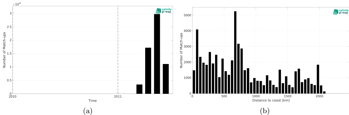
Figure 2: Number of match-ups between TSG (CSIC-UTM) and SMOS SSS L4 v2 - Daily (BEC) SSS as a function of time (a) and as function of the distance to coast (b) over the Pacific Ocean Pi-MEP region and for the full satellite product period.
