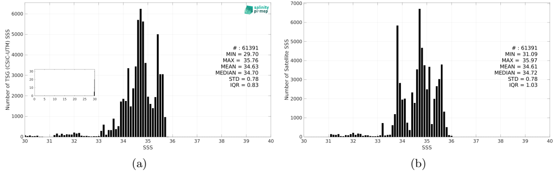
Figure 3: Histograms of SSS from TSG (CSIC-UTM) (a) and SMOS SSS L4 v2 - Daily (BEC) (b) considering all match-up pairs per bins of 0.1 over the Pacific Ocean Pi-MEP region and for the full satellite product period.
