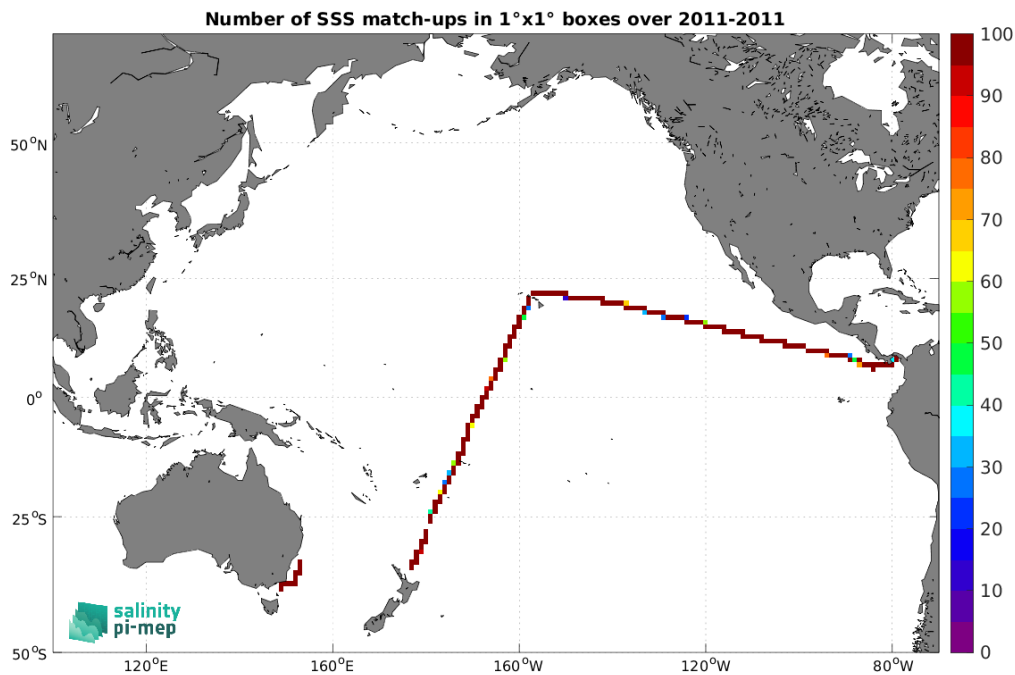
Figure 5: Number of SSS match-ups between TSG (CSIC-UTM) SSS and the SMOS SSS L4 v2 - Daily (BEC) SSS product for the Pacific Ocean Pi-MEP region over 1^\circ \times 1^\circ boxes and for the full satellite product period.
