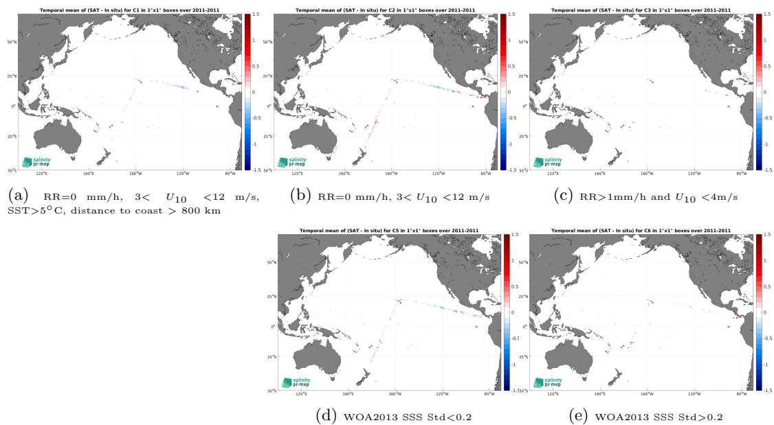
Figure 14: Temporal mean gridded over spatial boxes of size 1^\circ \times 1^\circ of \Delta\text{SSS} (SMOS SSS L4 v2 - Daily (BEC) - TSG (CSIC-UTM)) for 5 different subdatasets corresponding to:RR=0 mm/h, 3 < U_{10} < 12 m/s, SST > 5^\circ\text{C} , distance to coast > 800 km (a), RR=0 mm/h, 3 < U_{10} < 12 m/s (b), RR > 1 mm/h and U_{10} < 4 m/s (c), WOA2013 SSS Std < 0.2 (d), WOA2013 SSS Std > 0.2 (e).
