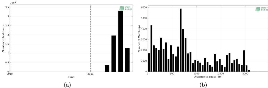
Figure 1: Number of match-ups between TSG (CSIC-UTM) and SMOS SSS L4 v2 - Daily (BEC) SSS as a function of time (a) and as function of the distance to coast (b) over the Pacific Ocean Pi-MEP region and for the full satellite product period.
