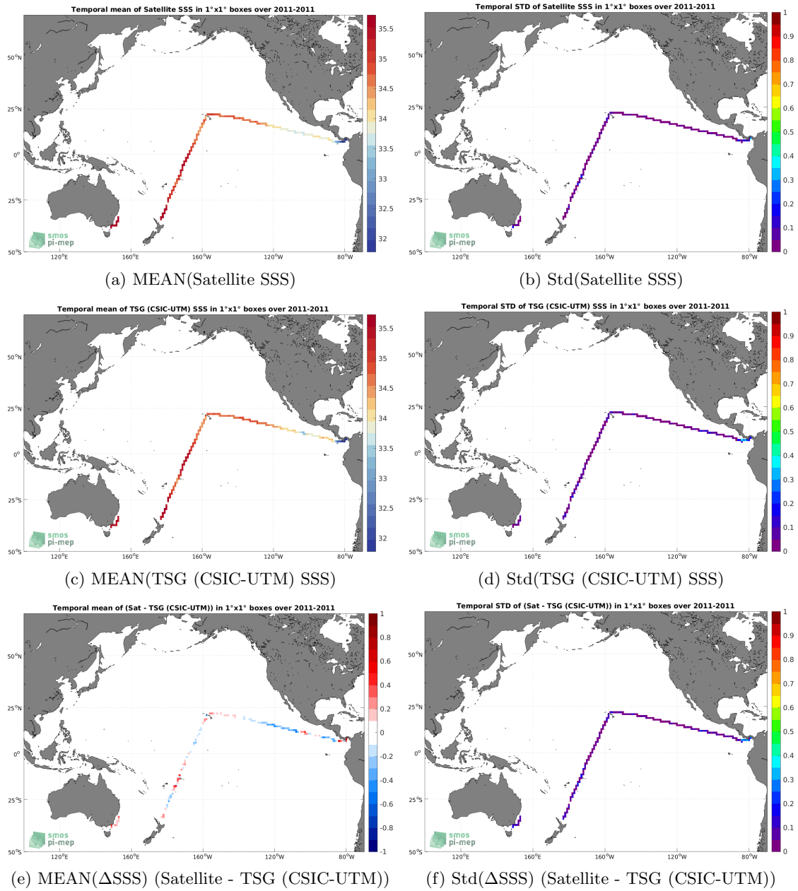
Figure 6: Temporal mean (left) and Std (right) of SSS from SMOS SSS L4 v2 - Daily (BEC) (top), TSG (CSIC-UTM) (middle), and of \Delta SSS (Satellite - TSG (CSIC-UTM)). Only match-up pairs are used to generate these maps.
