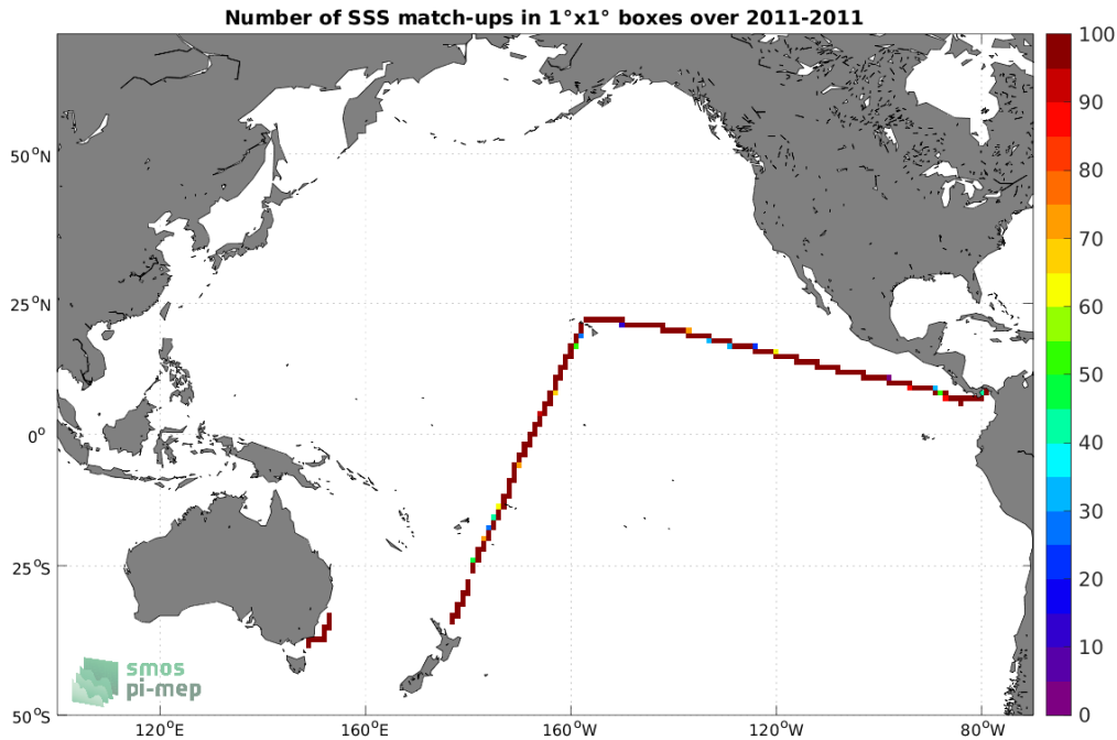
Figure 4: Number of SSS match-ups between TSG (CSIC-UTM) SSS and the SMOS SSS L4 v2 - Daily (BEC) SSS product for the Pacific Ocean Pi-MEP region over 1^\circ \times 1^\circ boxes and for the full satellite product period.
