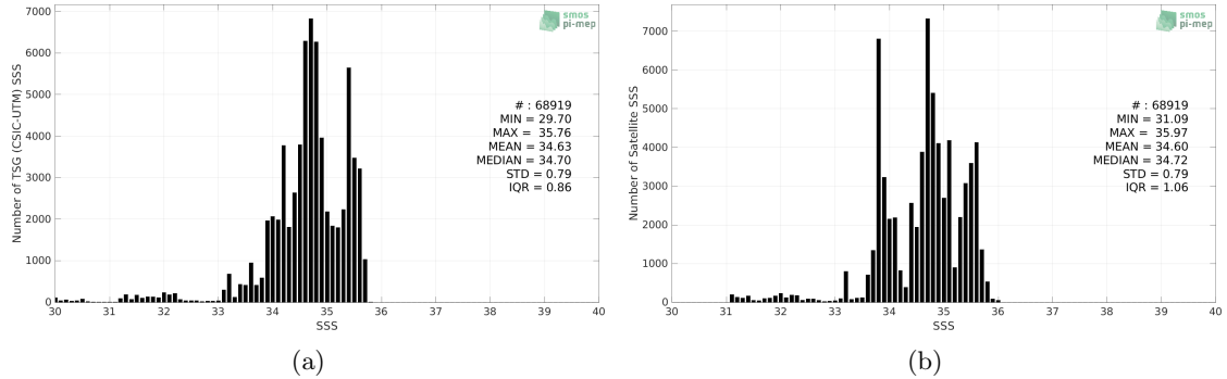
Figure 2: Histograms of SSS from TSG (CSIC-UTM) (a) and SMOS SSS L4 v2 - Daily (BEC) (b) considering all match-up pairs per bins of 0.1 over the Pacific Ocean Pi-MEP region and for the full satellite product period.
