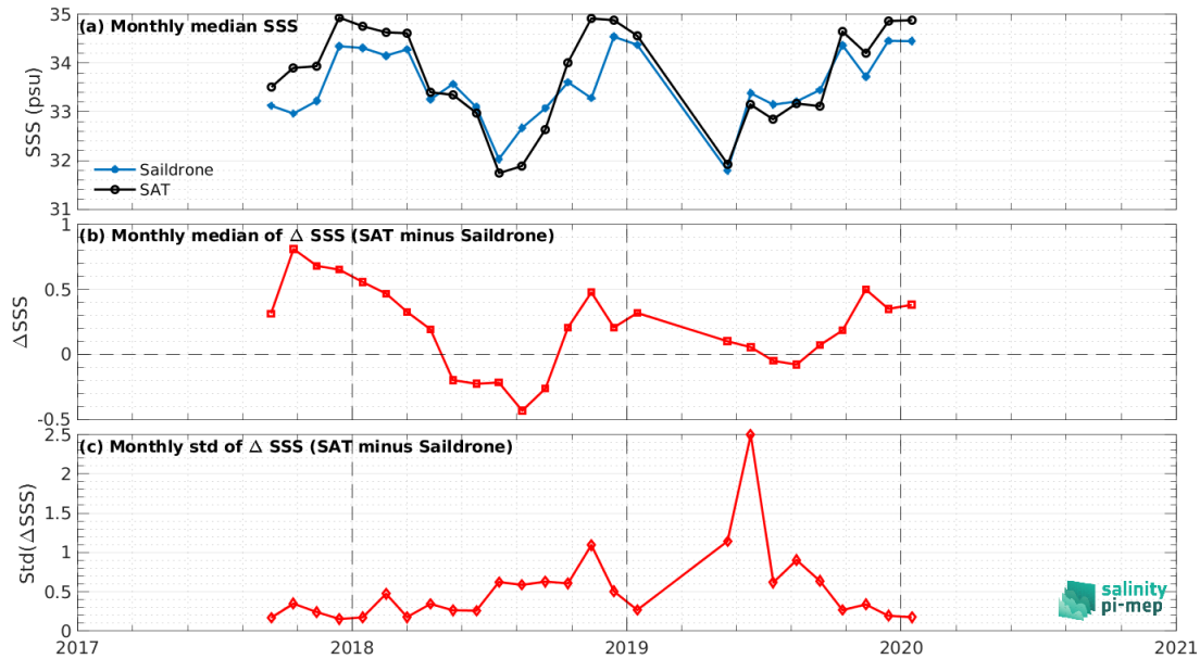
Figure 8: Time series of the monthly median SSS (top), median of \Delta SSS (Satellite - Sairdronne) and Std of \Delta SSS (Satellite - Sairdronne) over the Pacific Ocean Pi-MEP region considering all match-ups collected by the Pi-MEP.
