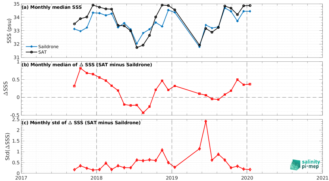
Figure 7: Time series of the monthly median SSS (top), median of \Delta SSS (Satellite - Sairdrone) and Std of \Delta SSS (Satellite - Sairdrone) over the Pacific Ocean Pi-MEP region considering all match-ups collected by the Pi-MEP.
