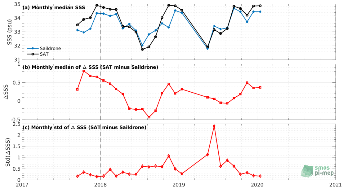
Figure 7: Time series of the monthly median SSS (top), median of \Delta\text{SSS} (Satellite - Sairdrone) and Std of \Delta\text{SSS} (Satellite - Sairdrone) over the Pacific Ocean Pi-MEP region considering all match-ups collected by the Pi-MEP.
