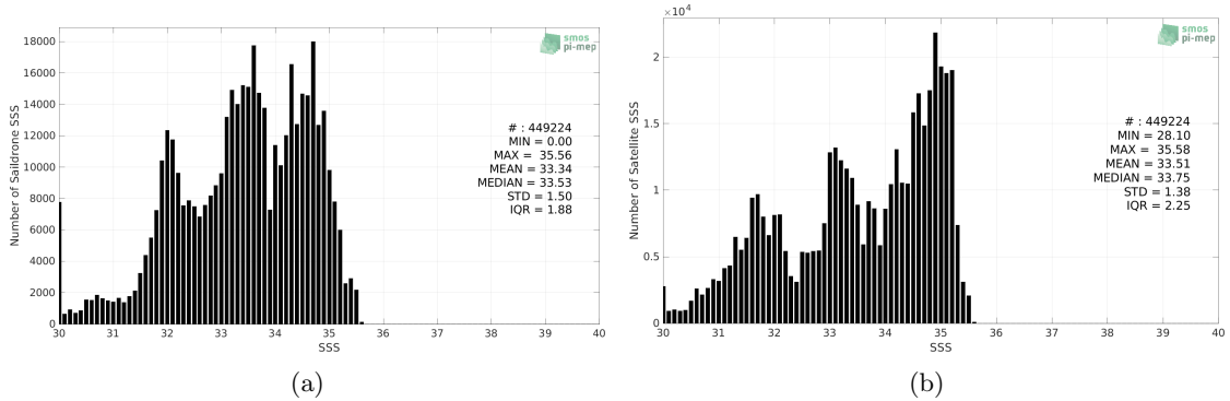
Figure 2: Histograms of SSS from Saildrone (a) and SMOS SSS L4 v2 - Daily (BEC) (b) considering all match-up pairs per bins of 0.1 over the Pacific Ocean Pi-MEP region and for the full satellite product period.
