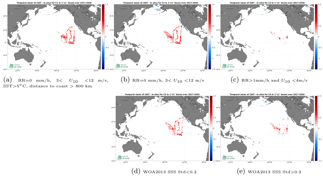
Figure 12: Temporal mean gridded over spatial boxes of size 1^\circ \times 1^\circ of \Delta SSS (SMOS SSS L4 v2 - Daily (BEC) - Sairdrone) for 5 different subdatasets corresponding to:RR=0 mm/h, 3 < U_{10} < 12 m/s, SST >5^\circ C, distance to coast > 800 km (a), RR=0 mm/h, 3 < U_{10} < 12 m/s (b), RR >1 mm/h and U_{10} < 4 m/s (c), WOA2013 SSS Std <0.2 (d), WOA2013 SSS Std >0.2 (e).
