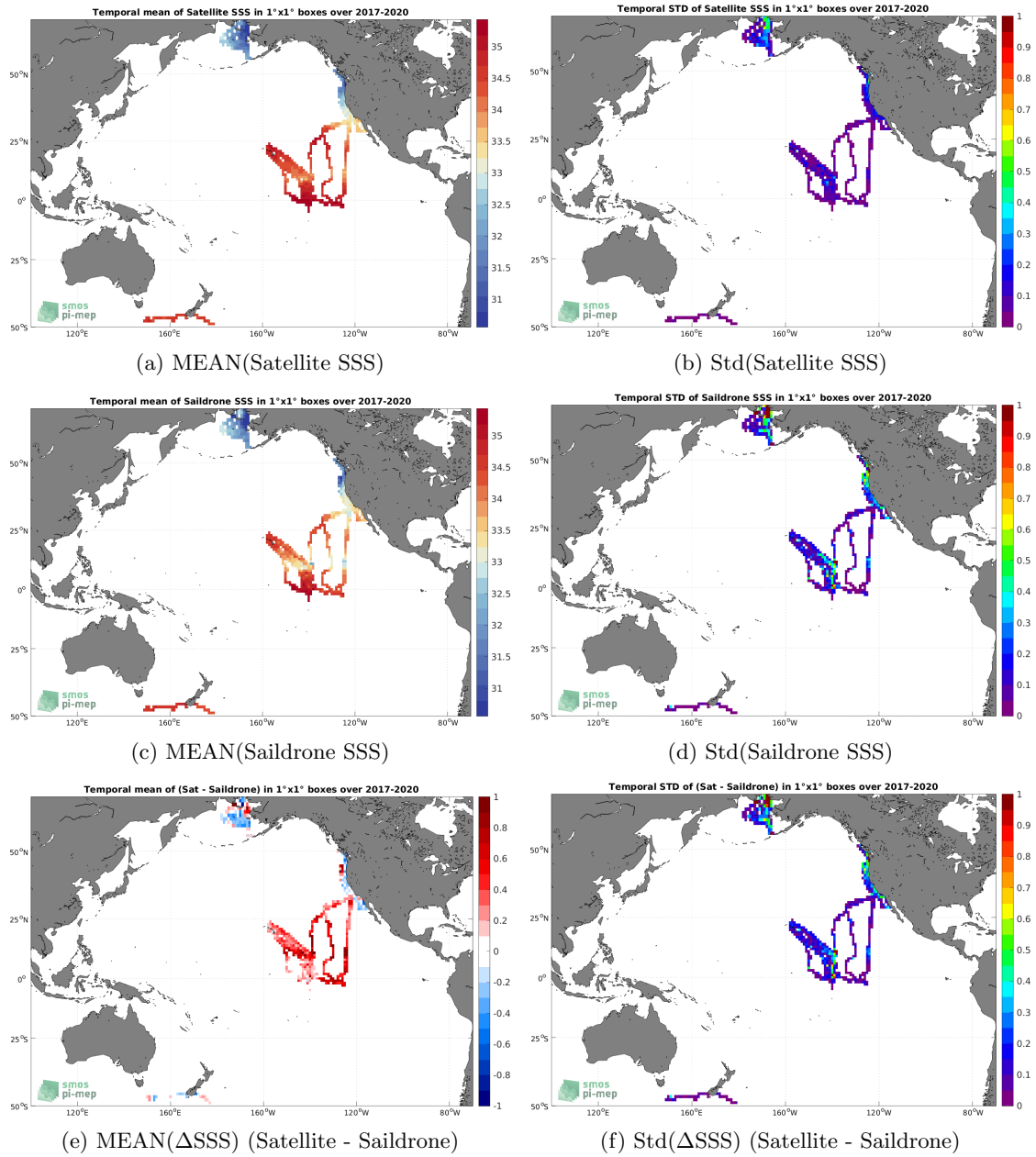
Figure 6: Temporal mean (left) and Std (right) of SSS from SMOS SSS L4 v2 - Daily (BEC) (top), Saildrone (middle), and of \Delta SSS (Satellite - Saildrone). Only match-up pairs are used to generate these maps.
