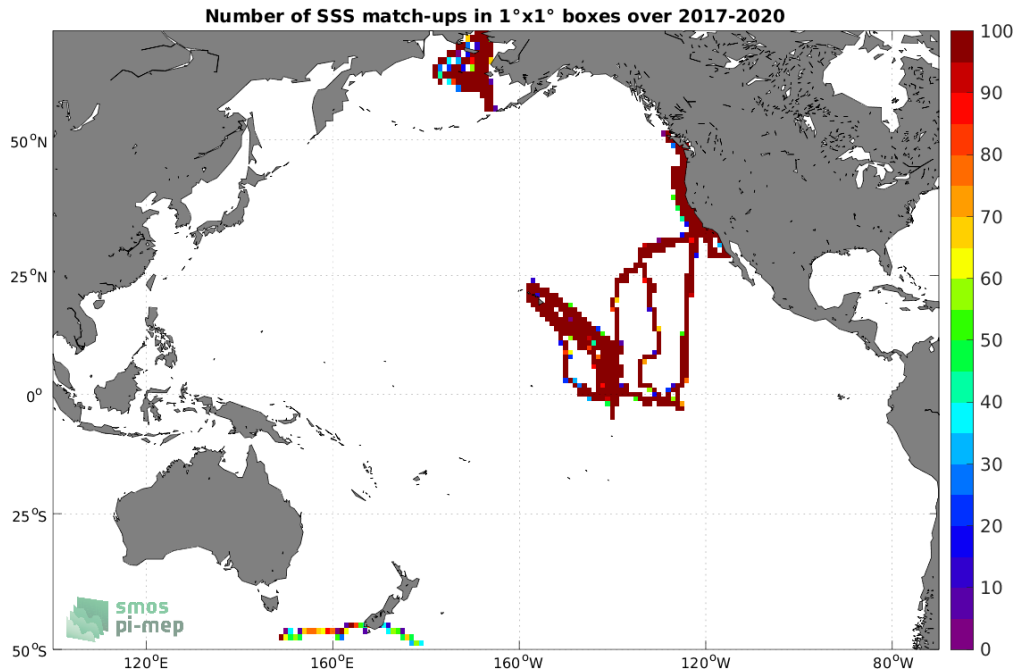
Figure 4: Number of SSS match-ups between Saildrone SSS and the SMOS SSS L4 v2 - Daily (BEC) SSS product for the Pacific Ocean Pi-MEP region over 1^\circ \times 1^\circ boxes and for the full satellite product period.
