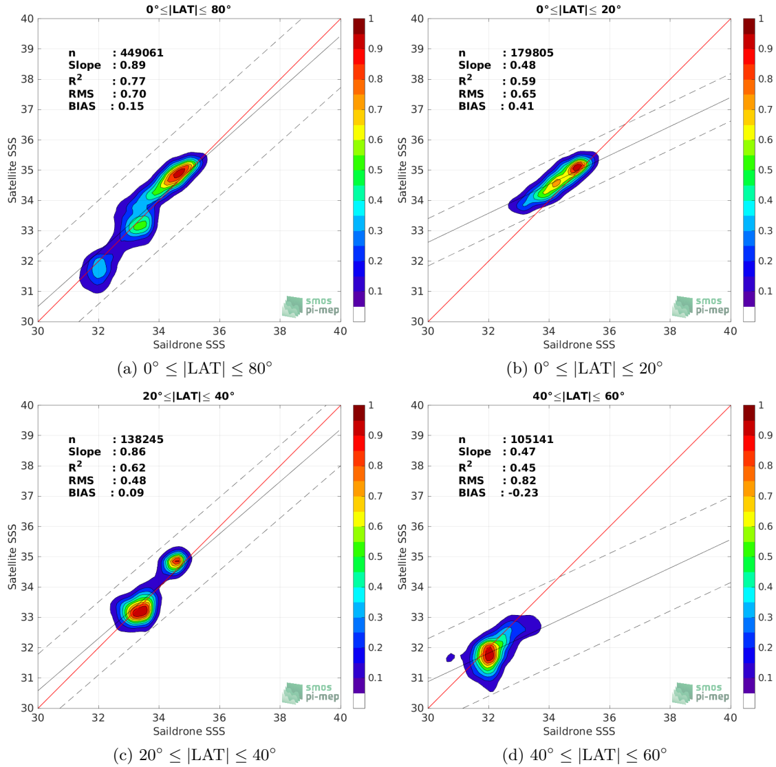
Figure 9: Contour maps of the concentration of SMOS SSS L4 v2 - Daily (BEC) SSS (y-axis) versus Saildrone SSS (x-axis) at match-up pairs for different latitude bands. For each plot, the red line shows x=y . The black thin and dashed lines indicate a linear fit through the data cloud and the \pm 95\% confidence levels, respectively. The number match-up pairs n , the slope and R^2 coefficient of the linear fit, the root mean square (RMS) and the mean bias between satellite and in situ data are indicated for each latitude band in each plots.
