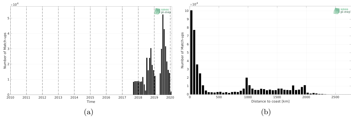
Figure 1: Number of match-ups between Saildrone and SMOS SSS L4 v2 - Daily (BEC) SSS as a function of time (a) and as function of the distance to coast (b) over the Pacific Ocean Pi-MEP region and for the full satellite product period.
