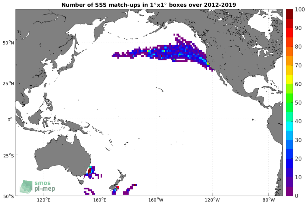
Figure 4: Number of SSS match-ups between Marine mammals SSS and the SMOS SSS L4 v2 - Daily (BEC) SSS product for the Pacific Ocean Pi-MEP region over 1^\circ \times 1^\circ boxes and for the full satellite product period.
