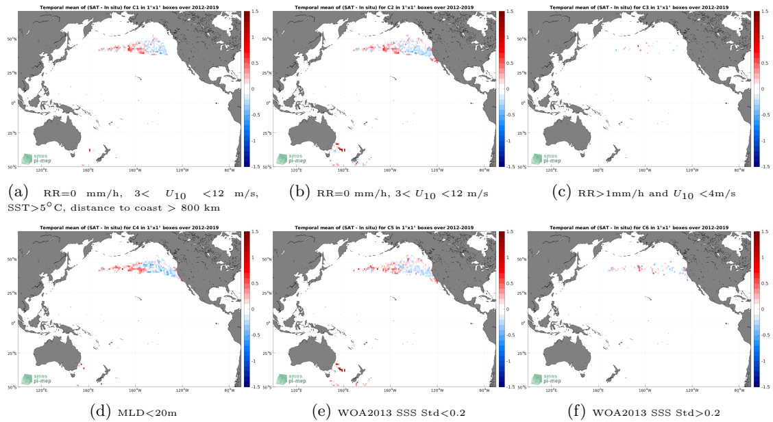
Figure 12: Temporal mean gridded over spatial boxes of size 1^\circ \times 1^\circ of \Delta SSS (SMOS SSS L4 v2 - Daily (BEC) - Marine mammals) for 6 different subdatasets corresponding to:RR=0 mm/h, 3 < U_{10} < 12 m/s, SST >5^\circ C, distance to coast > 800 km (a), RR=0 mm/h, 3 < U_{10} < 12 m/s (b), RR >1 mm/h and U_{10} < 4 m/s (c),MLD <20 m (d),WOA2013 SSS Std <0.2 (e),WOA2013 SSS Std >0.2 (f).
