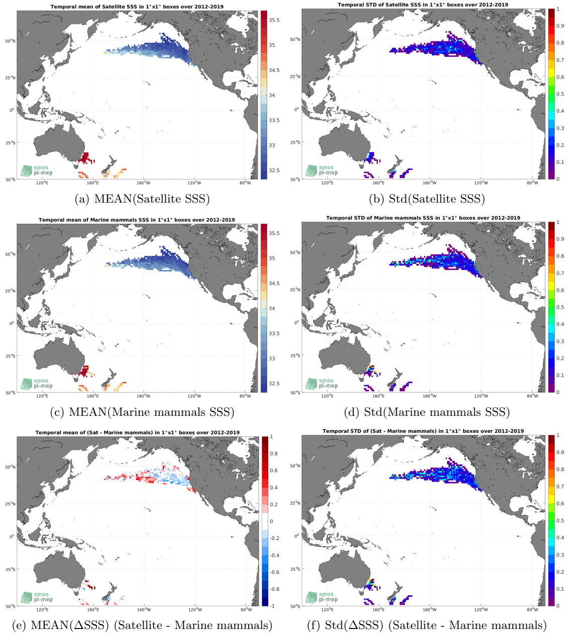
Figure 6: Temporal mean (left) and Std (right) of SSS from SMOS SSS L4 v2 - Daily (BEC) (top), Marine mammals (middle), and of \Delta SSS (Satellite - Marine mammals). Only match-up pairs are used to generate these maps.
