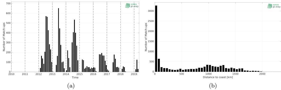
Figure 1: Number of match-ups between Marine mammals and SMOS SSS L4 v2 - Daily (BEC) SSS as a function of time (a) and as function of the distance to coast (b) over the Pacific Ocean Pi-MEP region and for the full satellite product period.
