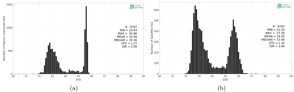
Figure 2: Histograms of SSS from Marine mammals (a) and SMOS SSS L4 v2 - Daily (BEC) (b) considering all match-up pairs per bins of 0.1 over the Pacific Ocean Pi-MEP region and for the full satellite product period.
