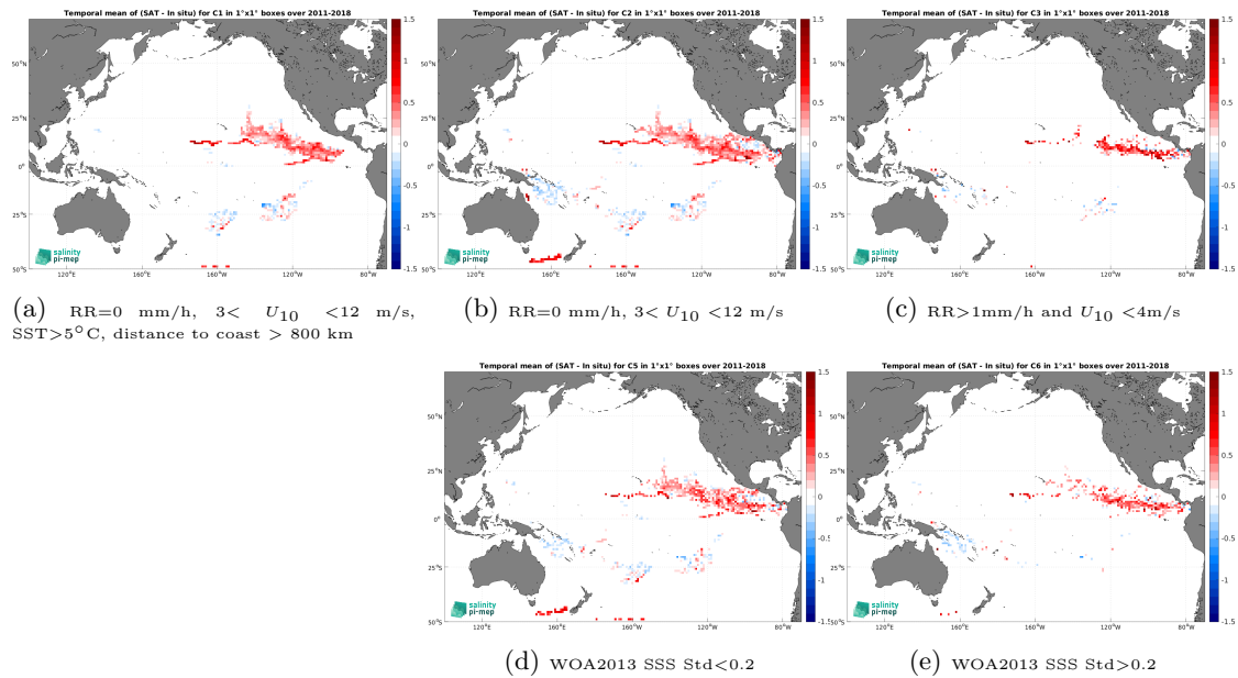
Figure 13: Temporal mean gridded over spatial boxes of size 1^\circ \times 1^\circ of \Delta\text{SSS} (SMOS SSS L4 v2 - Daily (BEC) - Surface drifters) for 5 different subdatasets corresponding to:RR=0 mm/h, 3 < U_{10} < 12 m/s, SST >5^\circ\text{C} , distance to coast > 800 km (a), RR=0 mm/h, 3 < U_{10} < 12 m/s (b), RR >1 mm/h and U_{10} < 4 m/s (c), WOA2013 SSS Std <0.2 (d), WOA2013 SSS Std >0.2 (e).
