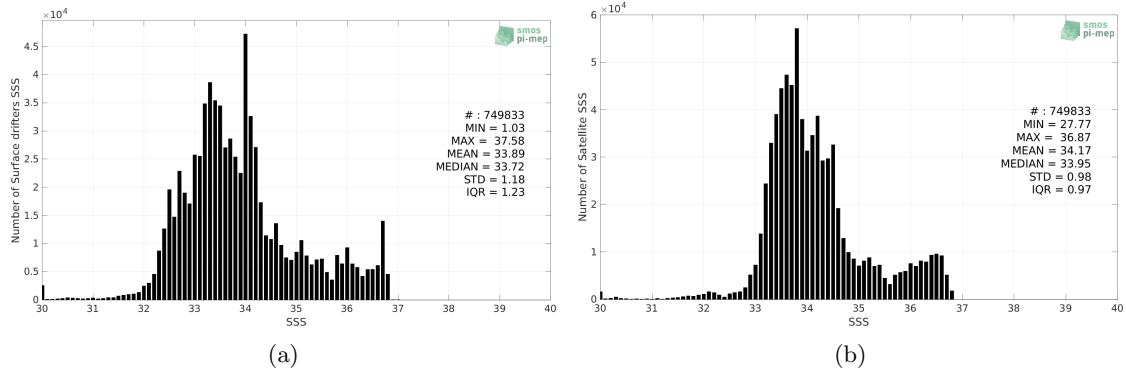
Figure 2: Histograms of SSS from Surface drifters (a) and SMOS SSS L4 v2 - Daily (BEC) (b) considering all match-up pairs per bins of 0.1 over the Pacific Ocean Pi-MEP region and for the full satellite product period.
