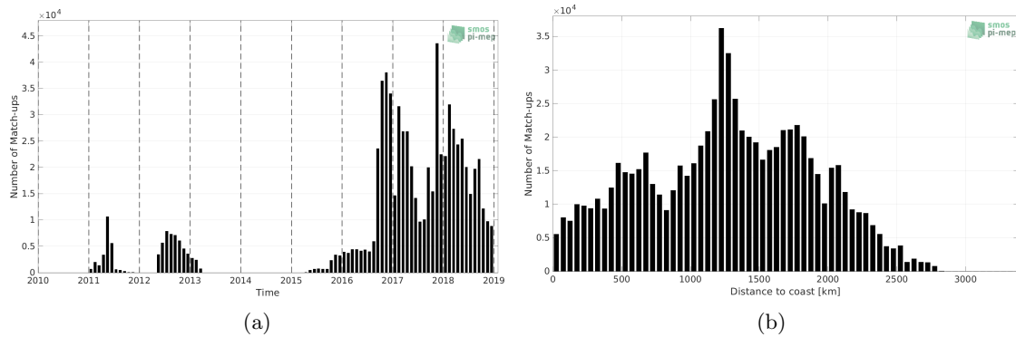
Figure 1: Number of match-ups between Surface drifters and SMOS SSS L4 v2 - Daily (BEC) SSS as a function of time (a) and as function of the distance to coast (b) over the Pacific Ocean Pi-MEP region and for the full satellite product period.
