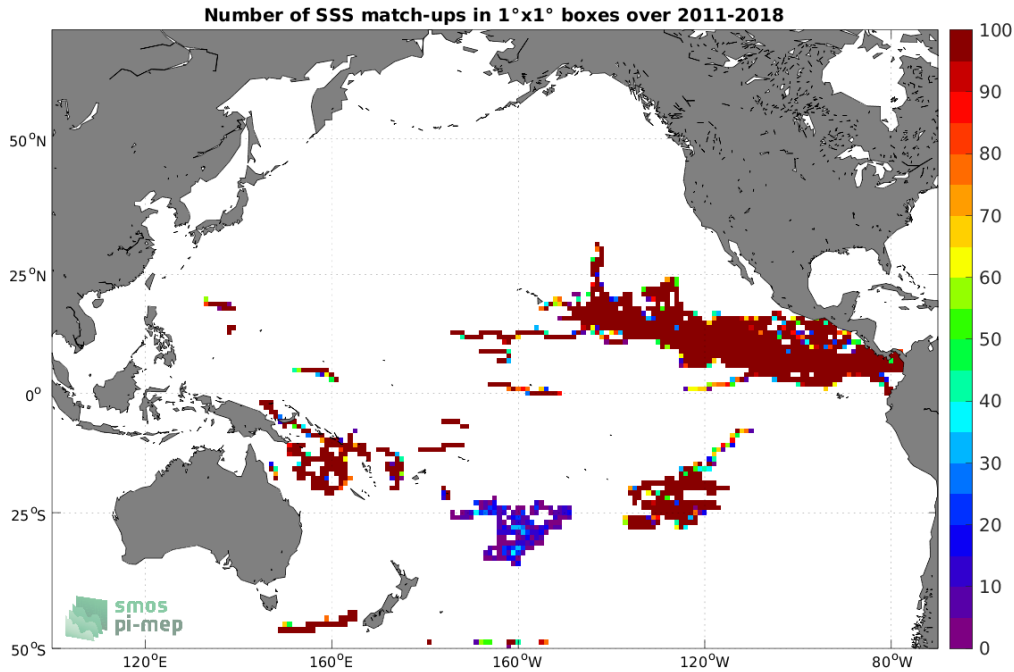
Figure 3: Number of SSS match-ups between Surface drifters SSS and the SMOS SSS L4 v2 - Daily (BEC) SSS product for the Pacific Ocean Pi-MEP region over 1^\circ \times 1^\circ boxes and for the full satellite product period.
