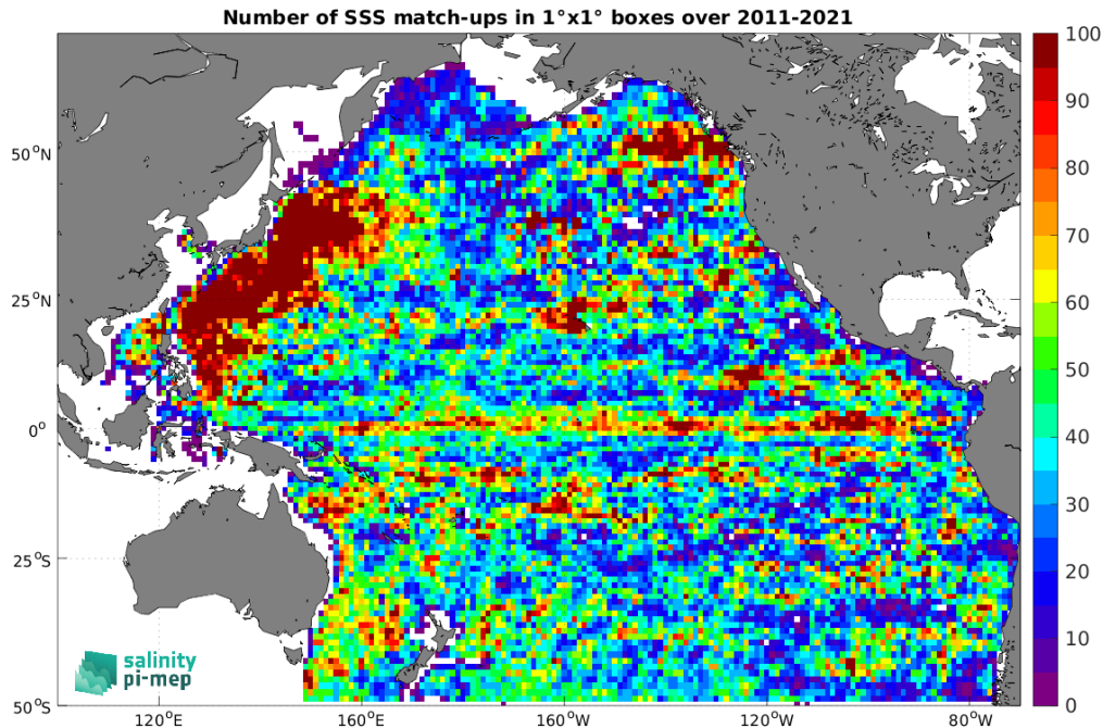
Figure 4: Number of SSS match-ups between Argo SSS and the SMOS SSS L4 v2 - Daily (BEC) SSS product for the Pacific Ocean Pi-MEP region over 1^{\circ} \times 1^{\circ} boxes and for the full satellite product period.
