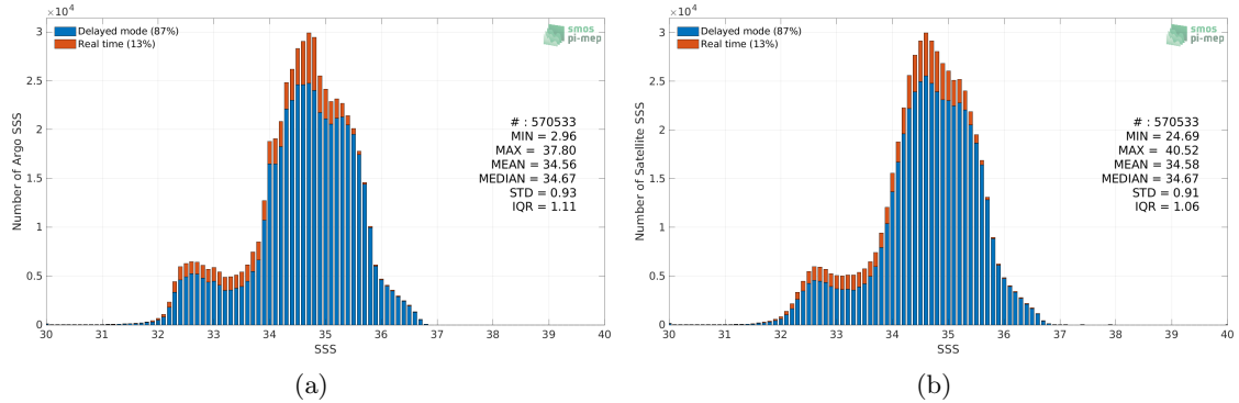
Figure 2: Histograms of SSS from Argo (a) and SMOS SSS L4 v2 - Daily (BEC) (b) considering all match-up pairs per bins of 0.1 over the Pacific Ocean Pi-MEP region and for the full satellite product period.
