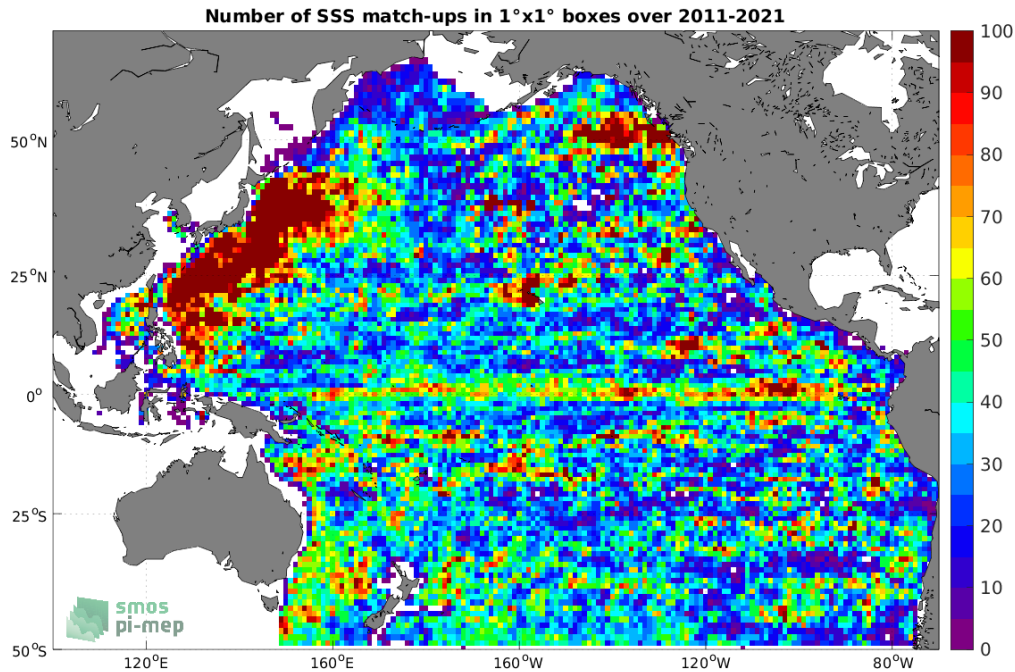
Figure 4: Number of SSS match-ups between Argo SSS and the SMOS SSS L4 v2 - Daily (BEC) SSS product for the Pacific Ocean Pi-MEP region over 1^\circ \times 1^\circ boxes and for the full satellite product period.
