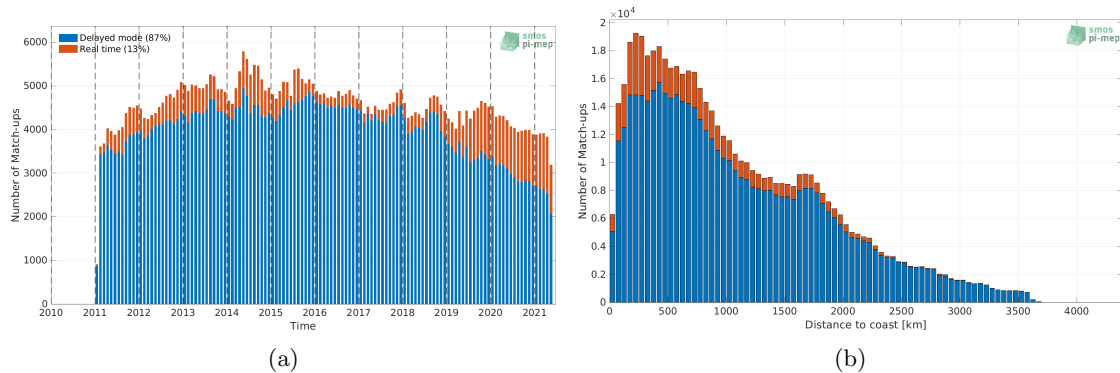
Figure 1: Number of match-ups between Argo and SMOS SSS L4 v2 - Daily (BEC) SSS as a function of time (a) and as function of the distance to coast (b) over the Pacific Ocean Pi-MEP region and for the full satellite product period.
