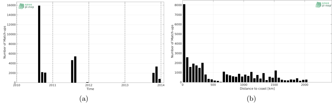
Figure 1: Number of match-ups between TSG-GOSUD-Sailing-ship and SMOS-L3-ICDC-V3-MONTHLY-0.5DEG SSS as a function of time (a) and as function of the distance to coast (b) over the Pacific Ocean Pi-MEP region and for the full satellite product period.
