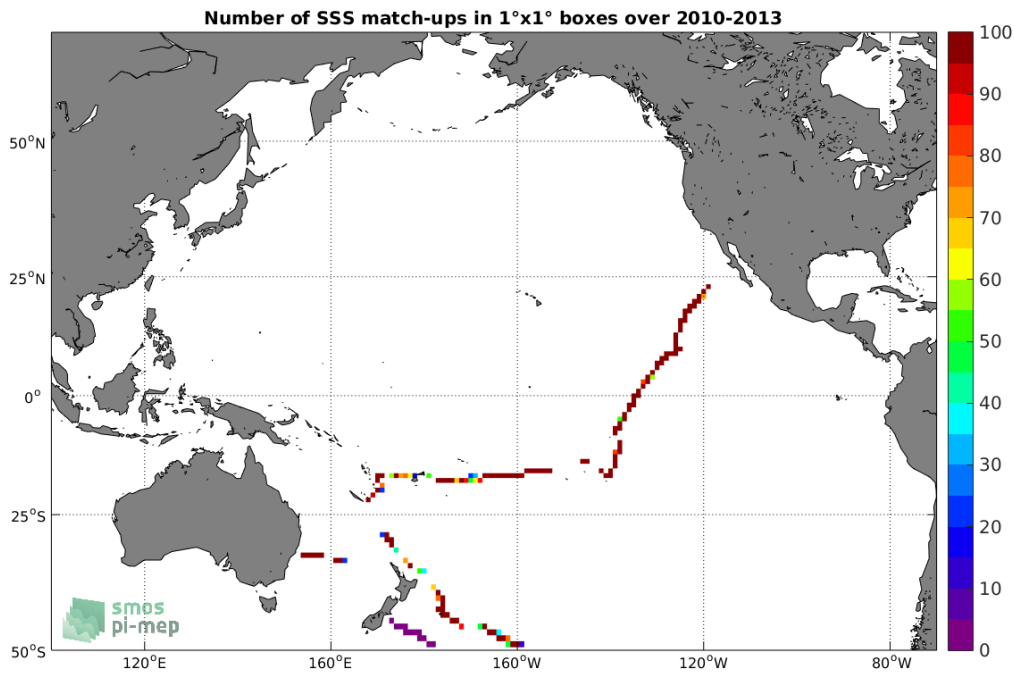
Figure 4: Number of SSS match-ups between TSG-GOSUD-Sailing-ship SSS and the SMOS-L3-ICDC-V3-MONTHLY-0.5DEG SSS product for the Pacific Ocean Pi-MEP region over 1^{\circ} \times 1^{\circ} boxes and for the full satellite product period.
