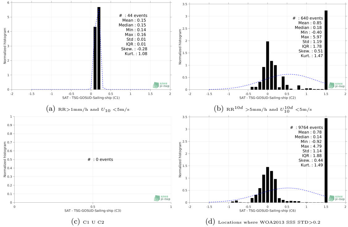
Figure 13: Normalized histogram of \Delta SSS (SMOS-L3-ICDC-V3-MONTHLY-0.5DEG - TSG-GOSUD-Sailing-ship) for 6 different subdatasets corresponding to: RR > 1\text{mm/h} and U_{10} < 5\text{m/s} (a), RR^{10d} > 5\text{mm/h} and U_{10}^{10d} < 5\text{m/s} (b), C1 U C2 (c), Locations where WOA2013 SSS STD > 0.2 (d).
