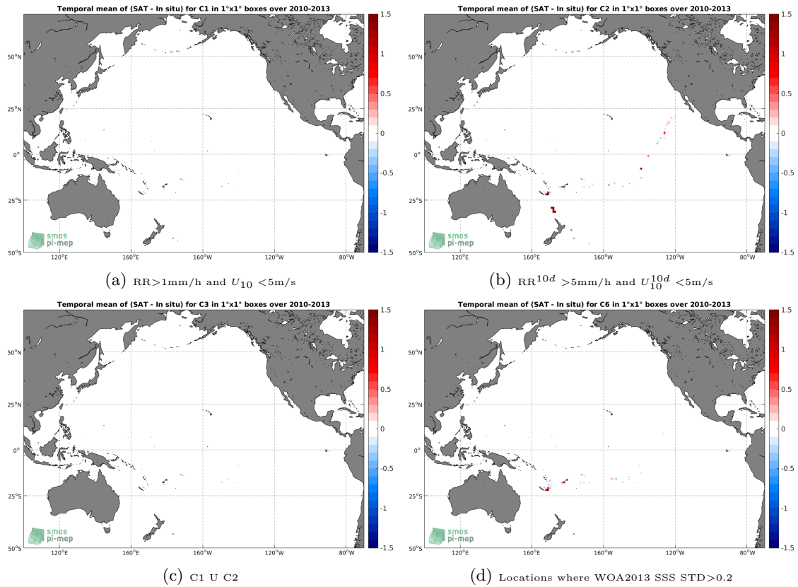
Figure 12: Temporal mean gridded over spatial boxes of size 1^\circ \times 1^\circ of \Delta SSS (SMOS-L3-ICDC-V3-MONTHLY-0.5DEG - TSG-GOSUD-Sailing-ship) for 4 different subdatasets corresponding to: RR > 1mm/h and U_{10} < 5\text{m/s} (a), RR^{10d} > 5\text{mm/h} and U_{10}^{10d} < 5\text{m/s} (b), C1 U C2 (c), Locations where WOA2013 SSS STD > 0.2 (d).
