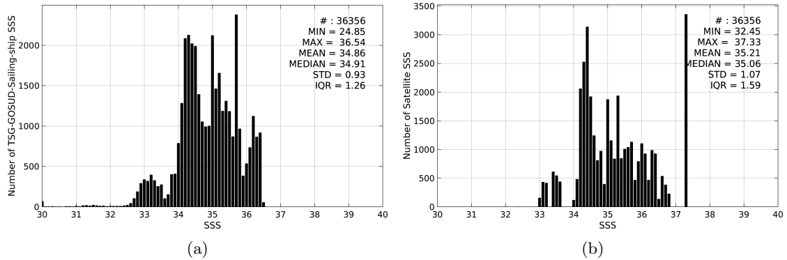
Figure 2: Histograms of SSS from TSG-GOSUD-Sailing-ship (a) and SMOS-L3-ICDC-V3-MONTHLY-0.5DEG (b) considering all match-up pairs per bins of 0.1 over the Pacific Ocean Pi-MEP region and for the full satellite product period.
