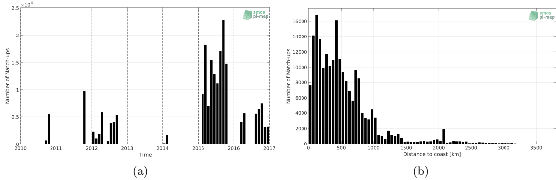
Figure 1: Number of match-ups between TSG (GOSUD-Research-vessel) and SMOS SSS L3 v3 Monthly (ICDC) SSS as a function of time (a) and as function of the distance to coast (b) over the Pacific Ocean Pi-MEP region and for the full satellite product period.
