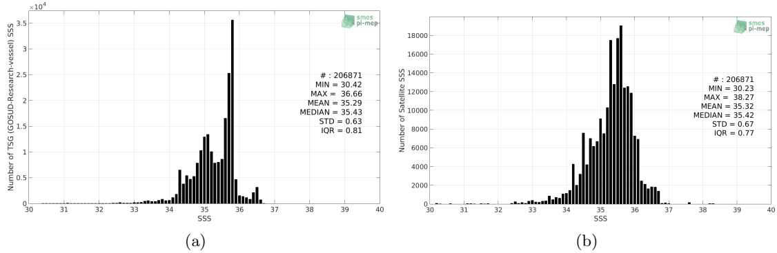
Figure 2: Histograms of SSS from TSG (GOSUD-Research-vessel) (a) and SMOS SSS L3 v3 Monthly (ICDC) (b) considering all match-up pairs per bins of 0.1 over the Pacific Ocean Pi-MEP region and for the full satellite product period.
