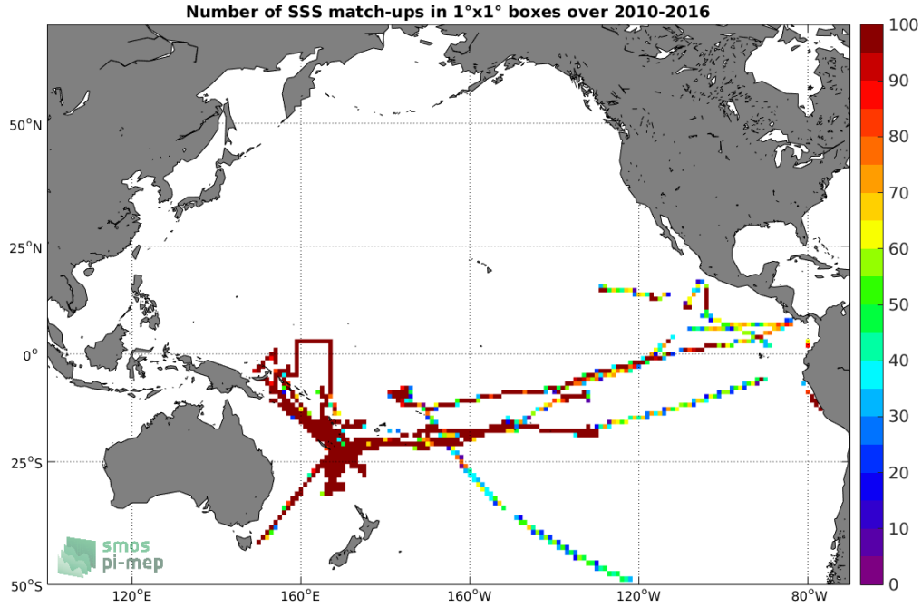
Figure 4: Number of SSS match-ups between TSG (GOSUD-Research-vessel) SSS and the SMOS SSS L3 v3 Monthly (ICDC) SSS product for the Pacific Ocean Pi-MEP region over 1^\circ \times 1^\circ boxes and for the full satellite product period.
