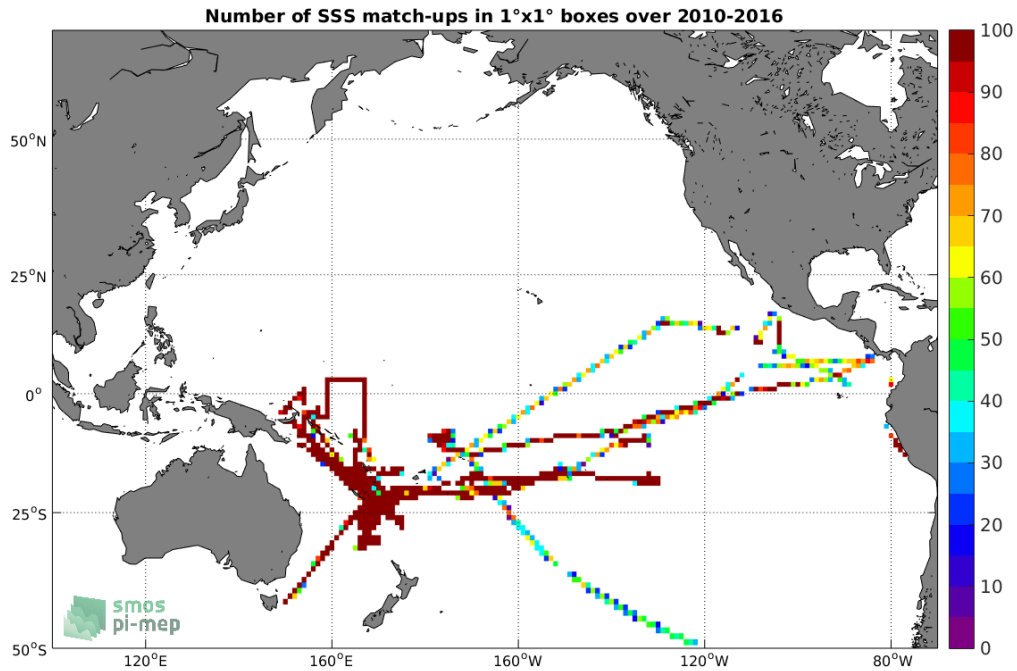
Figure 4: Number of SSS match-ups between TSG-GOSUD-Research-vessel SSS and the SMOS-L3-ICDC-V3-MONTHLY-0.5DEG SSS product for the Pacific Ocean Pi-MEP region over 1^\circ \times 1^\circ boxes and for the full satellite product period.
