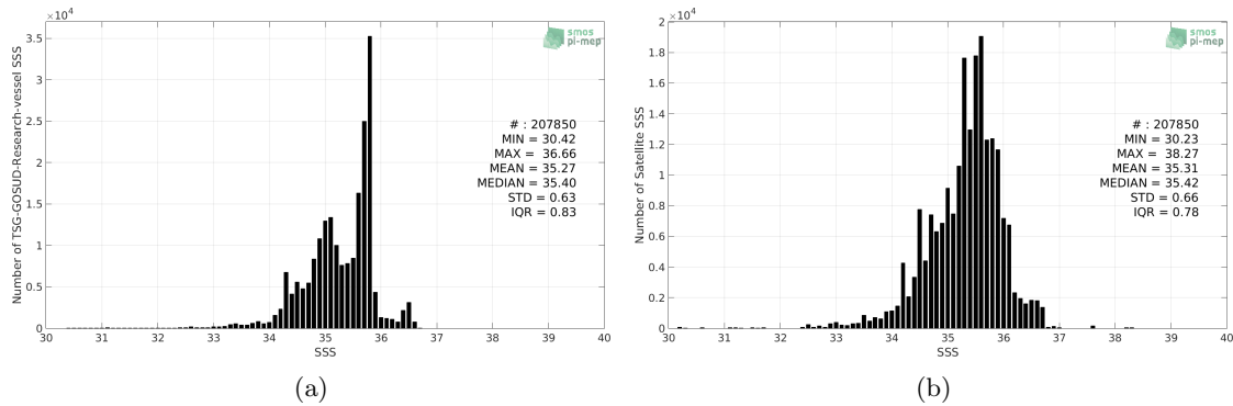
Figure 2: Histograms of SSS from TSG-GOSUD-Research-vessel (a) and SMOS-L3-ICDC-V3-MONTHLY-0.5DEG (b) considering all match-up pairs per bins of 0.1 over the Pacific Ocean Pi-MEP region and for the full satellite product period.
