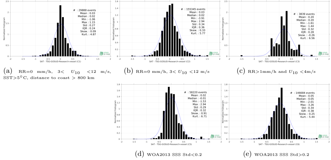
Figure 13: Normalized histogram of \Delta SSS (SMOS-L3-ICDC-V3-MONTHLY-0.5DEG - TSG-GOSUD-Research-vessel) for 5 different subdatasets corresponding to: RR=0 mm/h, 3 < U_{10} < 12 m/s, SST > 5°C, distance to coast > 800 km (a), RR=0 mm/h, 3 < U_{10} < 12 m/s (b), RR > 1mm/h and U_{10} < 4 m/s (c), WOA2013 SSS Std < 0.2 (d), WOA2013 SSS Std > 0.2 (e).
