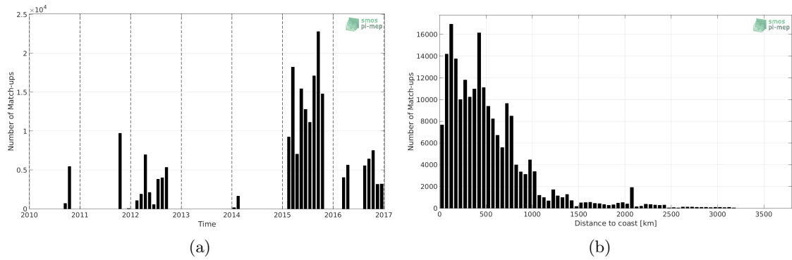
Figure 1: Number of match-ups between TSG-GOSUD-Research-vessel and SMOS-L3-ICDC-V3-MONTHLY-0.5DEG SSS as a function of time (a) and as function of the distance to coast (b) over the Pacific Ocean Pi-MEP region and for the full satellite product period.
