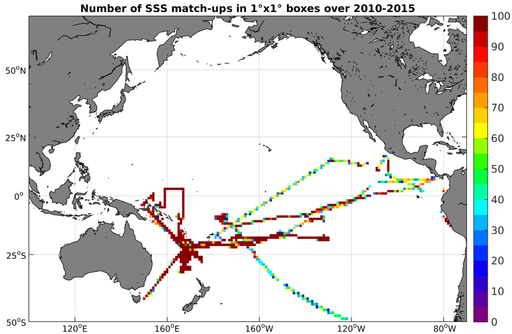
Figure 4: Number of SSS match-ups between TSG-GOSUD-Research-vessel SSS and the SMOS-L3-ICDC-V3-MONTHLY-0.5DEG SSS product for the Pacific Ocean Pi-MEP region over 1^\circ \times 1^\circ boxes and for the full satellite product period.
