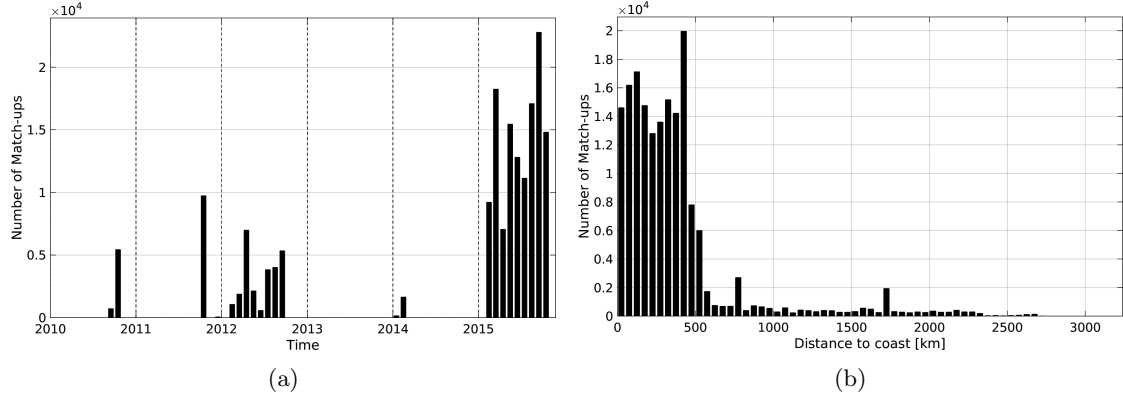
Figure 1: Number of match-ups between TSG-GOSUD-Research-vessel and SMOS-L3-ICDC-V3-MONTHLY-0.5DEG SSS as a function of time (a) and as function of the distance to coast (b) over the Pacific Ocean Pi-MEP region and for the full satellite product period.
