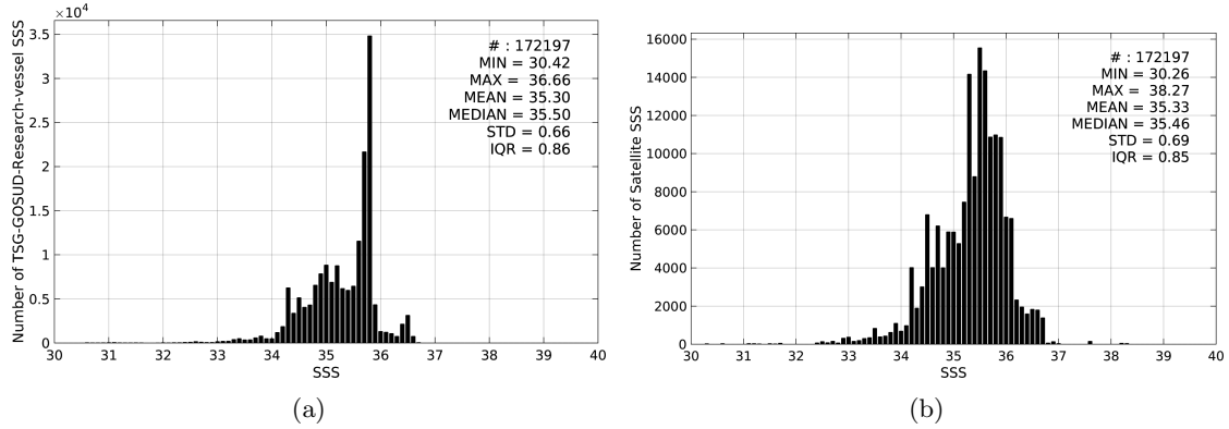
Figure 2: Histograms of SSS from TSG-GOSUD-Research-vessel (a) and SMOS-L3-ICDC-V3-MONTHLY-0.5DEG (b) considering all match-up pairs per bins of 0.1 over the Pacific Ocean Pi-MEP region and for the full satellite product period.
