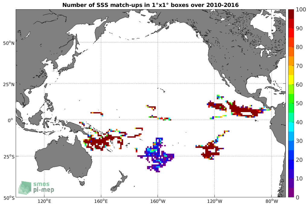
Figure 3: Number of SSS match-ups between Surface drifters SSS and the SMOS SSS L3 v3 Monthly (ICDC) SSS product for the Pacific Ocean Pi-MEP region over 1^\circ \times 1^\circ boxes and for the full satellite product period.
