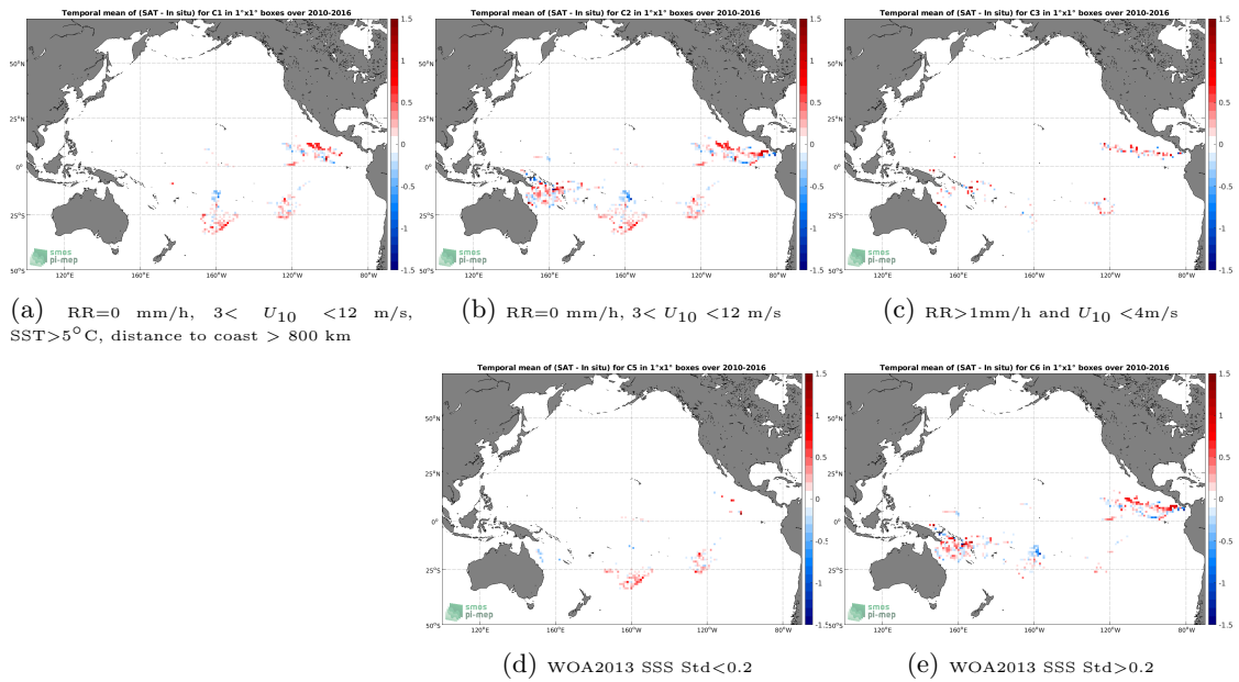
Figure 11: Temporal mean gridded over spatial boxes of size 1°x1° of \Delta SSS (SMOS SSS L3 v3 Monthly (ICDC) - Surface drifters) for 5 different subdatasets corresponding to: RR=0 mm/h, 3 < U_{10} < 12 m/s, SST > 5°C, distance to coast > 800 km (a), RR=0 mm/h, 3 < U_{10} < 12 m/s (b), RR > 1mm/h and U_{10} < 4 m/s (c), WOA2013 SSS Std < 0.2 (d), WOA2013 SSS Std > 0.2 (e).
