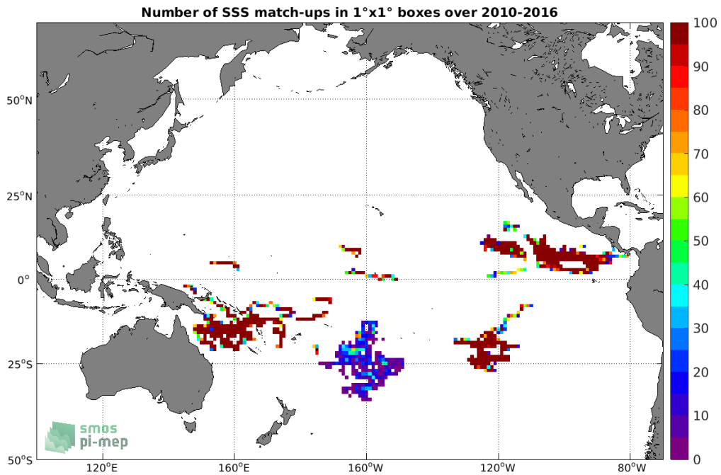
Figure 3: Number of SSS match-ups between Surface drifters SSS and the SMOS SSS L3 v3 Monthly (ICDC) SSS product for the Pacific Ocean Pi-MEP region over 1°x1° boxes and for the full satellite product period.
