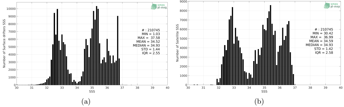
Figure 2: Histograms of SSS from Surface drifters (a) and SMOS SSS L3 v3 Monthly (ICDC) (b) considering all match-up pairs per bins of 0.1 over the Pacific Ocean Pi-MEP region and for the full satellite product period.
