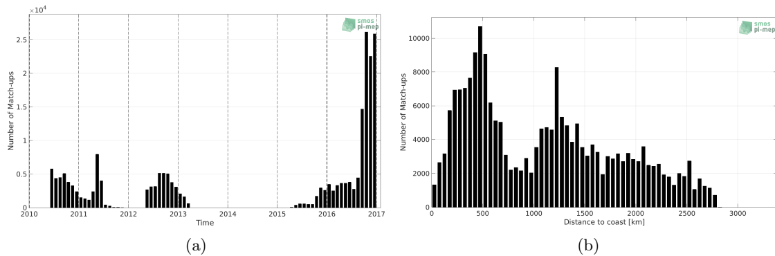
Figure 1: Number of match-ups between Surface drifters and SMOS SSS L3 v3 Monthly (ICDC) SSS as a function of time (a) and as function of the distance to coast (b) over the Pacific Ocean Pi-MEP region and for the full satellite product period.
