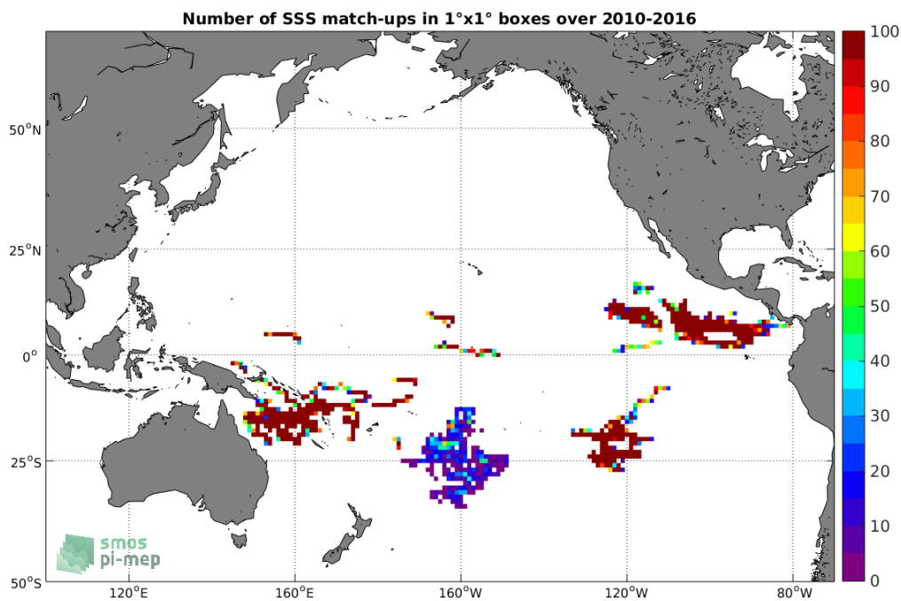
Figure 3: Number of SSS match-ups between Surface drifters SSS and the SMOS-L3-ICDC-V3-MONTHLY-0.5DEG SSS product for the Pacific Ocean Pi-MEP region over 1^\circ \times 1^\circ boxes and for the full satellite product period.
