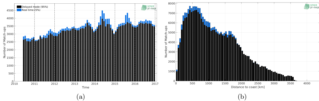
Figure 1: Number of match-ups between Argo and SMOS SSS L3 v3 Monthly (ICDC) SSS as a function of time (a) and as function of the distance to coast (b) over the Pacific Ocean Pi-MEP region and for the full satellite product period.
