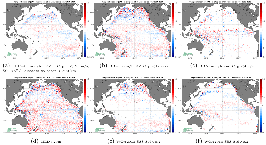
Figure 12: Temporal mean gridded over spatial boxes of size 1^\circ \times 1^\circ of \Delta SSS (SMOS SSS L3 v3 Monthly (ICDC) - Argo) for 6 different subdatasets corresponding to: RR=0 mm/h, 3 < U_{10} < 12 m/s, SST > 5^\circ\text{C} , distance to coast > 800 km (a), RR=0 mm/h, 3 < U_{10} < 12 m/s (b), RR > 1 mm/h and U_{10} < 4 m/s (c), MLD < 20 m (d), WOA2013 SSS Std < 0.2 (e), WOA2013 SSS Std > 0.2 (f).
