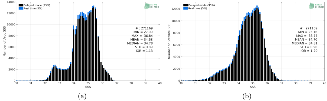
Figure 2: Histograms of SSS from Argo (a) and SMOS SSS L3 v3 Monthly (ICDC) (b) considering all match-up pairs per bins of 0.1 over the Pacific Ocean Pi-MEP region and for the full satellite product period.
