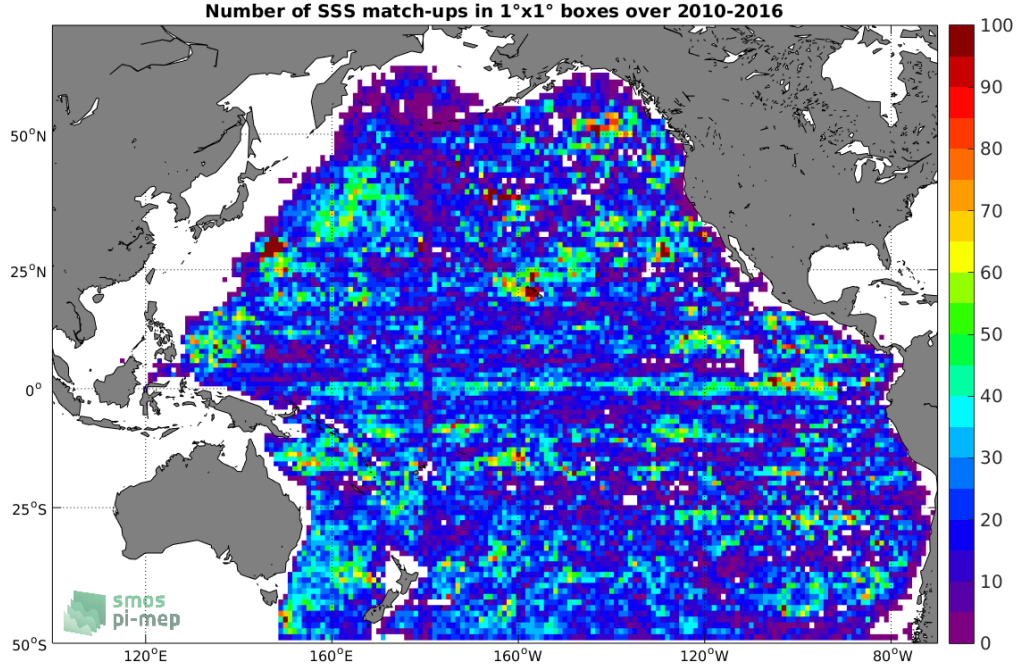
Figure 4: Number of SSS match-ups between Argo SSS and the SMOS SSS L3 v3 Monthly (ICDC) SSS product for the Pacific Ocean Pi-MEP region over 1^\circ \times 1^\circ boxes and for the full satellite product period.
