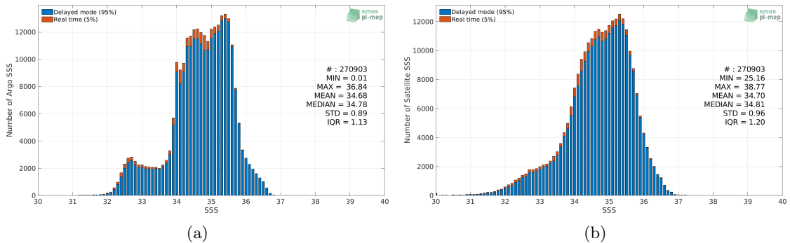
Figure 2: Histograms of SSS from Argo (a) and SMOS SSS L3 v3 Monthly (ICDC) (b) considering all match-up pairs per bins of 0.1 over the Pacific Ocean Pi-MEP region and for the full satellite product period.
