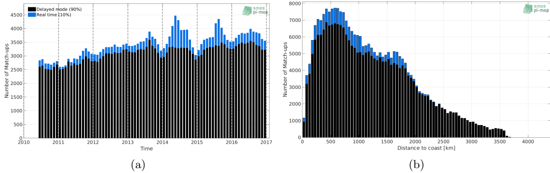
Figure 1: Number of match-ups between Argo and SMOS-L3-ICDC-V3-MONTHLY-0.5DEG SSS as a function of time (a) and as function of the distance to coast (b) over the Pacific Ocean Pi-MEP region and for the full satellite product period.
