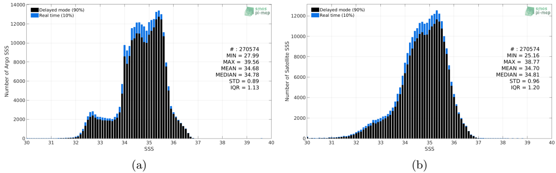
Figure 2: Histograms of SSS from Argo (a) and SMOS-L3-ICDC-V3-MONTHLY-0.5DEG (b) considering all match-up pairs per bins of 0.1 over the Pacific Ocean Pi-MEP region and for the full satellite product period.
