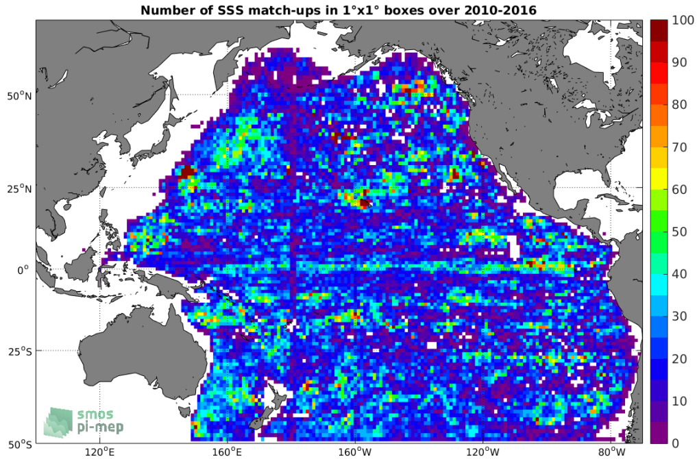
Figure 4: Number of SSS match-ups between Argo SSS and the SMOS-L3-ICDC-V3-MONTHLY-0.5DEG SSS product for the Pacific Ocean Pi-MEP region over 1^\circ \times 1^\circ boxes and for the full satellite product period.
