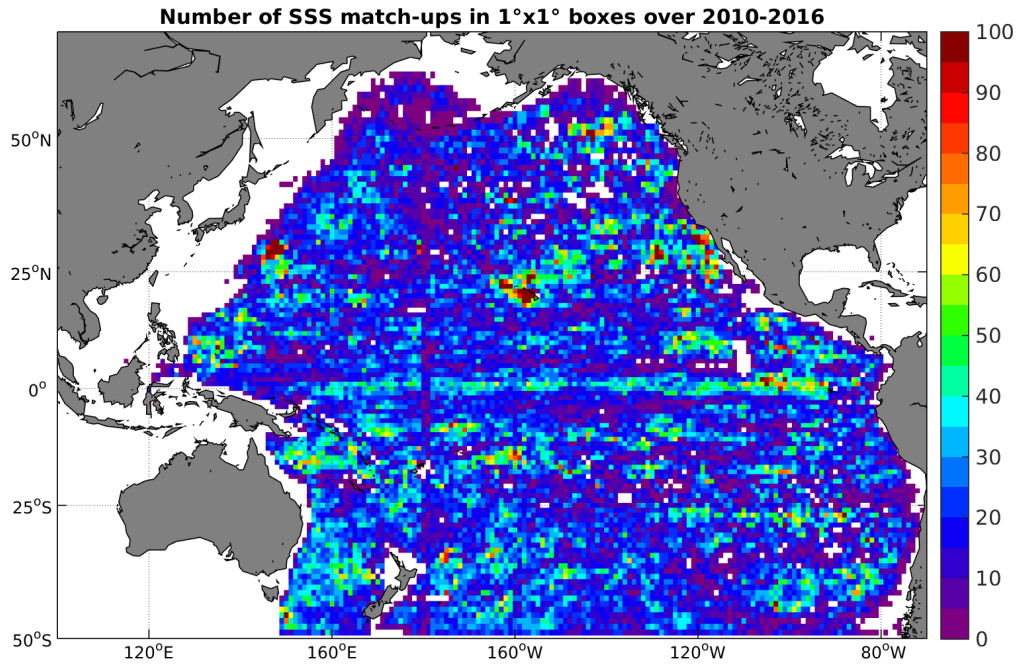
Figure 4: Number of SSS match-ups between Argo SSS and the SMOS-L3-ICDC-V3-MONTHLY-0.5DEG SSS product for the Pacific Ocean Pi-MEP region over 1^\circ \times 1^\circ boxes and for the full satellite product period.
