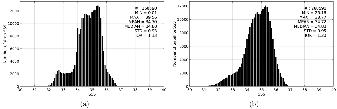
Figure 2: Histograms of SSS from Argo (a) and SMOS-L3-ICDC-V3-MONTHLY-0.5DEG (b) considering all match-up pairs per bins of 0.1 over the Pacific Ocean Pi-MEP region and for the full satellite product period.
