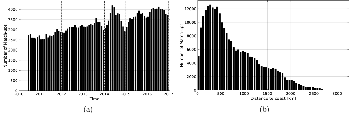
Figure 1: Number of match-ups between Argo and SMOS-L3-ICDC-V3-MONTHLY-0.5DEG SSS as a function of time (a) and as function of the distance to coast (b) over the Pacific Ocean Pi-MEP region and for the full satellite product period.
