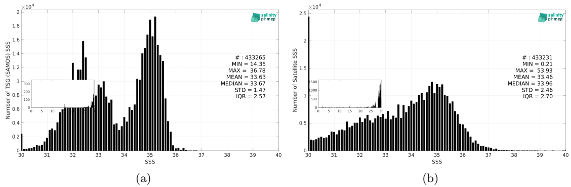
Figure 3: Histograms of SSS from TSG (SAMOS) (a) and SMOS SSS L2Q v331 - With FLAG (CMEMS-CATDS-CPDC) (b) considering all match-up pairs per bins of 0.1 over the Pacific Ocean Pi-MEP region and for the full satellite product period.
