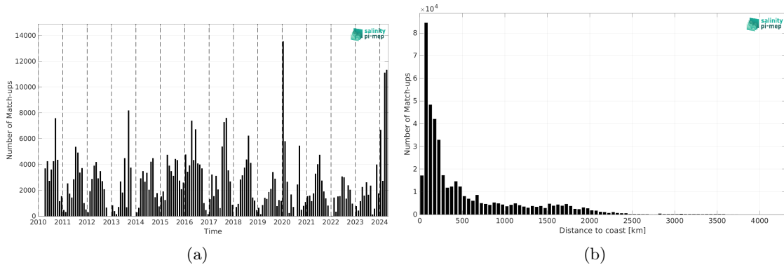
Figure 2: Number of match-ups between TSG (SAMOS) and SMOS SSS L2Q v331 - With FLAG (CMEMS-CATDS-CPDC) SSS as a function of time (a) and as function of the distance to coast (b) over the Pacific Ocean Pi-MEP region and for the full satellite product period.
