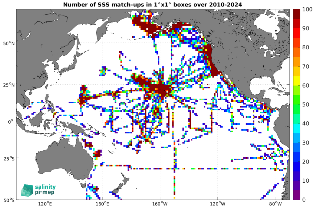
Figure 5: Number of SSS match-ups between TSG (SAMOS) SSS and the SMOS SSS L2Q v331 - With FLAG (CMEMS-CATDS-CPDC) SSS product for the Pacific Ocean Pi-MEP region over 1^\circ \times 1^\circ boxes and for the full satellite product period.
