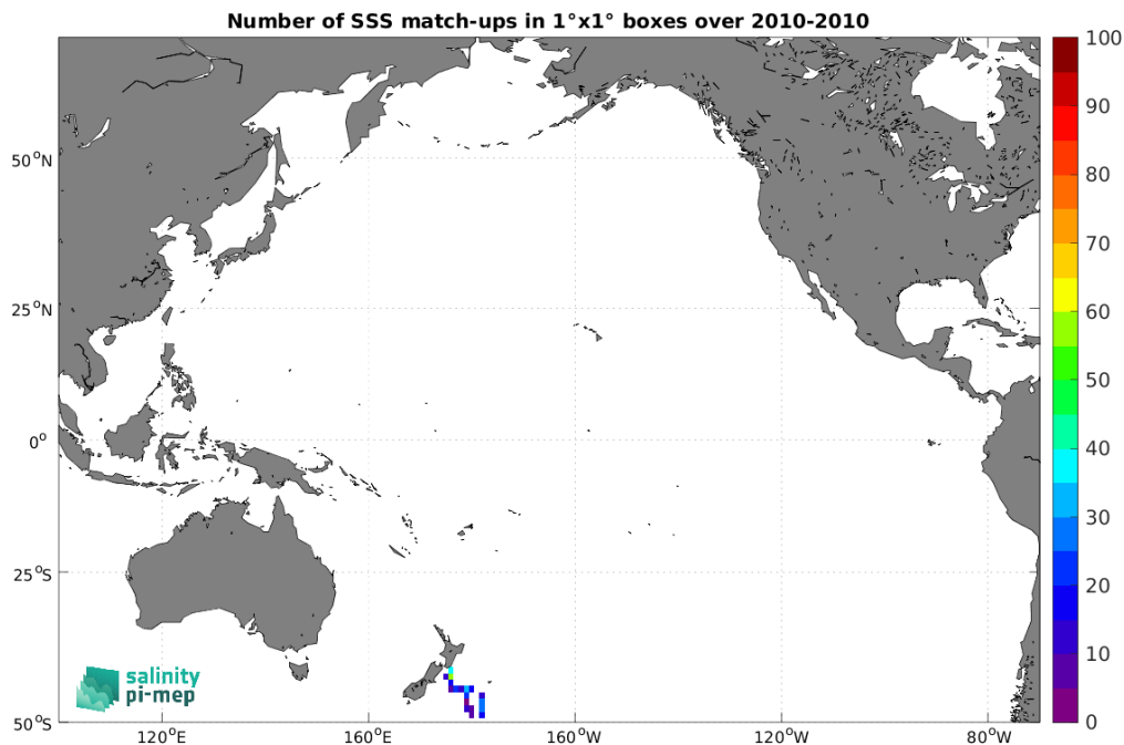
Figure 5: Number of SSS match-ups between TSG (Polarstern) SSS and the SMOS SSS L2Q v331 - With FLAG (CMEMS-CATDS-CPDC) SSS product for the Pacific Ocean Pi-MEP region over 1^\circ \times 1^\circ boxes and for the full satellite product period.
