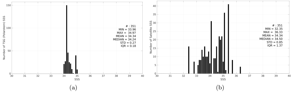
Figure 3: Histograms of SSS from TSG (Polarstern) (a) and SMOS SSS L2Q v331 - With FLAG (CMEMS-CATDS-CPDC) (b) considering all match-up pairs per bins of 0.1 over the Pacific Ocean Pi-MEP region and for the full satellite product period.
