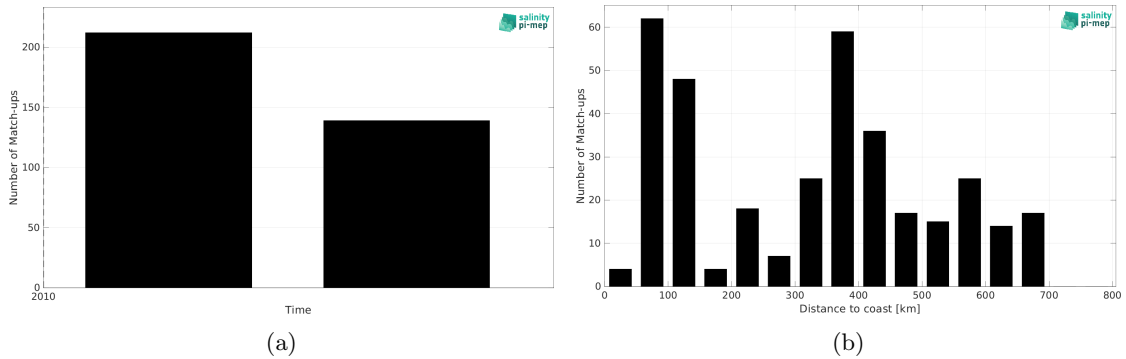
Figure 2: Number of match-ups between TSG (Polarstern) and SMOS SSS L2Q v331 - With FLAG (CMEMS-CATDS-CPDC) SSS as a function of time (a) and as function of the distance to coast (b) over the Pacific Ocean Pi-MEP region and for the full satellite product period.
