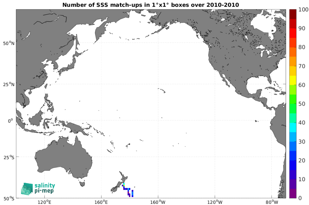
Figure 4: Number of SSS match-ups between TSG (Polarstern) SSS and the SMOS SSS L2Q v331 - With FLAG (CMEMS-CATDS-CPDC) SSS product for the Pacific Ocean Pi-MEP region over 1^\circ \times 1^\circ boxes and for the full satellite product period.
