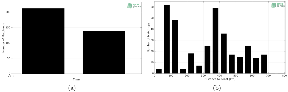
Figure 1: Number of match-ups between TSG (Polarstern) and SMOS SSS L2Q v331 - With FLAG (CMEMS-CATDS-CPDC) SSS as a function of time (a) and as function of the distance to coast (b) over the Pacific Ocean Pi-MEP region and for the full satellite product period.
