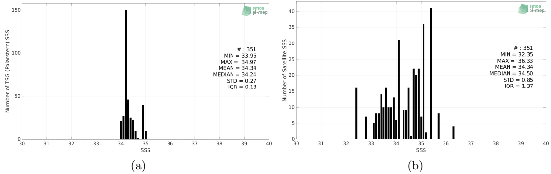
Figure 2: Histograms of SSS from TSG (Polarstern) (a) and SMOS SSS L2Q v331 - With FLAG (CMEMS-CATDS-CPDC) (b) considering all match-up pairs per bins of 0.1 over the Pacific Ocean Pi-MEP region and for the full satellite product period.
