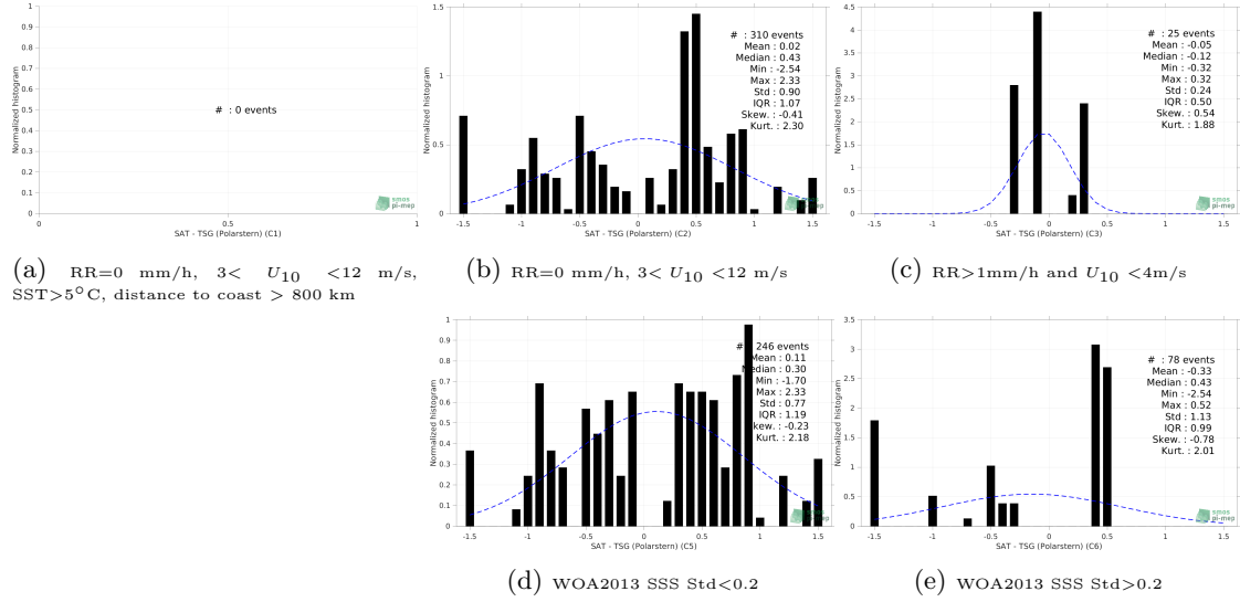
Figure 13: Normalized histogram of \Delta SSS (SMOS SSS L2Q v331 - With FLAG (CMEMS-CATDS-CPDC) - TSG (Polarstern)) for 5 different subdatasets corresponding to: RR=0 mm/h, 3 < U_{10} < 12 m/s, SST > 5°C, distance to coast > 800 km (a), RR=0 mm/h, 3 < U_{10} < 12 m/s (b), RR > 1mm/h and U_{10} < 4 m/s (c), WOA2013 SSS Std < 0.2 (d), WOA2013 SSS Std > 0.2 (e).
