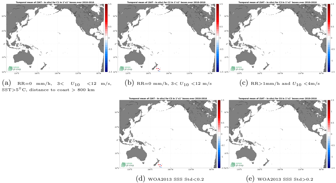
Figure 12: Temporal mean gridded over spatial boxes of size 1^{\circ}\times 1^{\circ} of \Delta\text{SSS} (SMOS SSS L2Q v331 - With FLAG (CMEMS-CATDS-CPDC) - TSG (Polarstern)) for 5 different subdatasets corresponding to:RR=0 mm/h, 3 < U_{10} < 12 m/s, SST >5^{\circ}\text{C} , distance to coast > 800 km (a), RR=0 mm/h, 3 < U_{10} < 12 m/s (b), RR >1 mm/h and U_{10} < 4 m/s (c), WOA2013 SSS Std <0.2 (d), WOA2013 SSS Std >0.2 (e).
