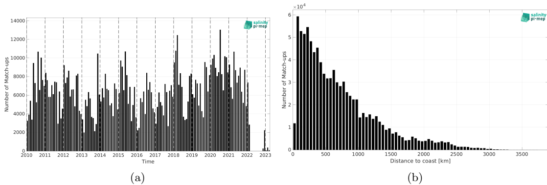
Figure 2: Number of match-ups between TSG (LEGOS-DM) and SMOS SSS L2Q v331 - With FLAG (CMEMS-CATDS-CPDC) SSS as a function of time (a) and as function of the distance to coast (b) over the Pacific Ocean Pi-MEP region and for the full satellite product period.
