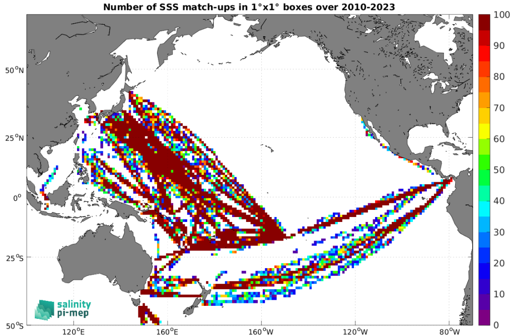
Figure 5: Number of SSS match-ups between TSG (LEGOS-DM) SSS and the SMOS SSS L2Q v331 - With FLAG (CMEMS-CATDS-CPDC) SSS product for the Pacific Ocean Pi-MEP region over 1^\circ \times 1^\circ boxes and for the full satellite product period.
