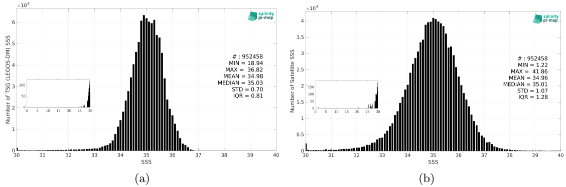
Figure 3: Histograms of SSS from TSG (LEGOS-DM) (a) and SMOS SSS L2Q v331 - With FLAG (CMEMS-CATDS-CPDC) (b) considering all match-up pairs per bins of 0.1 over the Pacific Ocean Pi-MEP region and for the full satellite product period.
