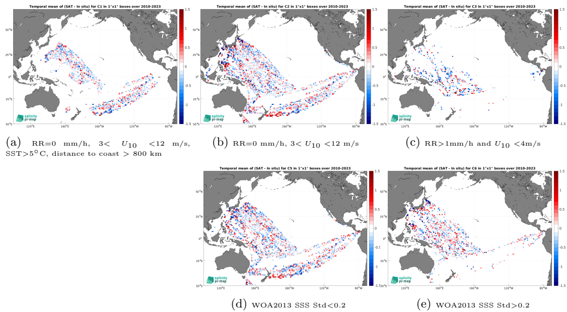
Figure 14: Temporal mean gridded over spatial boxes of size 1^\circ \times 1^\circ of \Delta SSS (SMOS SSS L2Q v331 - With FLAG (CMEMS-CATDS-CPDC) - TSG (LEGOS-DM)) for 5 different subdatasets corresponding to:RR=0 mm/h, 3 < U_{10} < 12 m/s, SST >5^\circ C, distance to coast > 800 km (a), RR=0 mm/h, 3 < U_{10} < 12 m/s (b), RR >1 mm/h and U_{10} < 4 m/s (c), WOA2013 SSS Std <0.2 (d), WOA2013 SSS Std >0.2 (e).
