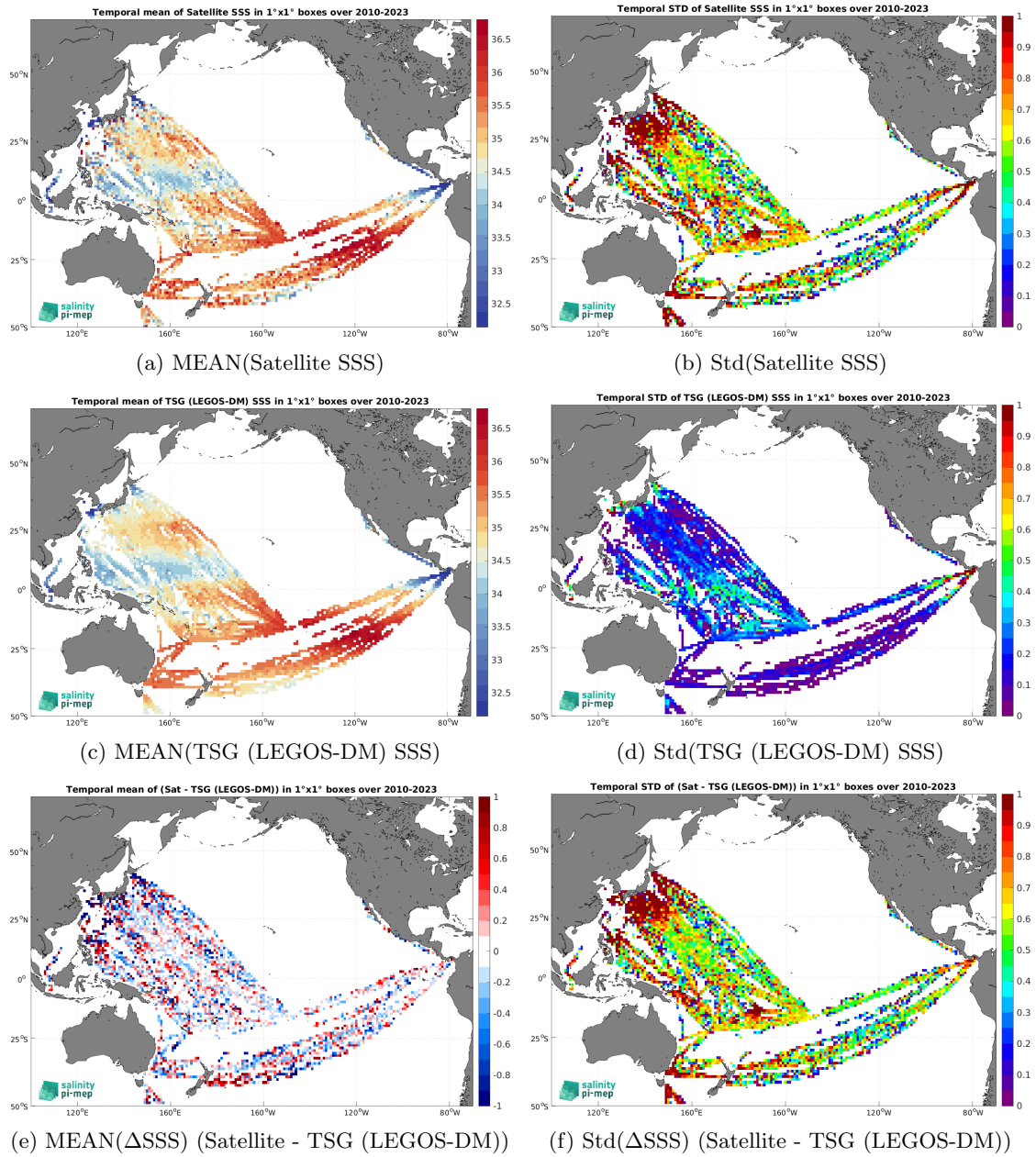
Figure 7: Temporal mean (left) and Std (right) of SSS from SMOS SSS L2Q v331 - With FLAG (CMEMS-CATDS-CPDC) (top), TSG (LEGOS-DM) (middle), and of \Delta SSS (Satellite - TSG (LEGOS-DM)). Only match-up pairs are used to generate these maps.
