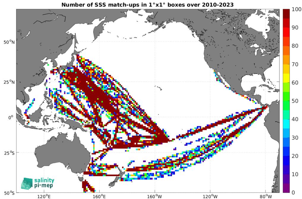
Figure 4: Number of SSS match-ups between TSG (LEGOS-DM) SSS and the SMOS SSS L2Q v331 - With FLAG (CMEMS-CATDS-CPDC) SSS product for the Pacific Ocean Pi-MEP region over 1^\circ \times 1^\circ boxes and for the full satellite product period.
