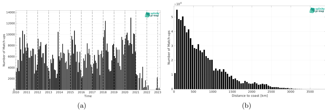
Figure 1: Number of match-ups between TSG (LEGOS-DM) and SMOS SSS L2Q v331 - With FLAG (CMEMS-CATDS-CPDC) SSS as a function of time (a) and as function of the distance to coast (b) over the Pacific Ocean Pi-MEP region and for the full satellite product period.
