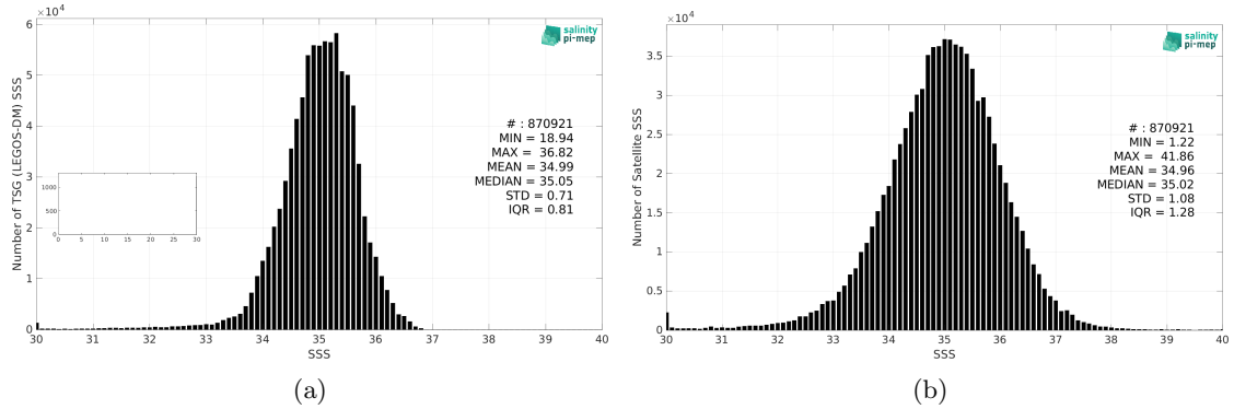
Figure 2: Histograms of SSS from TSG (LEGOS-DM) (a) and SMOS SSS L2Q v331 - With FLAG (CMEMS-CATDS-CPDC) (b) considering all match-up pairs per bins of 0.1 over the Pacific Ocean Pi-MEP region and for the full satellite product period.
