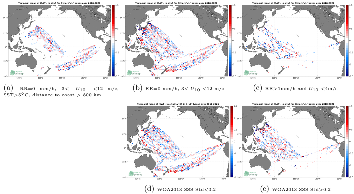
Figure 12: Temporal mean gridded over spatial boxes of size 1^\circ \times 1^\circ of \Delta SSS (SMOS SSS L2Q v331 - With FLAG (CMEMS-CATDS-CPDC) - TSG (LEGOS-DM)) for 5 different subdatasets corresponding to:RR=0 mm/h, 3 < U_{10} < 12 m/s, SST >5^\circ C, distance to coast > 800 km (a), RR=0 mm/h, 3 < U_{10} < 12 m/s (b), RR >1 mm/h and U_{10} < 4 m/s (c), WOA2013 SSS Std <0.2 (d), WOA2013 SSS Std >0.2 (e).
