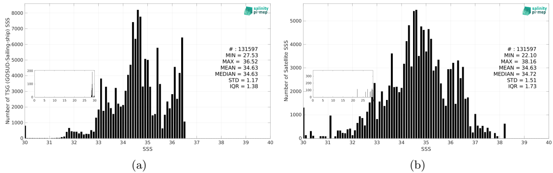
Figure 3: Histograms of SSS from TSG (GOSUD-Sailing-ship) (a) and SMOS SSS L2Q v331 - With FLAG (CMEMS-CATDS-CPDC) (b) considering all match-up pairs per bins of 0.1 over the Pacific Ocean Pi-MEP region and for the full satellite product period.
