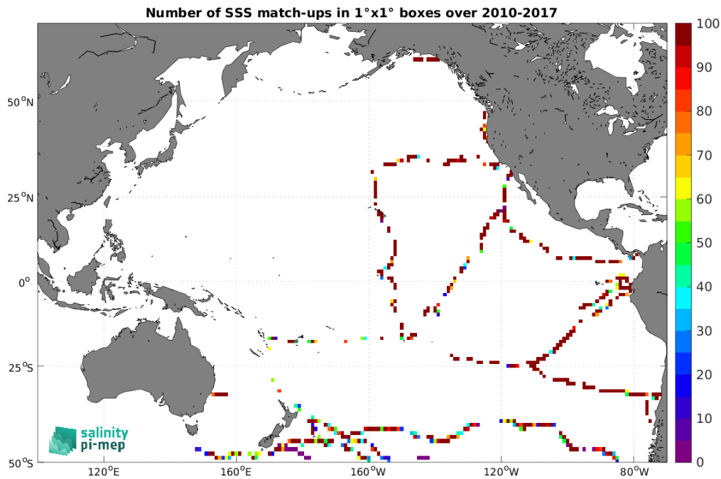
Figure 4: Number of SSS match-ups between TSG (GOSUD-Sailing-ship) SSS and the SMOS SSS L2Q v331 - With FLAG (CMEMS-CATDS-CPDC) SSS product for the Pacific Ocean Pi-MEP region over 1^\circ \times 1^\circ boxes and for the full satellite product period.
