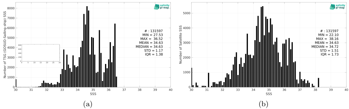
Figure 2: Histograms of SSS from TSG (GOSUD-Sailing-ship) (a) and SMOS SSS L2Q v331 - With FLAG (CMEMS-CATDS-CPDC) (b) considering all match-up pairs per bins of 0.1 over the Pacific Ocean Pi-MEP region and for the full satellite product period.
