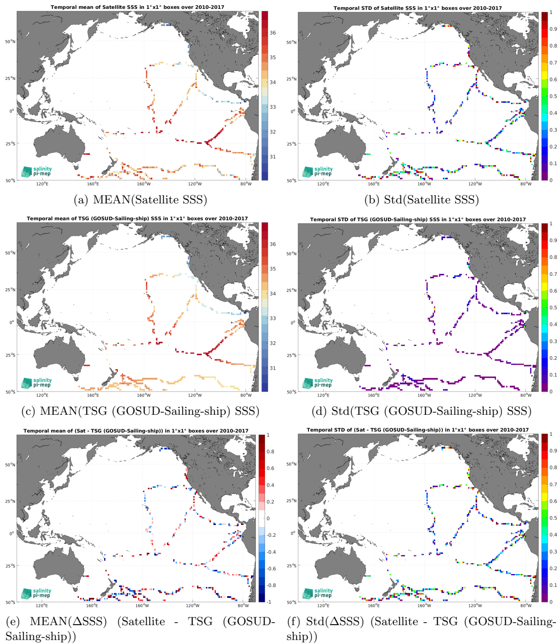
Figure 6: Temporal mean (left) and Std (right) of SSS from SMOS SSS L2Q v331 - With FLAG (CMEMS-CATDS-CPDC) (top), TSG (GOSUD-Sailing-ship) (middle), and of \Delta SSS (Satellite - TSG (GOSUD-Sailing-ship)). Only match-up pairs are used to generate these maps.
