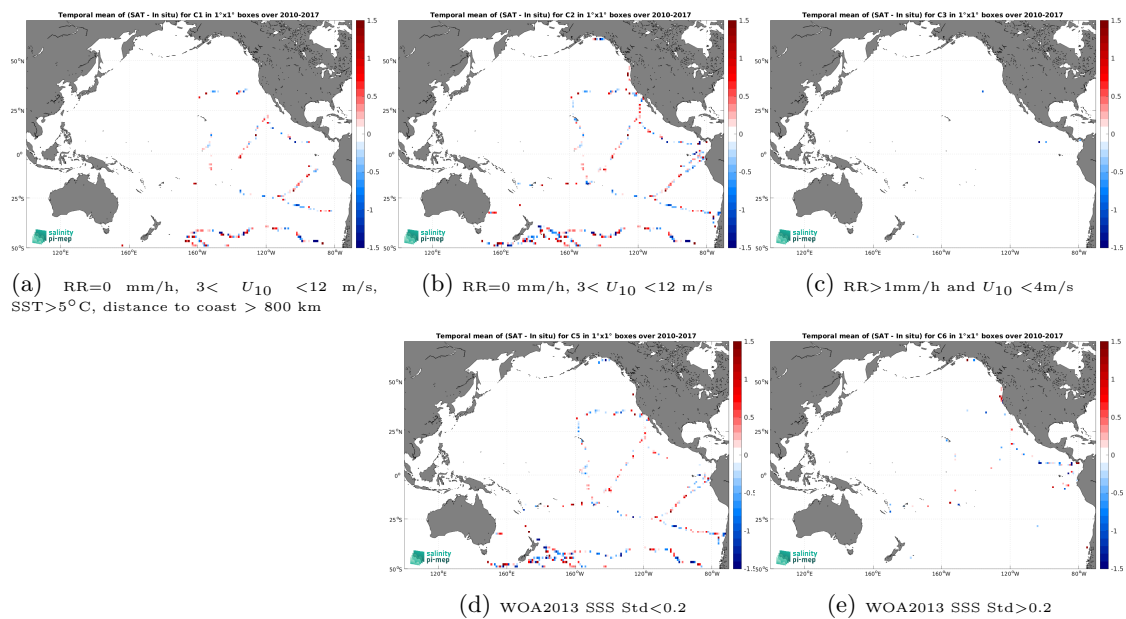
Figure 12: Temporal mean gridded over spatial boxes of size 1^\circ \times 1^\circ of \Delta\text{SSS} (SMOS SSS L2Q v331 - With FLAG (CMEMS-CATDS-CPDC) - TSG (GOSUD-Sailing-ship)) for 5 different subdatasets corresponding to:RR=0 mm/h, 3 < U_{10} < 12 m/s, SST >5^\circ\text{C} , distance to coast > 800 km (a), RR=0 mm/h, 3 < U_{10} < 12 m/s (b), RR >1 mm/h and U_{10} < 4 m/s (c), WOA2013 SSS Std <0.2 (d), WOA2013 SSS Std >0.2 (e).
