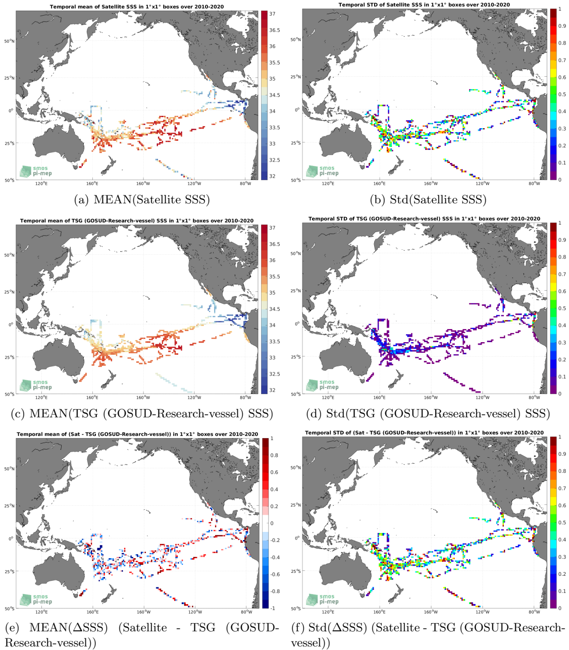
Figure 6: Temporal mean (left) and Std (right) of SSS from SMOS SSS L2Q v331 - With FLAG (CMEMS-CATDS-CPDC) (top), TSG (GOSUD-Research-vessel) (middle), and of \Delta SSS (Satellite - TSG (GOSUD-Research-vessel)). Only match-up pairs are used to generate these maps.
