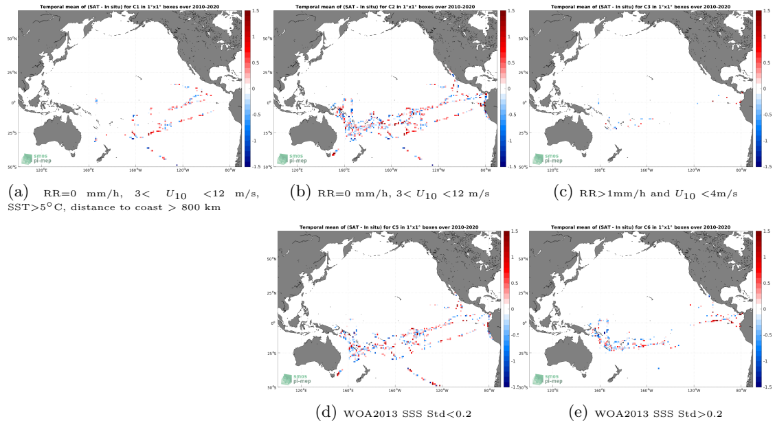
Figure 12: Temporal mean gridded over spatial boxes of size 1^\circ \times 1^\circ of \Delta SSS (SMOS SSS L2Q v331 - With FLAG (CMEMS-CATDS-CPDC) - TSG (GOSUD-Research-vessel)) for 5 different subdatasets corresponding to:RR=0 mm/h, 3 < U_{10} < 12 m/s, SST > 5^\circ\text{C} , distance to coast > 800 km (a), RR=0 mm/h, 3 < U_{10} < 12 m/s (b), RR > 1 mm/h and U_{10} < 4 m/s (c), WOA2013 SSS Std < 0.2 (d), WOA2013 SSS Std > 0.2 (e).
