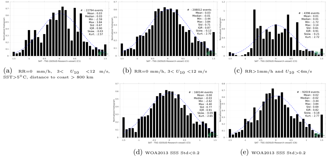
Figure 13: Normalized histogram of \Delta SSS (SMOS SSS L2Q v331 - With FLAG (CMEMS-CATDS-CPDC) - TSG (GOSUD-Research-vessel)) for 5 different subdatasets corresponding to: RR=0 mm/h, 3 < U_{10} < 12 m/s, SST > 5°C, distance to coast > 800 km (a), RR=0 mm/h, 3 < U_{10} < 12 m/s (b), RR > 1mm/h and U_{10} < 4 m/s (c), WOA2013 SSS Std < 0.2 (d), WOA2013 SSS Std > 0.2 (e).
