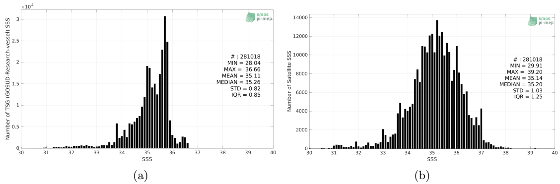
Figure 2: Histograms of SSS from TSG (GOSUD-Research-vessel) (a) and SMOS SSS L2Q v331 - With FLAG (CMEMS-CATDS-CPDC) (b) considering all match-up pairs per bins of 0.1 over the Pacific Ocean Pi-MEP region and for the full satellite product period.
