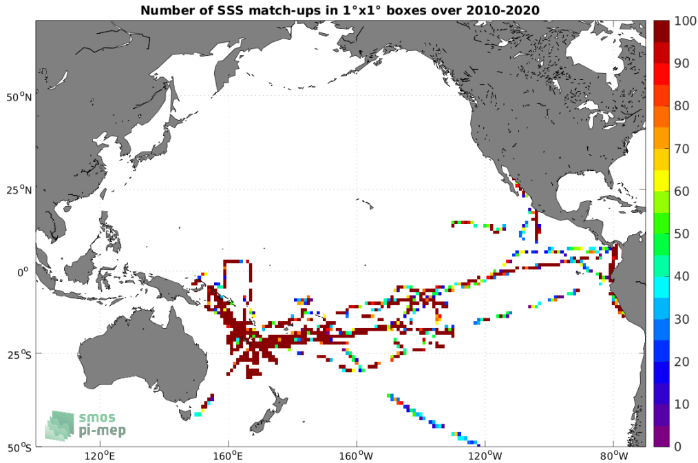
Figure 4: Number of SSS match-ups between TSG (GOSUD-Research-vessel) SSS and the SMOS SSS L2Q v331 - With FLAG (CMEMS-CATDS-CPDC) SSS product for the Pacific Ocean Pi-MEP region over 1^\circ \times 1^\circ boxes and for the full satellite product period.
