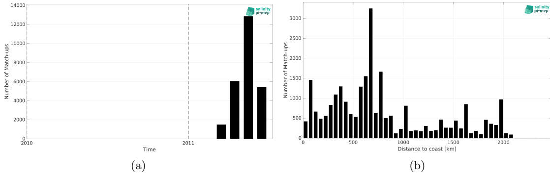
Figure 2: Number of match-ups between TSG (CSIC-UTM) and SMOS SSS L2Q v331 - With FLAG (CMEMS-CATDS-CPDC) SSS as a function of time (a) and as function of the distance to coast (b) over the Pacific Ocean Pi-MEP region and for the full satellite product period.
