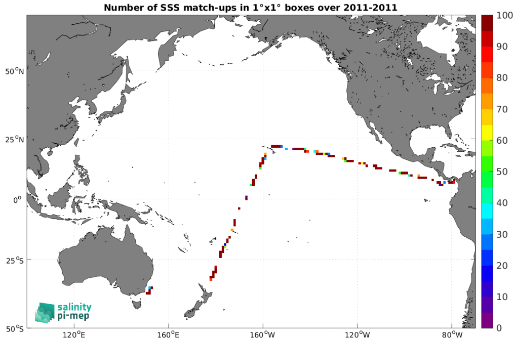
Figure 5: Number of SSS match-ups between TSG (CSIC-UTM) SSS and the SMOS SSS L2Q v331 - With FLAG (CMEMS-CATDS-CPDC) SSS product for the Pacific Ocean Pi-MEP region over 1^\circ \times 1^\circ boxes and for the full satellite product period.
