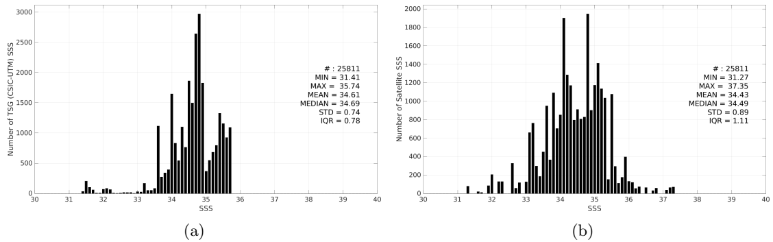
Figure 3: Histograms of SSS from TSG (CSIC-UTM) (a) and SMOS SSS L2Q v331 - With FLAG (CMEMS-CATDS-CPDC) (b) considering all match-up pairs per bins of 0.1 over the Pacific Ocean Pi-MEP region and for the full satellite product period.
