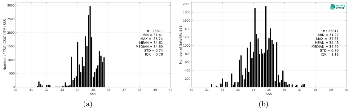
Figure 2: Histograms of SSS from TSG (CSIC-UTM) (a) and SMOS SSS L2Q v331 - With FLAG (CMEMS-CATDS-CPDC) (b) considering all match-up pairs per bins of 0.1 over the Pacific Ocean Pi-MEP region and for the full satellite product period.
