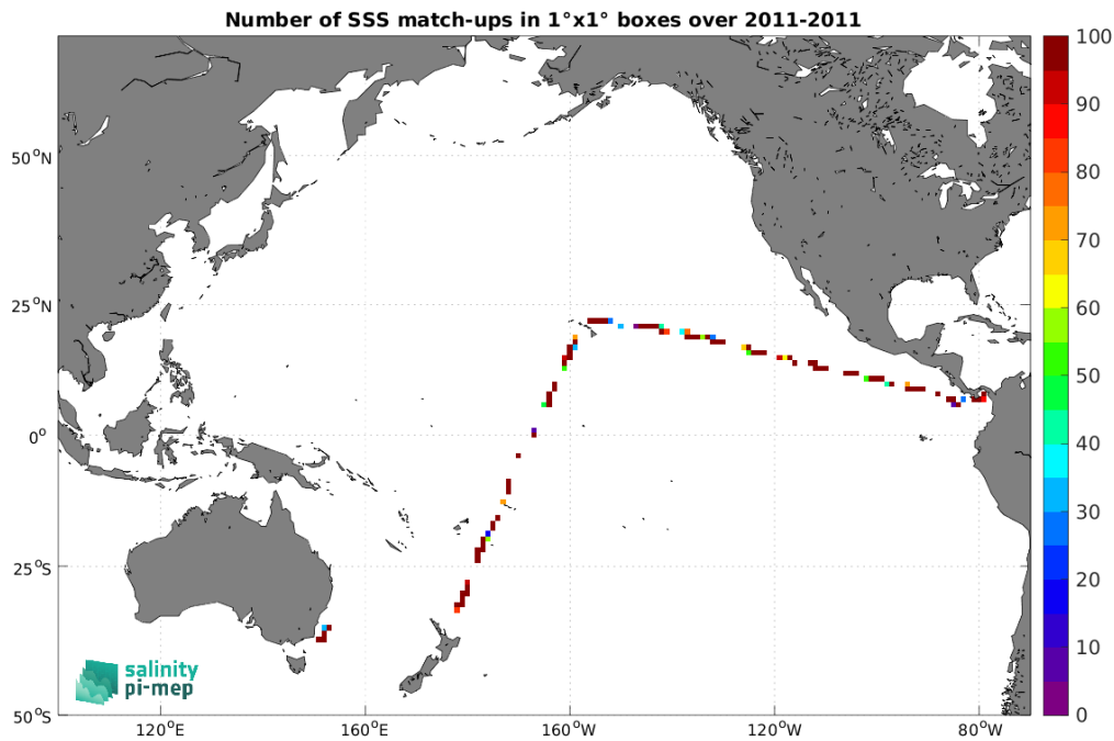
Figure 4: Number of SSS match-ups between TSG (CSIC-UTM) SSS and the SMOS SSS L2Q v331 - With FLAG (CMEMS-CATDS-CPDC) SSS product for the Pacific Ocean Pi-MEP region over 1^\circ \times 1^\circ boxes and for the full satellite product period.
