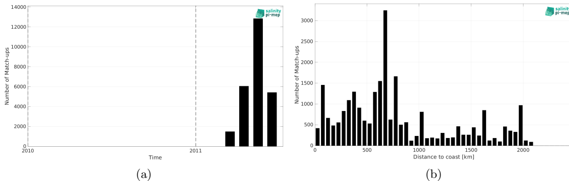
Figure 1: Number of match-ups between TSG (CSIC-UTM) and SMOS SSS L2Q v331 - With FLAG (CMEMS-CATDS-CPDC) SSS as a function of time (a) and as function of the distance to coast (b) over the Pacific Ocean Pi-MEP region and for the full satellite product period.
