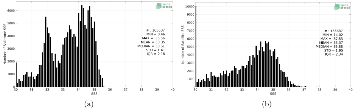
Figure 2: Histograms of SSS from Saildrone (a) and SMOS SSS L2Q v331 - With FLAG (CMEMS-CATDS-CPDC) (b) considering all match-up pairs per bins of 0.1 over the Pacific Ocean Pi-MEP region and for the full satellite product period.
