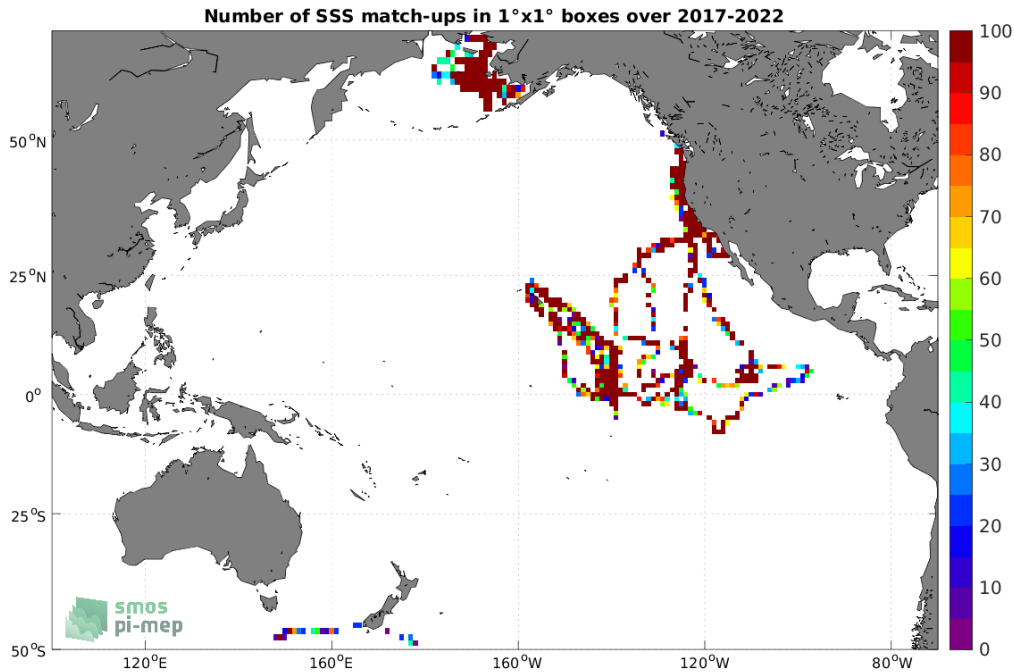
Figure 4: Number of SSS match-ups between Saildrone SSS and the SMOS SSS L2Q v331 - With FLAG (CMEMS-CATDS-CPDC) SSS product for the Pacific Ocean Pi-MEP region over 1^\circ \times 1^\circ boxes and for the full satellite product period.
