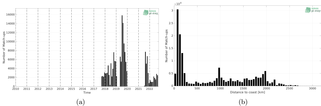
Figure 1: Number of match-ups between Saildrone and SMOS SSS L2Q v331 - With FLAG (CMEMS-CATDS-CPDC) SSS as a function of time (a) and as function of the distance to coast (b) over the Pacific Ocean Pi-MEP region and for the full satellite product period.
