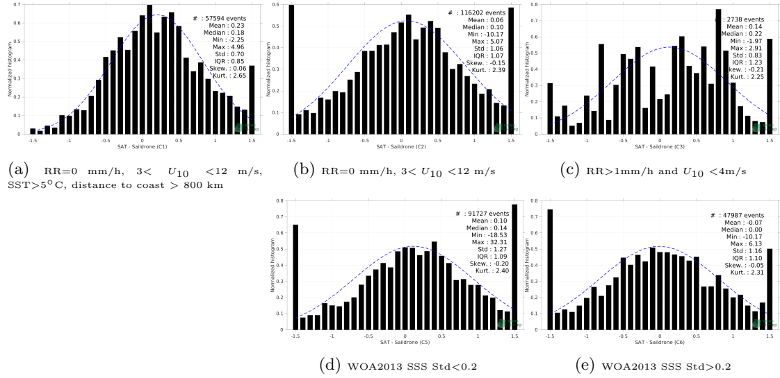
Figure 13: Normalized histogram of \Delta SSS (SMOS SSS L2Q v331 - With FLAG (CMEMS-CATDS-CPDC) - Sairdronne) for 5 different subdatasets corresponding to: RR=0 mm/h, 3 < U_{10} < 12 m/s, SST>5°C, distance to coast > 800 km (a), RR=0 mm/h, 3 < U_{10} < 12 m/s (b), RR>1mm/h and U_{10} < 4 m/s (c), WOA2013 SSS Std<0.2 (d), WOA2013 SSS Std>0.2 (e).
