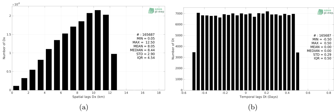
Figure 5: Histograms of the spatial (a) and temporal (b) lags between the location/time of the Saildrone measurement and the date of the corresponding SMOS SSS L2Q v331 - With FLAG (CMEMS-CATDS-CPDC) SSS pixel.
