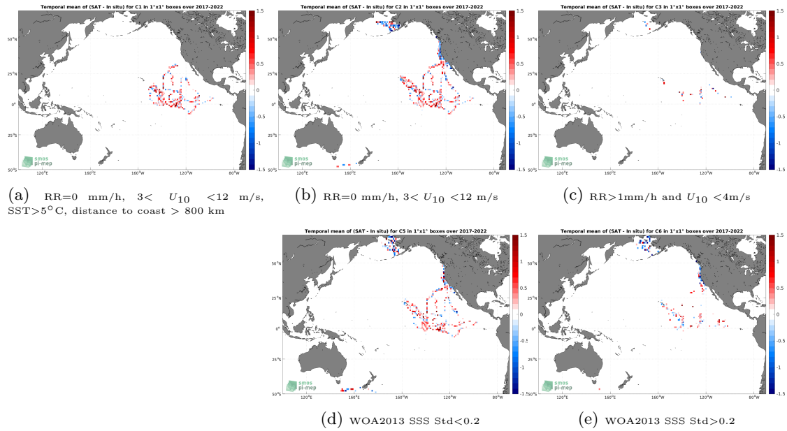
Figure 12: Temporal mean gridded over spatial boxes of size 1^\circ \times 1^\circ of \Delta SSS (SMOS SSS L2Q v331 - With FLAG (CMEMS-CATDS-CPDC) - Saildrone) for 5 different subdatasets corresponding to:RR=0 mm/h, 3 < U_{10} < 12 m/s, SST >5^\circ C, distance to coast > 800 km (a), RR=0 mm/h, 3 < U_{10} < 12 m/s (b), RR >1 mm/h and U_{10} < 4 m/s (c), WOA2013 SSS Std <0.2 (d), WOA2013 SSS Std >0.2 (e).
