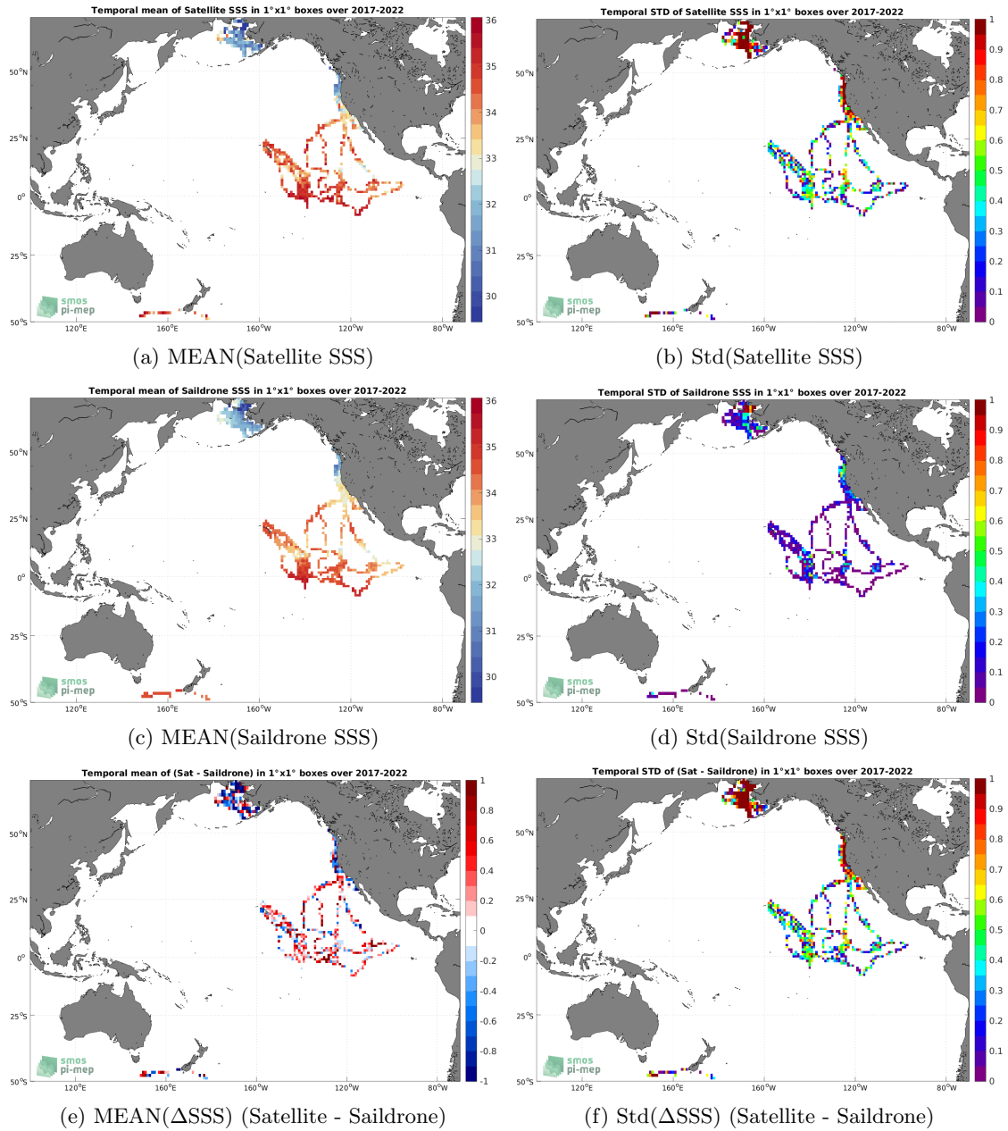
Figure 6: Temporal mean (left) and Std (right) of SSS from SMOS SSS L2Q v331 - With FLAG (CMEMS-CATDS-CPDC) (top), Saildrone (middle), and of \Delta SSS (Satellite - Saildrone). Only match-up pairs are used to generate these maps.
