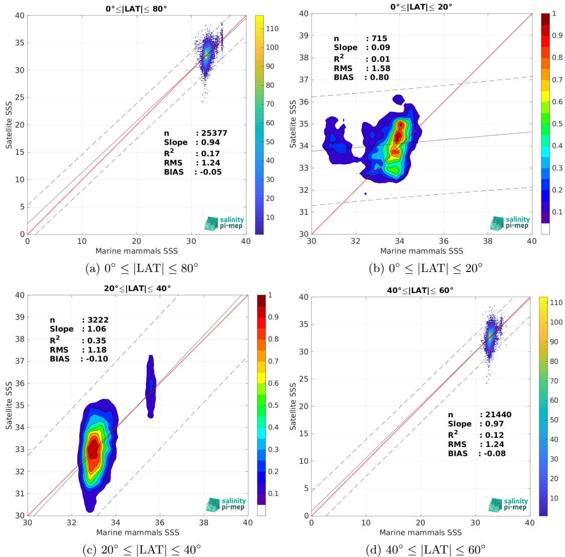
Figure 10: Contour maps of the concentration of SMOS SSS L2Q v331 - With FLAG (CMEMS-CATDS-CPDC) SSS (y-axis) versus Marine mammals SSS (x-axis) at match-up pairs for different latitude bands. For each plot, the red line shows x=y . The black thin and dashed lines indicate a linear fit through the data cloud and the \pm 95\% confidence levels, respectively. The number match-up pairs n , the slope and R^2 coefficient of the linear fit, the root mean square (RMS) and the mean bias between satellite and in situ data are indicated for each latitude band in each plots.
