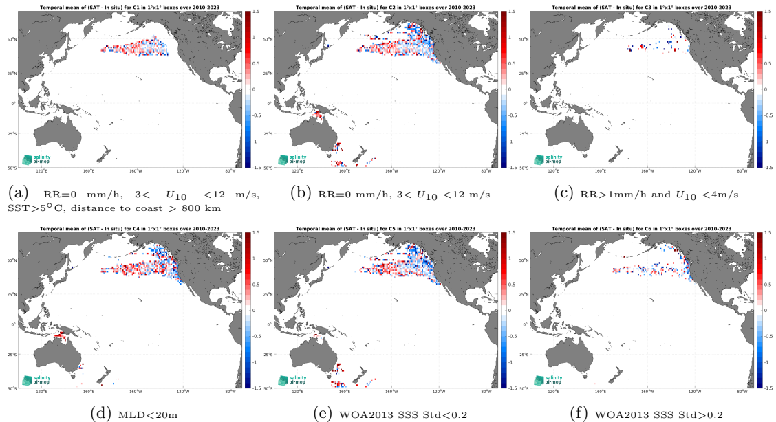
Figure 14: Temporal mean gridded over spatial boxes of size 1^\circ \times 1^\circ of \Delta SSS (SMOS SSS L2Q v331 - With FLAG (CMEMS-CATDS-CPDC) - Marine mammals) for 6 different subdatasets corresponding to: RR=0 mm/h, 3 < U_{10} < 12 m/s, SST > 5^\circ\text{C} , distance to coast > 800 km (a), RR=0 mm/h, 3 < U_{10} < 12 m/s (b), RR > 1 mm/h and U_{10} < 4 m/s (c),MLD < 20 m (d),WOA2013 SSS Std < 0.2 (e),WOA2013 SSS Std > 0.2 (f).
