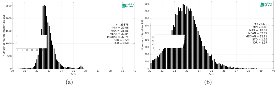
Figure 3: Histograms of SSS from Marine mammals (a) and SMOS SSS L2Q v331 - With FLAG (CMEMS-CATDS-CPDC) (b) considering all match-up pairs per bins of 0.1 over the Pacific Ocean Pi-MEP region and for the full satellite product period.
