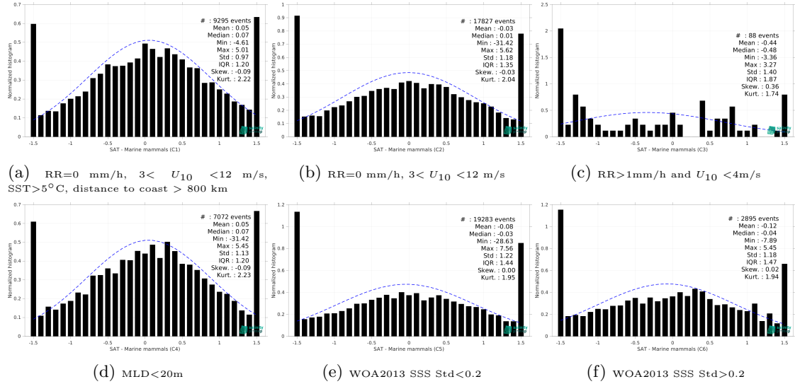
Figure 15: Normalized histogram of \Delta SSS (SMOS SSS L2Q v331 - With FLAG (CMEMS-CATDS-CPDC) - Marine mammals) for 6 different subdatasets corresponding to: RR=0 mm/h, 3 < U_{10} < 12 m/s, SST>5°C, distance to coast > 800 km (a), RR=0 mm/h, 3 < U_{10} < 12 m/s (b), RR>1mm/h and U_{10} < 4 m/s (c), MLD<20m (d), WOA2013 SSS Std<0.2 (e), WOA2013 SSS Std>0.2 (f).
