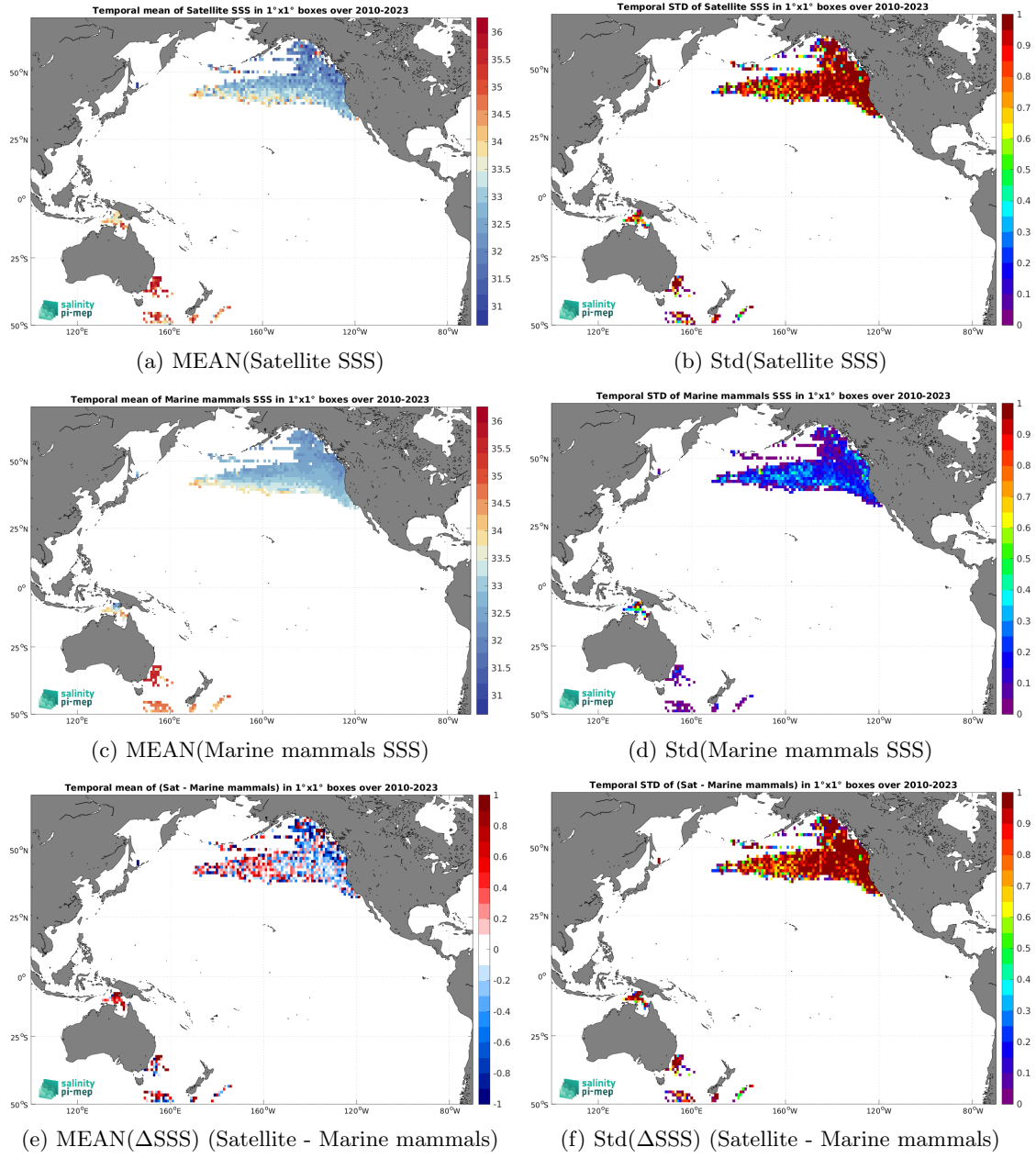
Figure 7: Temporal mean (left) and Std (right) of SSS from SMOS SSS L2Q v331 - With FLAG (CMEMS-CATDS-CPDC) (top), Marine mammals (middle), and of \Delta SSS (Satellite - Marine mammals). Only match-up pairs are used to generate these maps.
