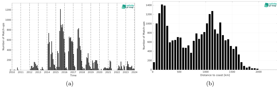
Figure 2: Number of match-ups between Marine mammals and SMOS SSS L2Q v331 - With FLAG (CMEMS-CATDS-CPDC) SSS as a function of time (a) and as function of the distance to coast (b) over the Pacific Ocean Pi-MEP region and for the full satellite product period.
