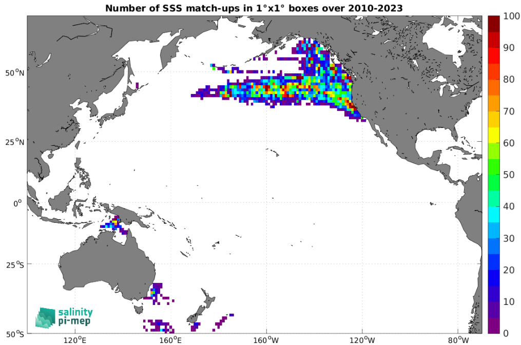
Figure 5: Number of SSS match-ups between Marine mammals SSS and the SMOS SSS L2Q v331 - With FLAG (CMEMS-CATDS-CPDC) SSS product for the Pacific Ocean Pi-MEP region over 1^\circ \times 1^\circ boxes and for the full satellite product period.
