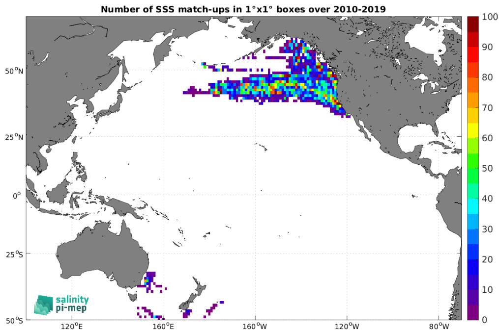
Figure 4: Number of SSS match-ups between Marine mammals SSS and the SMOS SSS L2Q v331 - With FLAG (CMEMS-CATDS-CPDC) SSS product for the Pacific Ocean Pi-MEP region over 1^\circ \times 1^\circ boxes and for the full satellite product period.
