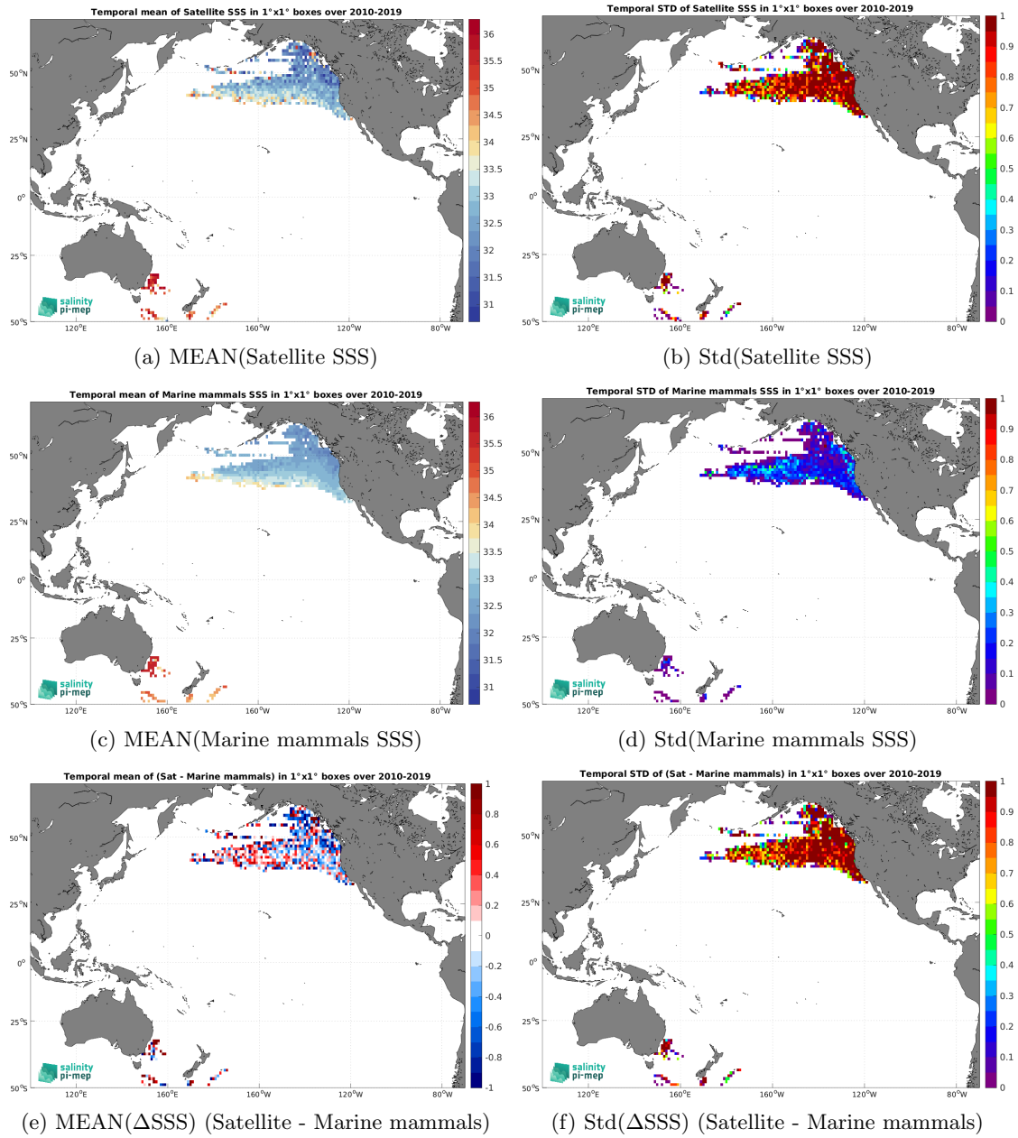
Figure 6: Temporal mean (left) and Std (right) of SSS from SMOS SSS L2Q v331 - With FLAG (CMEMS-CATDS-CPDC) (top), Marine mammals (middle), and of \Delta SSS (Satellite - Marine mammals). Only match-up pairs are used to generate these maps.
