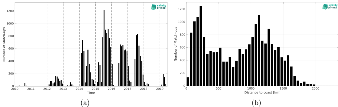
Figure 1: Number of match-ups between Marine mammals and SMOS SSS L2Q v331 - With FLAG (CMEMS-CATDS-CPDC) SSS as a function of time (a) and as function of the distance to coast (b) over the Pacific Ocean Pi-MEP region and for the full satellite product period.
