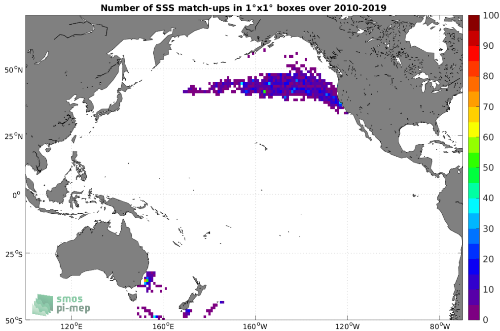
Figure 4: Number of SSS match-ups between Marine mammals SSS and the SMOS SSS L2Q v331 - With FLAG (CMEMS-CATDS-CPDC) SSS product for the Pacific Ocean Pi-MEP region over 1°×1° boxes and for the full satellite product period.
