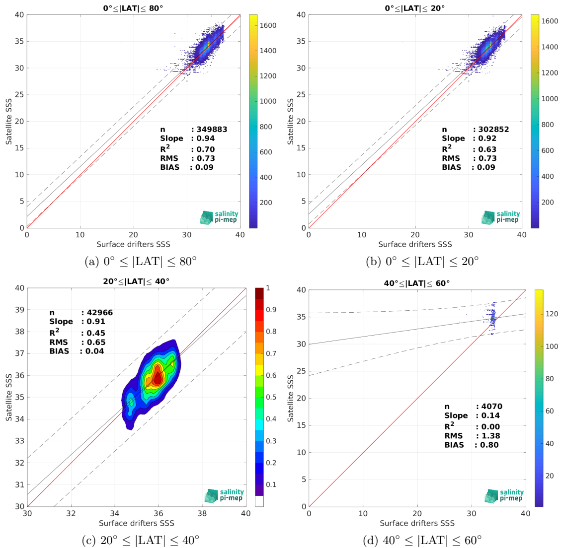
Figure 9: Contour maps of the concentration of SMOS SSS L2Q v331 - With FLAG (CMEMS-CATDS-CPDC) SSS (y-axis) versus Surface drifters SSS (x-axis) at match-up pairs for different latitude bands. For each plot, the red line shows x=y . The black thin and dashed lines indicate a linear fit through the data cloud and the \pm 95\% confidence levels, respectively. The number match-up pairs n , the slope and R^2 coefficient of the linear fit, the root mean square (RMS) and the mean bias between satellite and in situ data are indicated for each latitude band in each plots.
