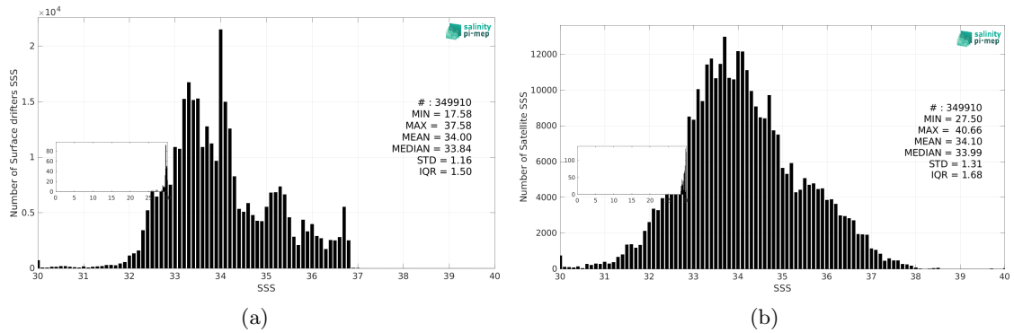
Figure 3: Histograms of SSS from Surface drifters (a) and SMOS SSS L2Q v331 - With FLAG (CMEMS-CATDS-CPDC) (b) considering all match-up pairs per bins of 0.1 over the Pacific Ocean Pi-MEP region and for the full satellite product period.
