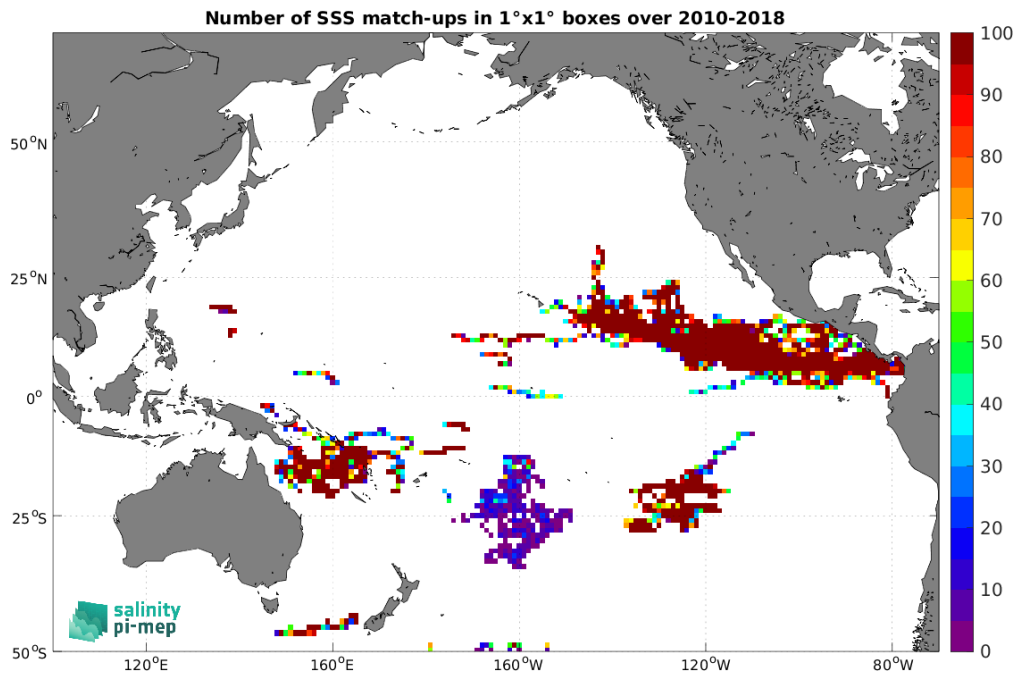
Figure 4: Number of SSS match-ups between Surface drifters SSS and the SMOS SSS L2Q v331 - With FLAG (CMEMS-CATDS-CPDC) SSS product for the Pacific Ocean Pi-MEP region over 1^\circ \times 1^\circ boxes and for the full satellite product period.
