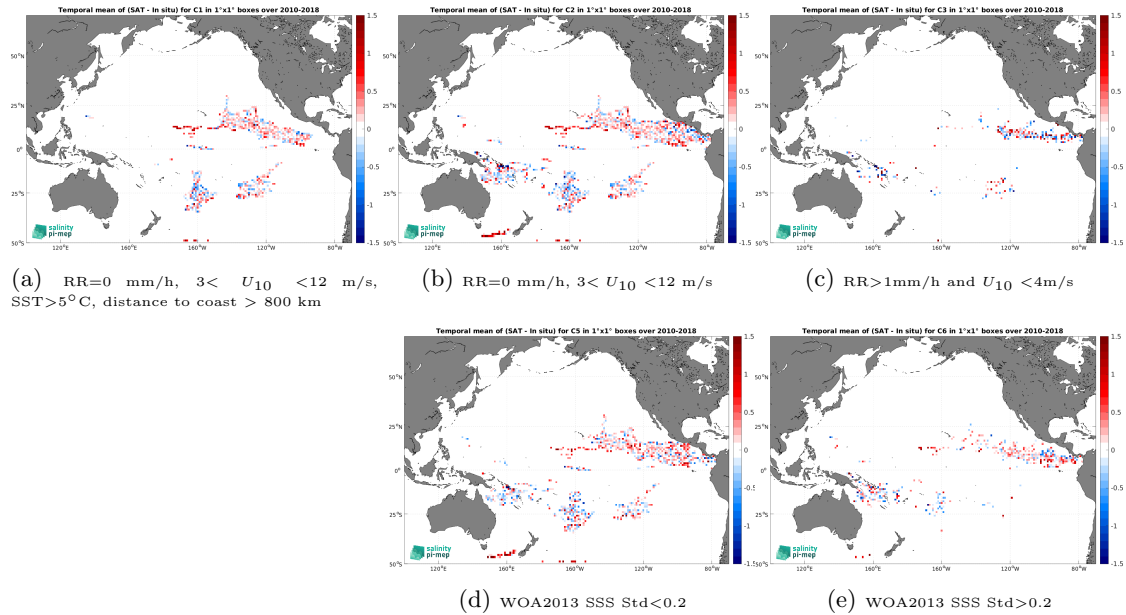
Figure 13: Temporal mean gridded over spatial boxes of size 1^\circ \times 1^\circ of \Delta SSS (SMOS SSS L2Q v331 - With FLAG (CMEMS-CATDS-CPDC) - Surface drifters) for 5 different subdatasets corresponding to:RR=0 mm/h, 3 < U_{10} < 12 m/s, SST >5^\circ C, distance to coast > 800 km (a), RR=0 mm/h, 3 < U_{10} < 12 m/s (b), RR >1 mm/h and U_{10} < 4 m/s (c), WOA2013 SSS Std <0.2 (d), WOA2013 SSS Std >0.2 (e).
