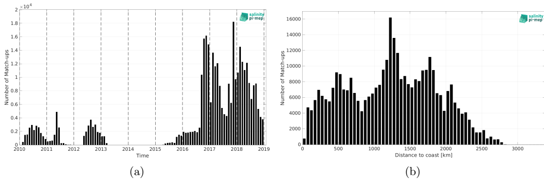
Figure 2: Number of match-ups between Surface drifters and SMOS SSS L2Q v331 - With FLAG (CMEMS-CATDS-CPDC) SSS as a function of time (a) and as function of the distance to coast (b) over the Pacific Ocean Pi-MEP region and for the full satellite product period.
