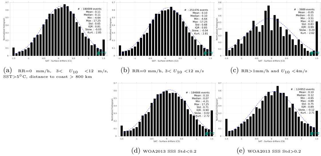
Figure 14: Normalized histogram of \Delta SSS (SMOS SSS L2Q v331 - With FLAG (CMEMS-CATDS-CPDC) - Surface drifters) for 5 different subdatasets corresponding to: RR=0 mm/h, 3 < U_{10} < 12 m/s, SST>5°C, distance to coast > 800 km (a), RR=0 mm/h, 3 < U_{10} < 12 m/s (b), RR>1mm/h and U_{10} < 4 m/s (c), WOA2013 SSS Std<0.2 (d), WOA2013 SSS Std>0.2 (e).
