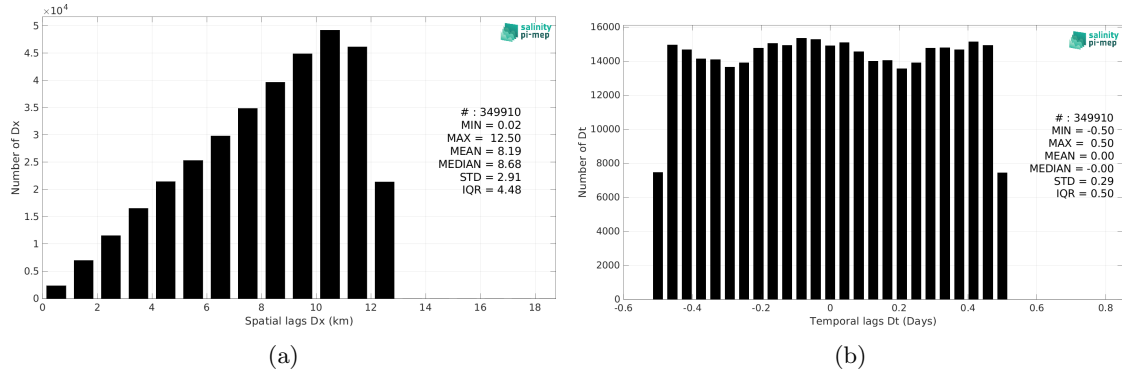
Figure 5: Histograms of the spatial (a) and temporal (b) lags between the location/time of the Surface drifters measurement and the date of the corresponding SMOS SSS L2Q v331 - With FLAG (CMEMS-CATDS-CPDC) SSS pixel.
