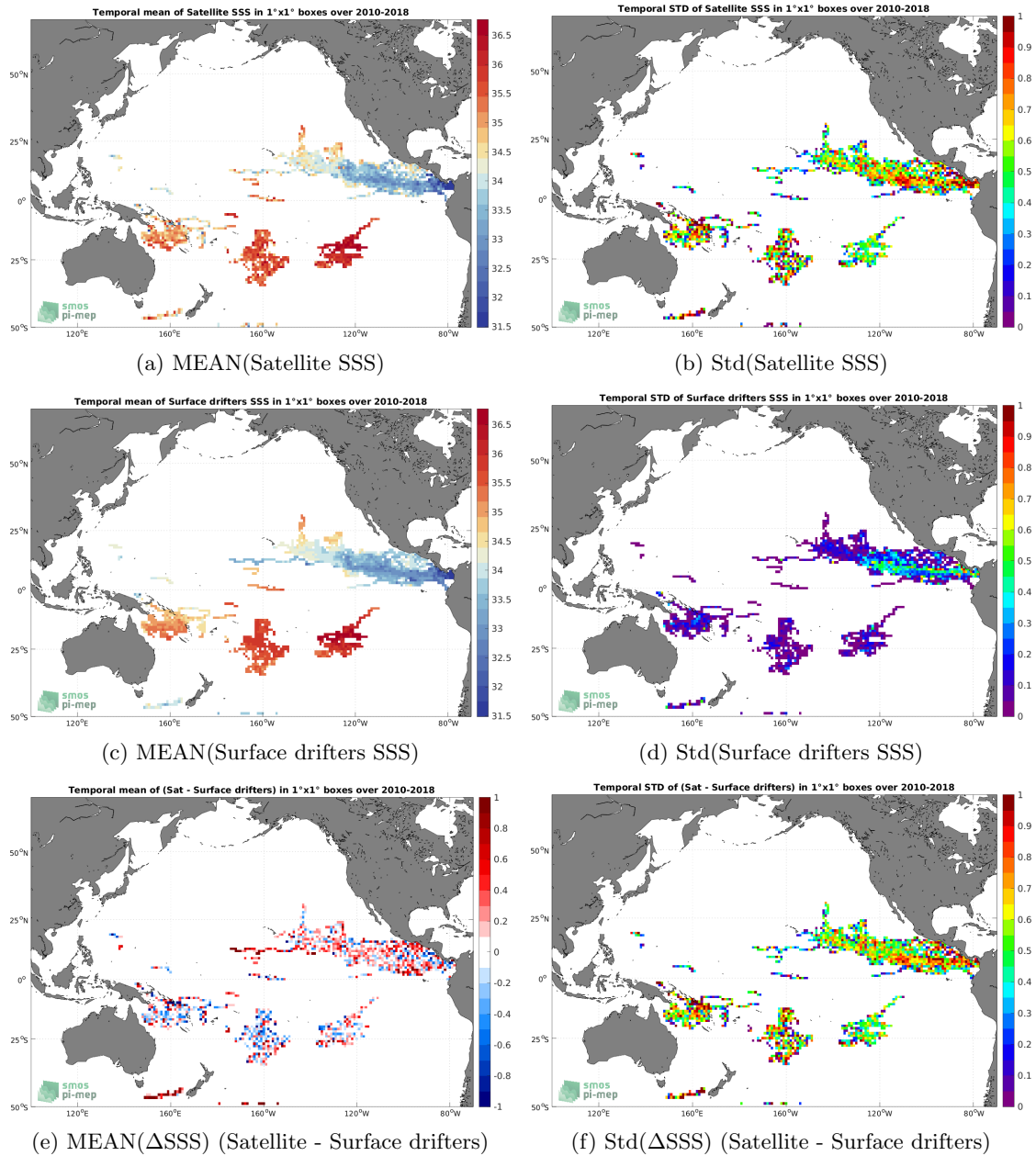
Figure 5: Temporal mean (left) and Std (right) of SSS from SMOS SSS L2Q v331 - With FLAG (CMEMS-CATDS-CPDC) (top), Surface drifters (middle), and of \Delta SSS (Satellite - Surface drifters). Only match-up pairs are used to generate these maps.
