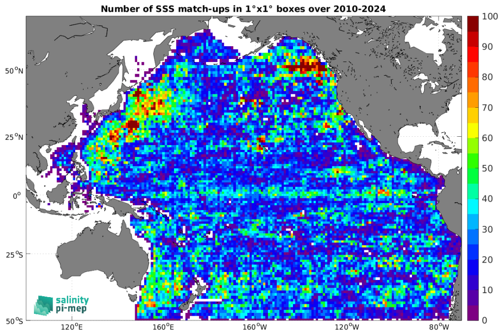
Figure 5: Number of SSS match-ups between Argo SSS and the SMOS SSS L2Q v331 - With FLAG (CMEMS-CATDS-CPDC) SSS product for the Pacific Ocean Pi-MEP region over 1^\circ \times 1^\circ boxes and for the full satellite product period.
