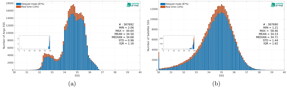
Figure 3: Histograms of SSS from Argo (a) and SMOS SSS L2Q v331 - With FLAG (CMEMS-CATDS-CPDC) (b) considering all match-up pairs per bins of 0.1 over the Pacific Ocean Pi-MEP region and for the full satellite product period.
