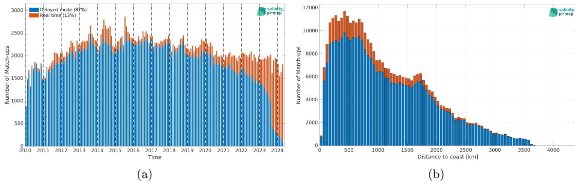
Figure 2: Number of match-ups between Argo and SMOS SSS L2Q v331 - With FLAG (CMEMS-CATDS-CPDC) SSS as a function of time (a) and as function of the distance to coast (b) over the Pacific Ocean Pi-MEP region and for the full satellite product period.
