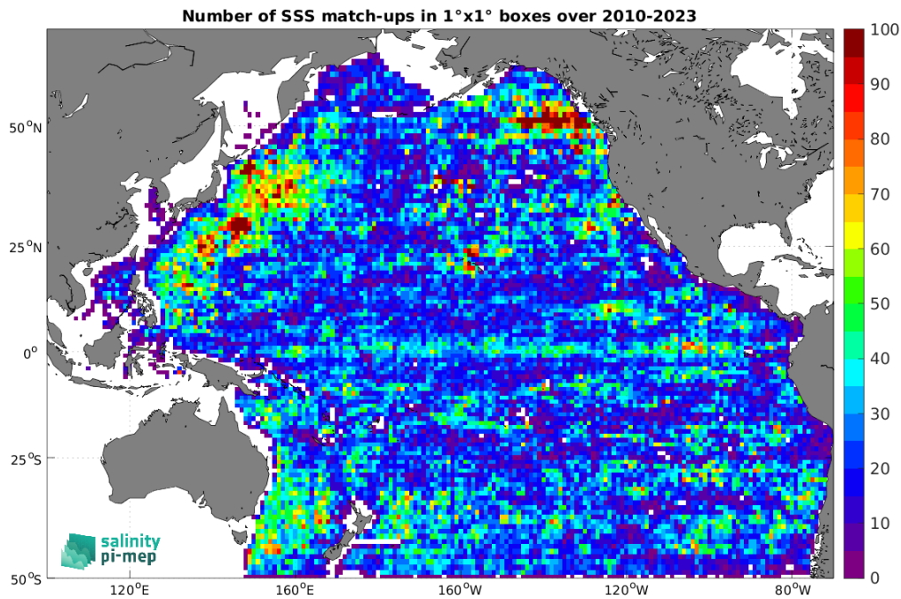
Figure 4: Number of SSS match-ups between Argo SSS and the SMOS SSS L2Q v331 - With FLAG (CMEMS-CATDS-CPDC) SSS product for the Pacific Ocean Pi-MEP region over 1^\circ \times 1^\circ boxes and for the full satellite product period.
