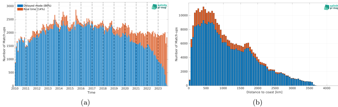
Figure 1: Number of match-ups between Argo and SMOS SSS L2Q v331 - With FLAG (CMEMS-CATDS-CPDC) SSS as a function of time (a) and as function of the distance to coast (b) over the Pacific Ocean Pi-MEP region and for the full satellite product period.
