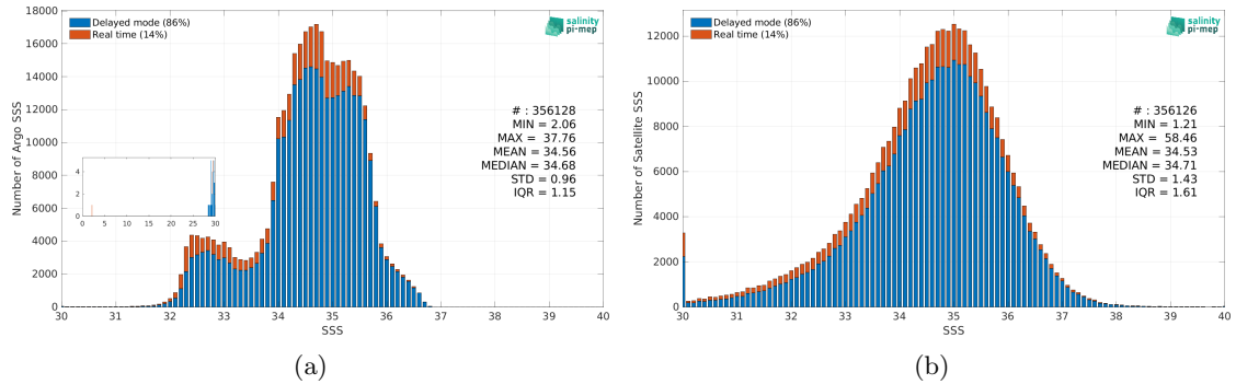
Figure 2: Histograms of SSS from Argo (a) and SMOS SSS L2Q v331 - With FLAG (CMEMS-CATDS-CPDC) (b) considering all match-up pairs per bins of 0.1 over the Pacific Ocean Pi-MEP region and for the full satellite product period.
