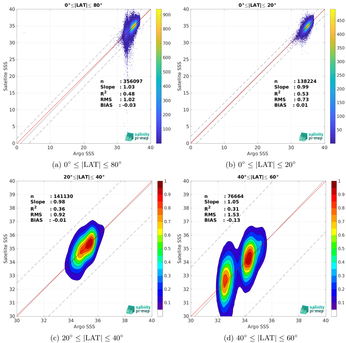
Figure 9: Contour maps of the concentration of SMOS SSS L2Q v331 - With FLAG (CMEMS-CATDS-CPDC) SSS ( y -axis) versus Argo SSS ( x -axis) at match-up pairs for different latitude bands. For each plot, the red line shows x=y . The black thin and dashed lines indicate a linear fit through the data cloud and the \pm 95\% confidence levels, respectively. The number match-up pairs n , the slope and R^2 coefficient of the linear fit, the root mean square (RMS) and the mean bias between satellite and in situ data are indicated for each latitude band in each plots.
