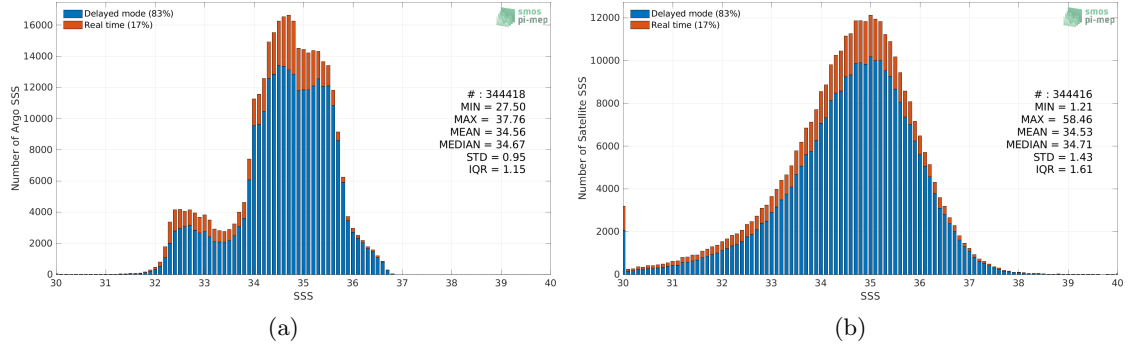
Figure 2: Histograms of SSS from Argo (a) and SMOS SSS L2Q v331 - With FLAG (CMEMS-CATDS-CPDC) (b) considering all match-up pairs per bins of 0.1 over the Pacific Ocean Pi-MEP region and for the full satellite product period.
