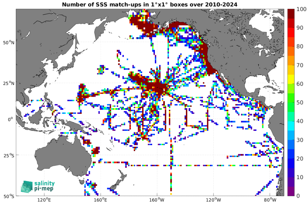
Figure 5: Number of SSS match-ups between TSG (SAMOS) SSS and the SMOS SSS L2Q v331 - No FLAG (CMEMS-CATDS-CPDC) SSS product for the Pacific Ocean Pi-MEP region over 1^\circ \times 1^\circ boxes and for the full satellite product period.
