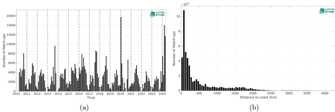
Figure 2: Number of match-ups between TSG (SAMOS) and SMOS SSS L2Q v331 - No FLAG (CMEMS-CATDS-CPDC) SSS as a function of time (a) and as function of the distance to coast (b) over the Pacific Ocean Pi-MEP region and for the full satellite product period.
