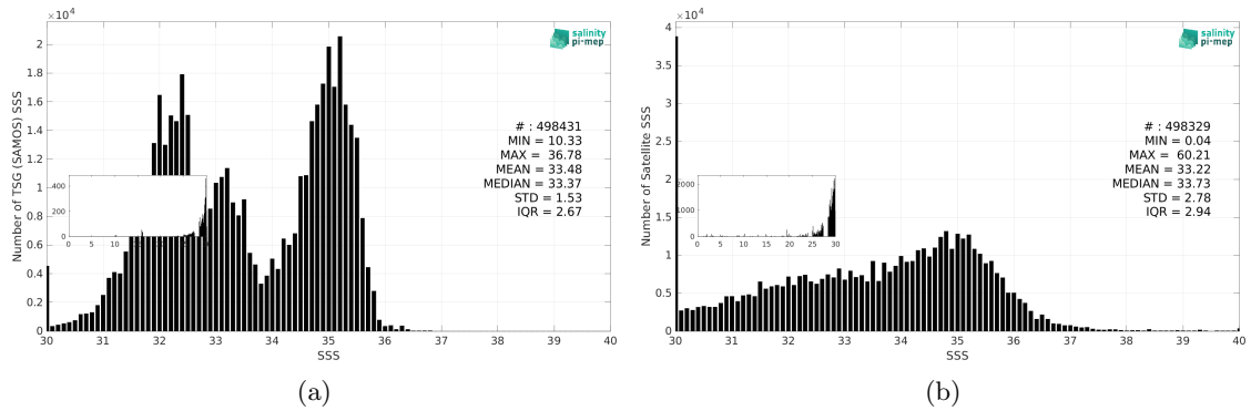
Figure 3: Histograms of SSS from TSG (SAMOS) (a) and SMOS SSS L2Q v331 - No FLAG (CMEMS-CATDS-CPDC) (b) considering all match-up pairs per bins of 0.1 over the Pacific Ocean Pi-MEP region and for the full satellite product period.
