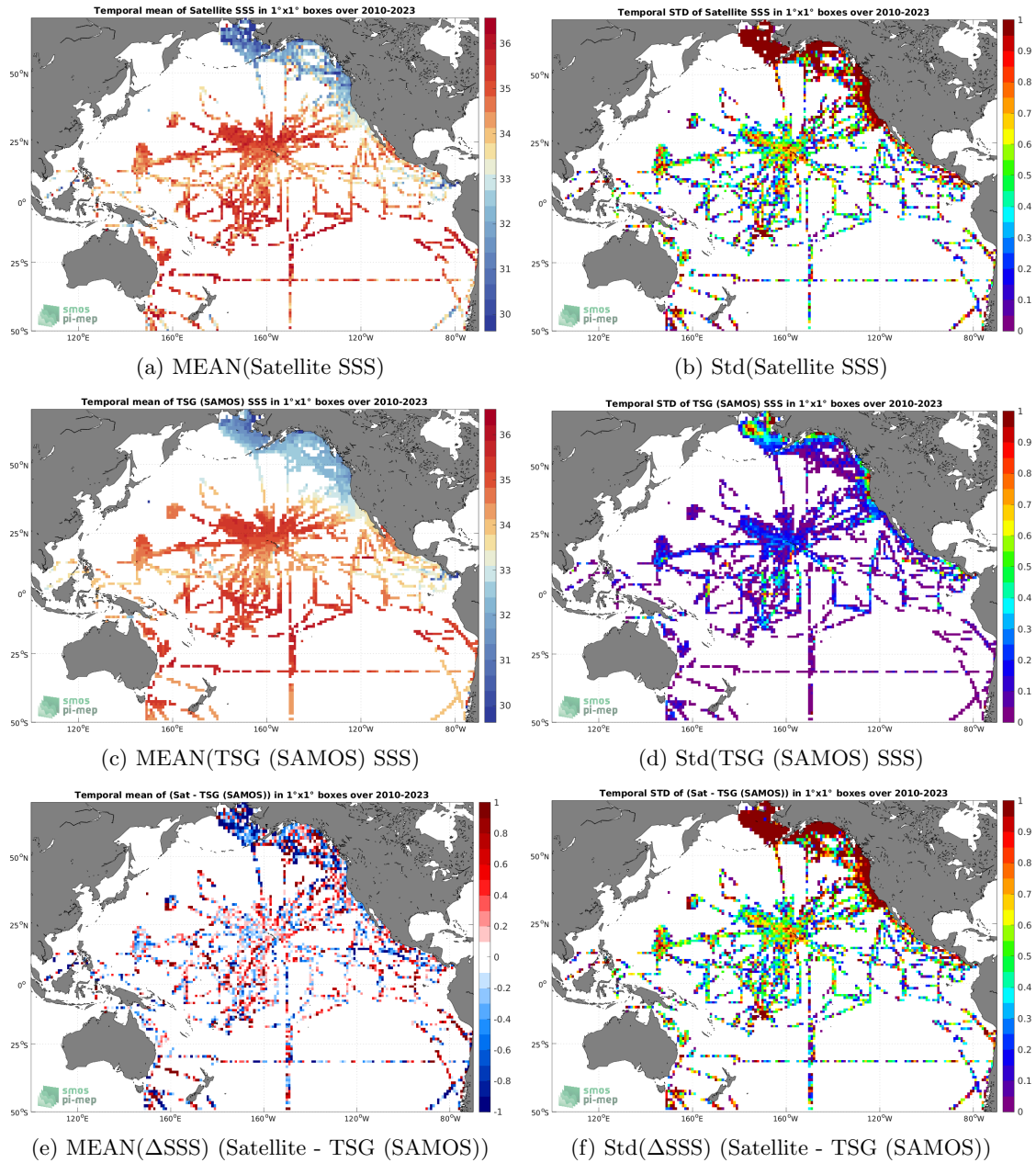
Figure 6: Temporal mean (left) and Std (right) of SSS from SMOS SSS L2Q v331 - No FLAG (CMEMS-CATDS-CPDC) (top), TSG (SAMOS) (middle), and of \Delta SSS (Satellite - TSG (SAMOS)). Only match-up pairs are used to generate these maps.
