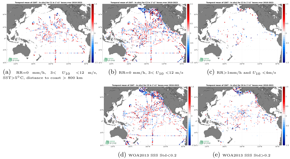
Figure 12: Temporal mean gridded over spatial boxes of size 1^\circ \times 1^\circ of \Delta SSS (SMOS SSS L2Q v331 - No FLAG (CMEMS-CATDS-CPDC) - TSG (SAMOS)) for 5 different subdatasets corresponding to:RR=0 mm/h, 3 < U_{10} < 12 m/s, SST >5^\circ C, distance to coast > 800 km (a), RR=0 mm/h, 3 < U_{10} < 12 m/s (b), RR >1 mm/h and U_{10} < 4 m/s (c), WOA2013 SSS Std <0.2 (d), WOA2013 SSS Std >0.2 (e).
