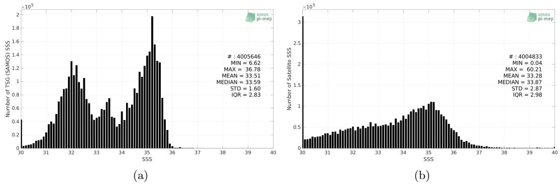
Figure 2: Histograms of SSS from TSG (SAMOS) (a) and SMOS SSS L2Q v331 - No FLAG (CMEMS-CATDS-CPDC) (b) considering all match-up pairs per bins of 0.1 over the Pacific Ocean Pi-MEP region and for the full satellite product period.
