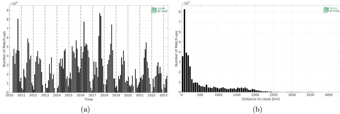
Figure 1: Number of match-ups between TSG (SAMOS) and SMOS SSS L2Q v331 - No FLAG (CMEMS-CATDS-CPDC) SSS as a function of time (a) and as function of the distance to coast (b) over the Pacific Ocean Pi-MEP region and for the full satellite product period.
