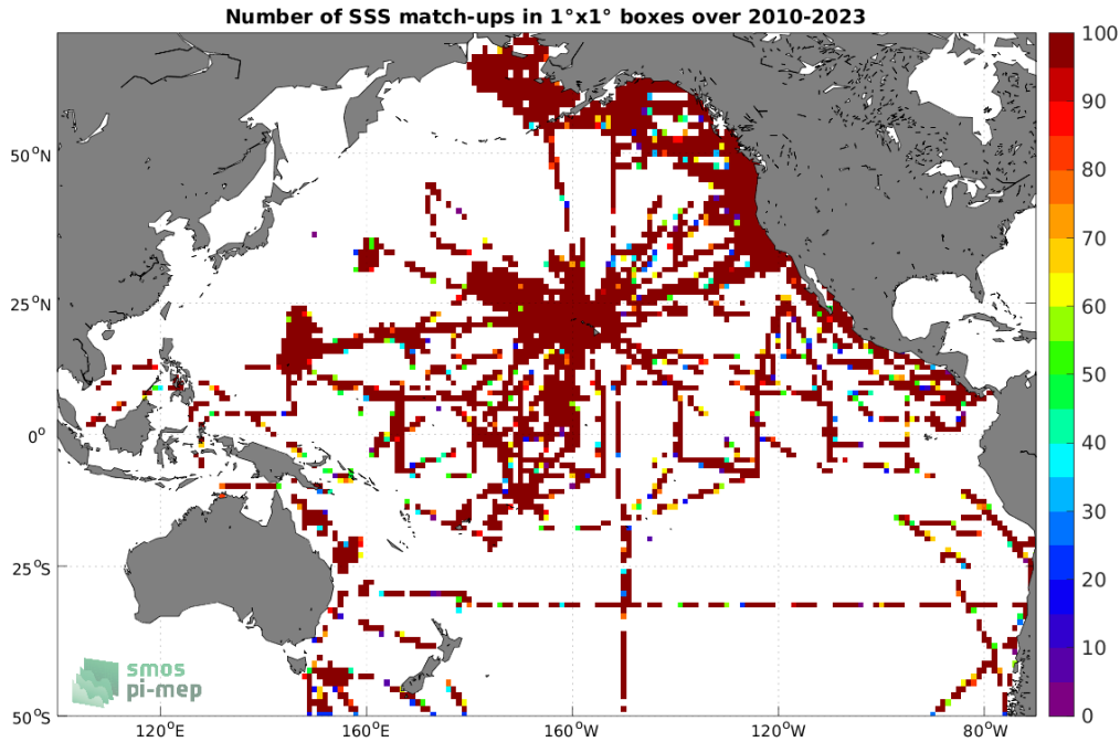
Figure 4: Number of SSS match-ups between TSG (SAMOS) SSS and the SMOS SSS L2Q v331 - No FLAG (CMEMS-CATDS-CPDC) SSS product for the Pacific Ocean Pi-MEP region over 1^\circ \times 1^\circ boxes and for the full satellite product period.
