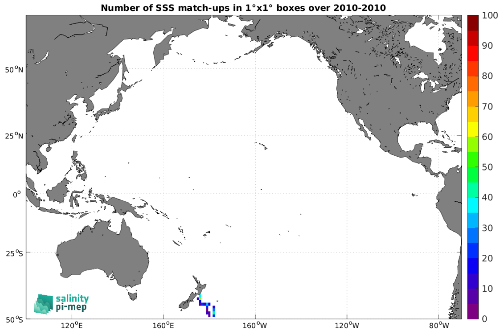
Figure 5: Number of SSS match-ups between TSG (Polarstern) SSS and the SMOS SSS L2Q v331 - No FLAG (CMEMS-CATDS-CPDC) SSS product for the Pacific Ocean Pi-MEP region over 1^\circ \times 1^\circ boxes and for the full satellite product period.
