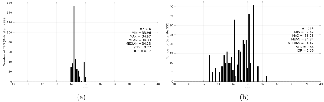
Figure 3: Histograms of SSS from TSG (Polarstern) (a) and SMOS SSS L2Q v331 - No FLAG (CMEMS-CATDS-CPDC) (b) considering all match-up pairs per bins of 0.1 over the Pacific Ocean Pi-MEP region and for the full satellite product period.
