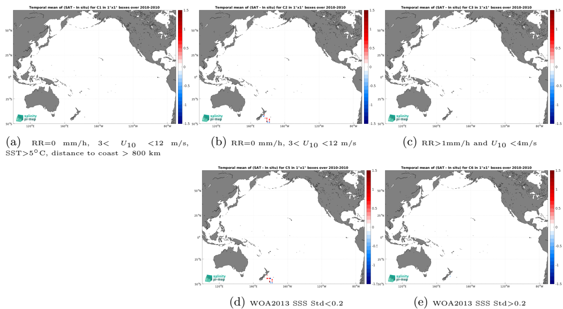
Figure 14: Temporal mean gridded over spatial boxes of size 1^\circ \times 1^\circ of \Delta SSS (SMOS SSS L2Q v331 - No FLAG (CMEMS-CATDS-CPDC) - TSG (Polarstern)) for 5 different subdatasets corresponding to:RR=0 mm/h, 3 < U_{10} < 12 m/s, SST >5^\circ C, distance to coast > 800 km (a), RR=0 mm/h, 3 < U_{10} < 12 m/s (b), RR >1 mm/h and U_{10} < 4 m/s (c), WOA2013 SSS Std <0.2 (d), WOA2013 SSS Std >0.2 (e).
