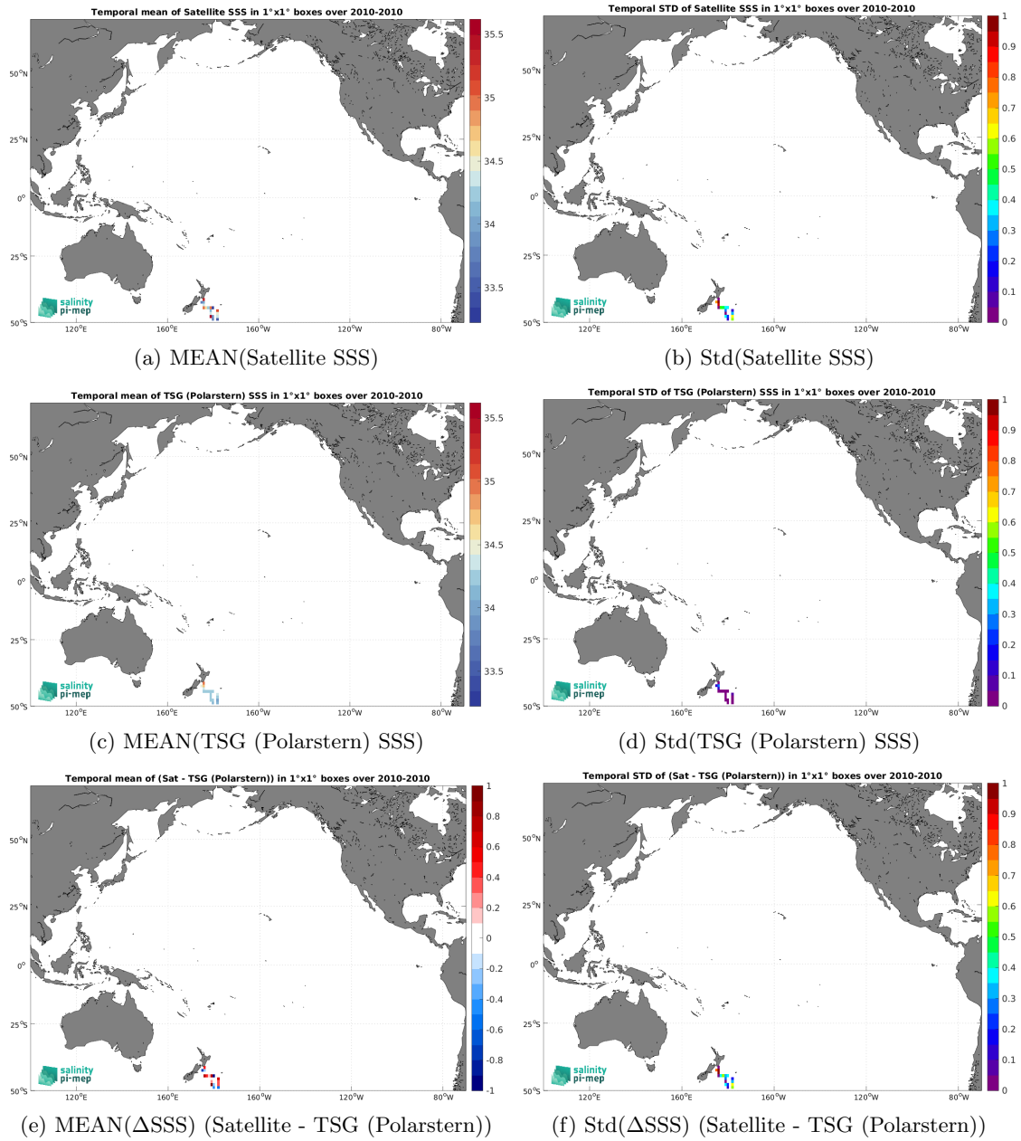
Figure 7: Temporal mean (left) and Std (right) of SSS from SMOS SSS L2Q v331 - No FLAG (CMEMS-CATDS-CPDC) (top), TSG (Polarstern) (middle), and of \Delta SSS (Satellite - TSG (Polarstern)). Only match-up pairs are used to generate these maps.
