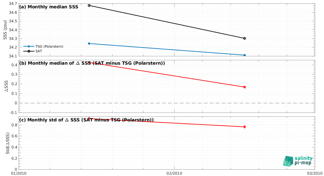
Figure 8: Time series of the monthly median SSS (top), median of \Delta\text{SSS} (Satellite - TSG (Polarstern)) and Std of \Delta\text{SSS} (Satellite - TSG (Polarstern)) over the Pacific Ocean Pi-MEP region considering all match-ups collected by the Pi-MEP.
