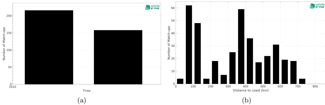
Figure 2: Number of match-ups between TSG (Polarstern) and SMOS SSS L2Q v331 - No FLAG (CMEMS-CATDS-CPDC) SSS as a function of time (a) and as function of the distance to coast (b) over the Pacific Ocean Pi-MEP region and for the full satellite product period.
