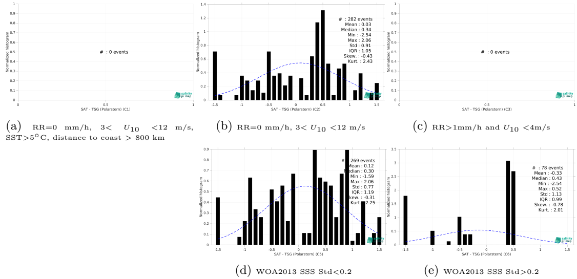
Figure 15: Normalized histogram of \Delta SSS (SMOS SSS L2Q v331 - No FLAG (CMEMS-CATDS-CPDC) - TSG (Polarstern)) for 5 different subdatasets corresponding to: RR=0 mm/h, 3 < U_{10} < 12 m/s, SST > 5°C, distance to coast > 800 km (a), RR=0 mm/h, 3 < U_{10} < 12 m/s (b), RR > 1mm/h and U_{10} < 4 m/s (c), WOA2013 SSS Std < 0.2 (d), WOA2013 SSS Std > 0.2 (e).
