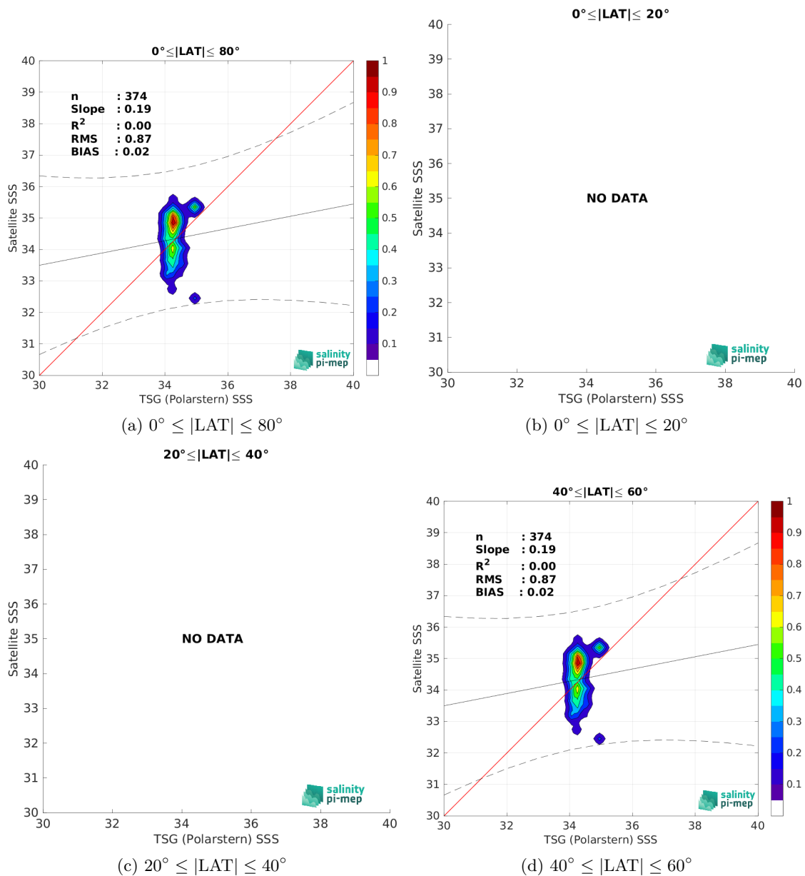
Figure 10: Contour maps of the concentration of SMOS SSS L2Q v331 - No FLAG (CMEMS-CATDS-CPDC) SSS (y-axis) versus TSG (Polarstern) SSS (x-axis) at match-up pairs for different latitude bands. For each plot, the red line shows x=y . The black thin and dashed lines indicate a linear fit through the data cloud and the \pm 95\% confidence levels, respectively. The number match-up pairs n , the slope and R^2 coefficient of the linear fit, the root mean square (RMS) and the mean bias between satellite and in situ data are indicated for each latitude band in each plots.
