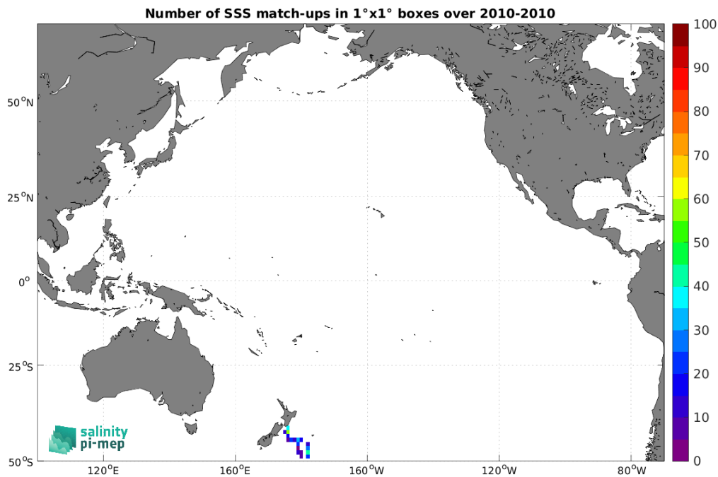
Figure 4: Number of SSS match-ups between TSG (Polarstern) SSS and the SMOS SSS L2Q v331 - No FLAG (CMEMS-CATDS-CPDC) SSS product for the Pacific Ocean Pi-MEP region over 1^\circ \times 1^\circ boxes and for the full satellite product period.
