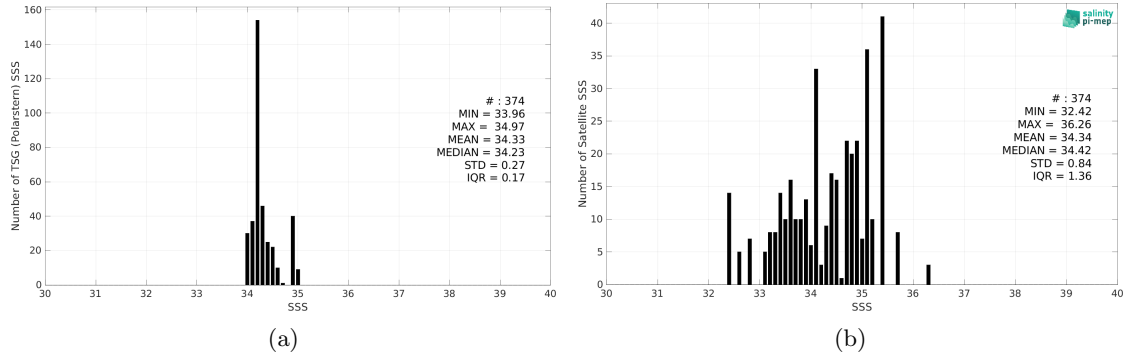
Figure 2: Histograms of SSS from TSG (Polarstern) (a) and SMOS SSS L2Q v331 - No FLAG (CMEMS-CATDS-CPDC) (b) considering all match-up pairs per bins of 0.1 over the Pacific Ocean Pi-MEP region and for the full satellite product period.
