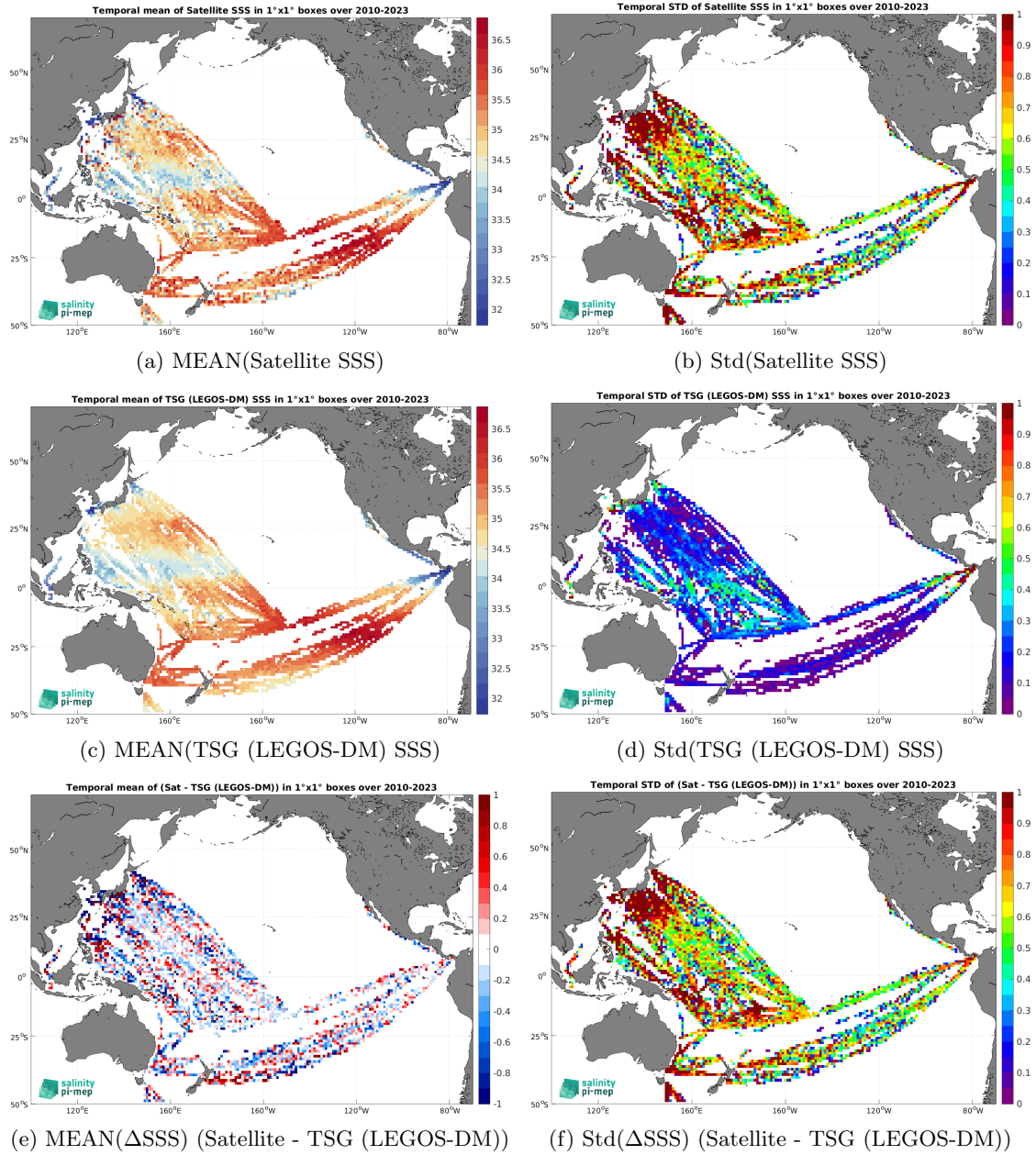
Figure 7: Temporal mean (left) and Std (right) of SSS from SMOS SSS L2Q v331 - No FLAG (CMEMS-CATDS-CPDC) (top), TSG (LEGOS-DM) (middle), and of \Delta SSS (Satellite - TSG (LEGOS-DM)). Only match-up pairs are used to generate these maps.
