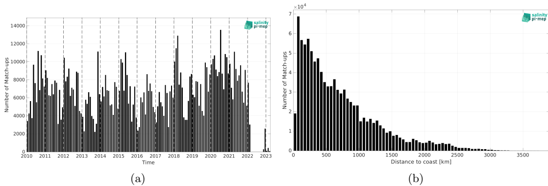
Figure 2: Number of match-ups between TSG (LEGOS-DM) and SMOS SSS L2Q v331 - No FLAG (CMEMS-CATDS-CPDC) SSS as a function of time (a) and as function of the distance to coast (b) over the Pacific Ocean Pi-MEP region and for the full satellite product period.
