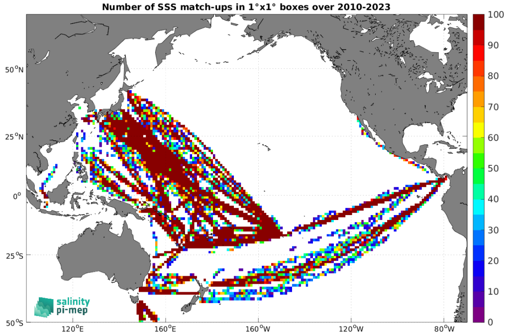
Figure 5: Number of SSS match-ups between TSG (LEGOS-DM) SSS and the SMOS SSS L2Q v331 - No FLAG (CMEMS-CATDS-CPDC) SSS product for the Pacific Ocean Pi-MEP region over 1^\circ \times 1^\circ boxes and for the full satellite product period.
