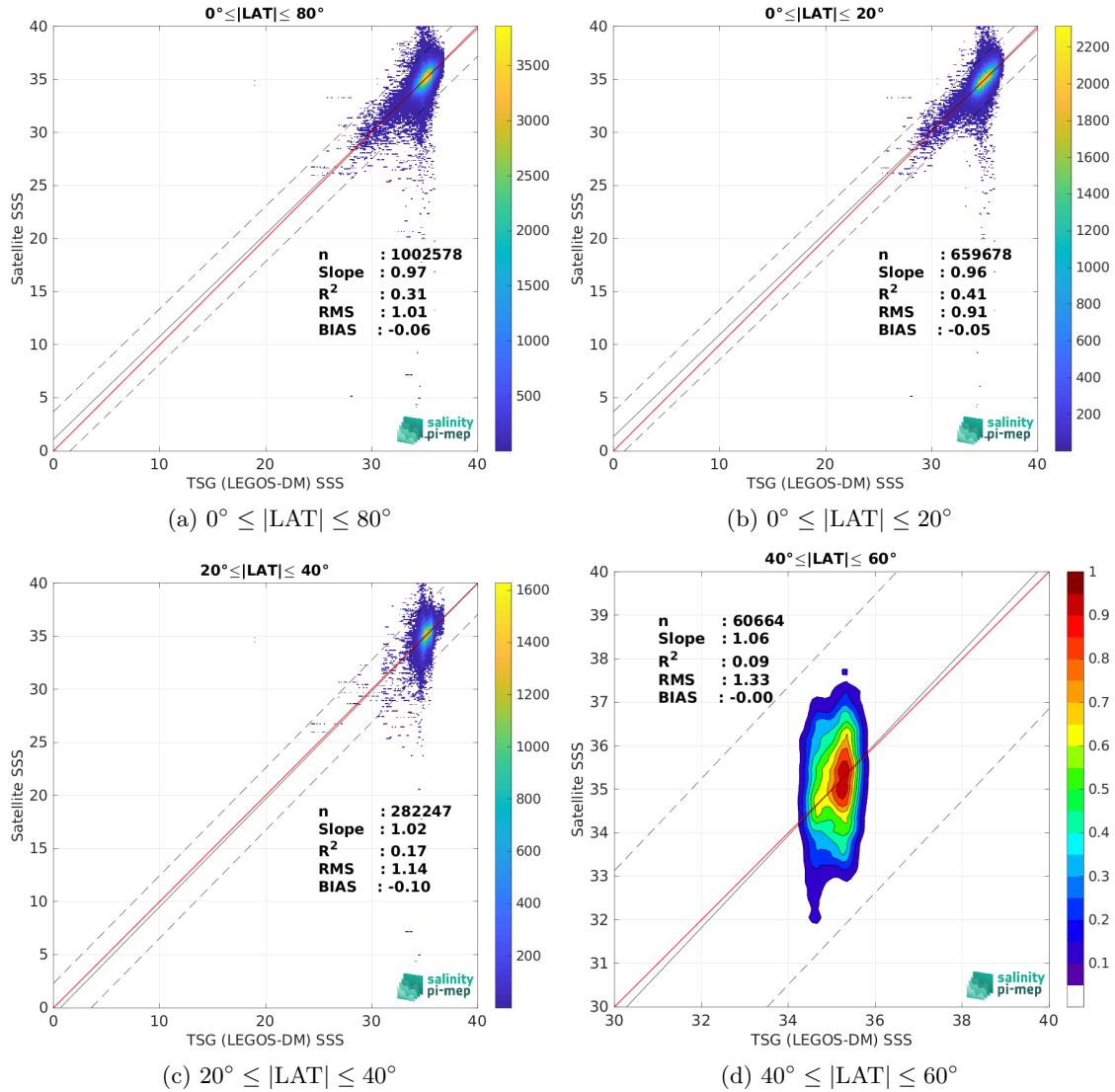
Figure 10: Contour maps of the concentration of SMOS SSS L2Q v331 - No FLAG (CMEMS-CATDS-CPDC) SSS (y-axis) versus TSG (LEGOS-DM) SSS (x-axis) at match-up pairs for different latitude bands. For each plot, the red line shows x=y . The black thin and dashed lines indicate a linear fit through the data cloud and the \pm 95\% confidence levels, respectively. The number match-up pairs n , the slope and R^2 coefficient of the linear fit, the root mean square (RMS) and the mean bias between satellite and in situ data are indicated for each latitude band in each plots.
