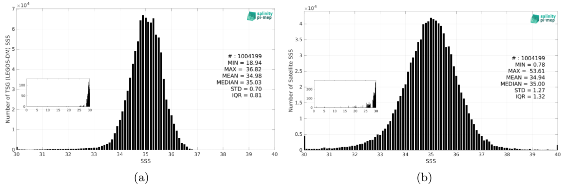
Figure 3: Histograms of SSS from TSG (LEGOS-DM) (a) and SMOS SSS L2Q v331 - No FLAG (CMEMS-CATDS-CPDC) (b) considering all match-up pairs per bins of 0.1 over the Pacific Ocean Pi-MEP region and for the full satellite product period.
