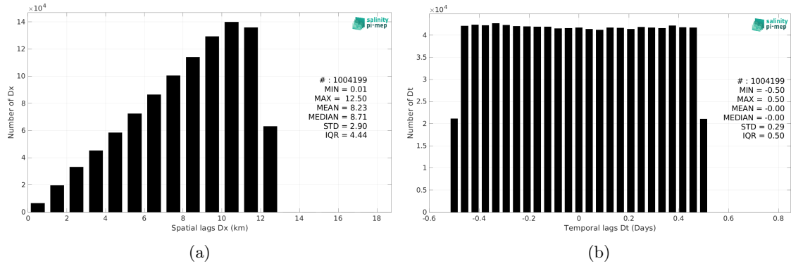
Figure 6: Histograms of the spatial (a) and temporal (b) lags between the location/time of the TSG (LEGOS-DM) measurement and the date of the corresponding SMOS SSS L2Q v331 - No FLAG (CMEMS-CATDS-CPDC) SSS pixel.
