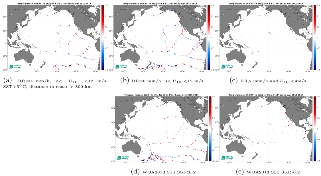
Figure 14: Temporal mean gridded over spatial boxes of size 1^\circ \times 1^\circ of \Delta SSS (SMOS SSS L2Q v331 - No FLAG (CMEMS-CATDS-CPDC) - TSG (GOSUD-Sailing-ship)) for 5 different sub-datasets corresponding to:RR=0 mm/h, 3 < U_{10} < 12 m/s, SST >5^\circ C, distance to coast > 800 km (a), RR=0 mm/h, 3 < U_{10} < 12 m/s (b), RR >1 mm/h and U_{10} < 4 m/s (c), WOA2013 SSS Std <0.2 (d), WOA2013 SSS Std >0.2 (e).
