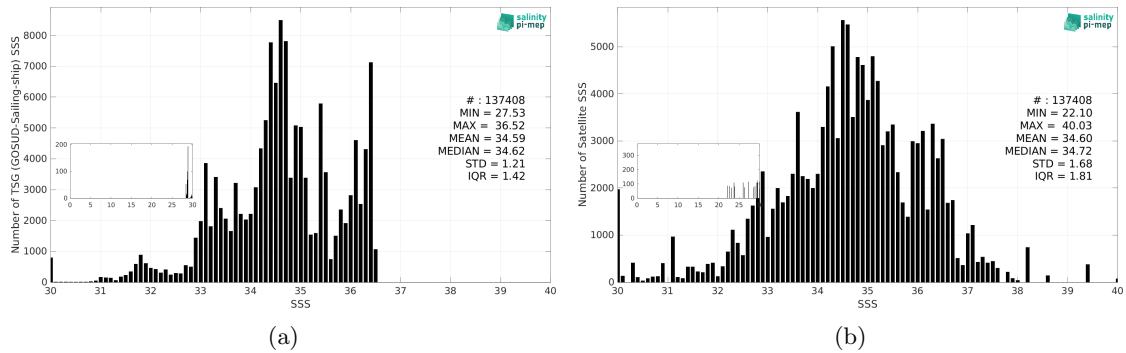
Figure 3: Histograms of SSS from TSG (GOSUD-Sailing-ship) (a) and SMOS SSS L2Q v331 - No FLAG (CMEMS-CATDS-CPDC) (b) considering all match-up pairs per bins of 0.1 over the Pacific Ocean Pi-MEP region and for the full satellite product period.
