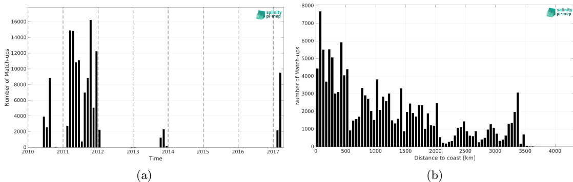
Figure 2: Number of match-ups between TSG (GOSUD-Sailing-ship) and SMOS SSS L2Q v331 - No FLAG (CMEMS-CATDS-CPDC) SSS as a function of time (a) and as function of the distance to coast (b) over the Pacific Ocean Pi-MEP region and for the full satellite product period.
